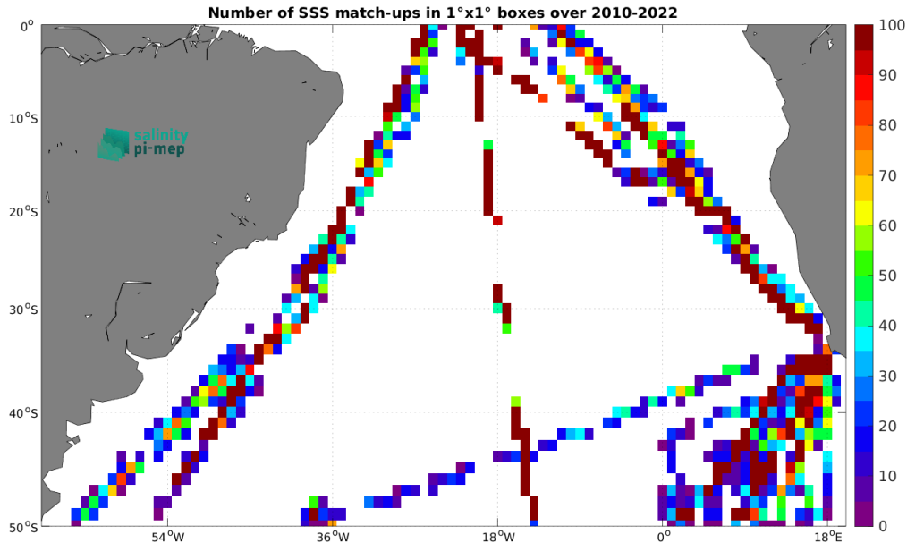
Figure 4: Number of SSS match-ups between TSG (Polarstern) SSS and the SMOS SSS L2Q v331 - With FLAG (CMEMS-CATDS-CPDC) SSS product for the South Atlantic Ocean Pi-MEP region over 1^\circ \times 1^\circ boxes and for the full satellite product period.
