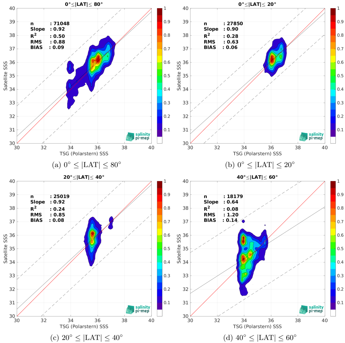
Figure 9: Contour maps of the concentration of SMOS SSS L2Q v331 - With FLAG (CMEMS-CATDS-CPDC) SSS (y-axis) versus TSG (Polarstern) SSS (x-axis) at match-up pairs for different latitude bands. For each plot, the red line shows x=y . The black thin and dashed lines indicate a linear fit through the data cloud and the \pm 95\% confidence levels, respectively. The number match-up pairs n , the slope and R^2 coefficient of the linear fit, the root mean square (RMS) and the mean bias between satellite and in situ data are indicated for each latitude band in each plots.
