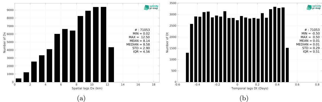
Figure 5: Histograms of the spatial (a) and temporal (b) lags between the location/time of the TSG (Polarstern) measurement and the date of the corresponding SMOS SSS L2Q v331 - With FLAG (CMEMS-CATDS-CPDC) SSS pixel.
