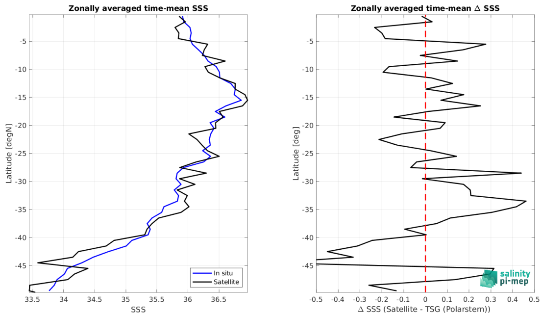
Figure 8: Left panel: Zonal mean SSS from SMOS SSS L2Q v331 - With FLAG (CMEMS-CATDS-CPDC) satellite product (black) and from TSG (Polarstern) (blue). Right panel: Zonal mean of \Delta SSS (Satellite - TSG (Polarstern)) for all the collected Pi-MEP match-up pairs estimated over the full satellite product period.
