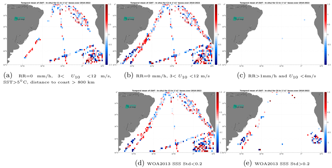
Figure 12: Temporal mean gridded over spatial boxes of size 1^\circ \times 1^\circ of \Delta SSS (SMOS SSS L2Q v331 - With FLAG (CMEMS-CATDS-CPDC) - TSG (Polarstern)) for 5 different subdatasets corresponding to:RR=0 mm/h, 3 < U_{10} < 12 m/s, SST >5^\circ\text{C} , distance to coast > 800 km (a), RR=0 mm/h, 3 < U_{10} < 12 m/s (b), RR >1 mm/h and U_{10} < 4 m/s (c), WOA2013 SSS Std <0.2 (d), WOA2013 SSS Std >0.2 (e).
