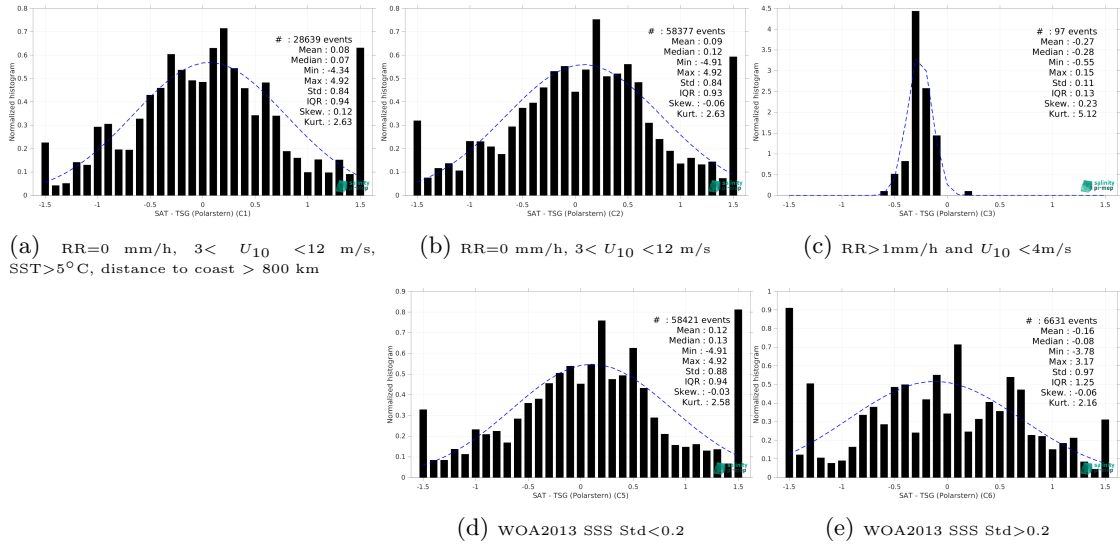
Figure 13: Normalized histogram of \Delta SSS (SMOS SSS L2Q v331 - With FLAG (CMEMS-CATDS-CPDC) - TSG (Polarstern)) for 5 different subdatasets corresponding to: RR=0 mm/h, 3 < U_{10} < 12 m/s, SST>5°C, distance to coast > 800 km (a), RR=0 mm/h, 3 < U_{10} < 12 m/s (b), RR>1mm/h and U_{10} < 4 m/s (c), WOA2013 SSS Std<0.2 (d), WOA2013 SSS Std>0.2 (e).
