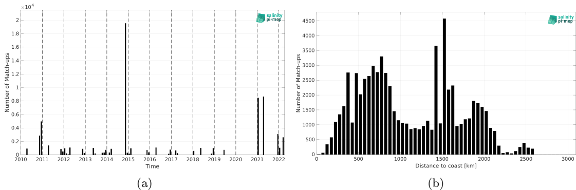
Figure 1: Number of match-ups between TSG (Polarstern) and SMOS SSS L2Q v331 - With FLAG (CMEMS-CATDS-CPDC) SSS as a function of time (a) and as function of the distance to coast (b) over the South Atlantic Ocean Pi-MEP region and for the full satellite product period.
