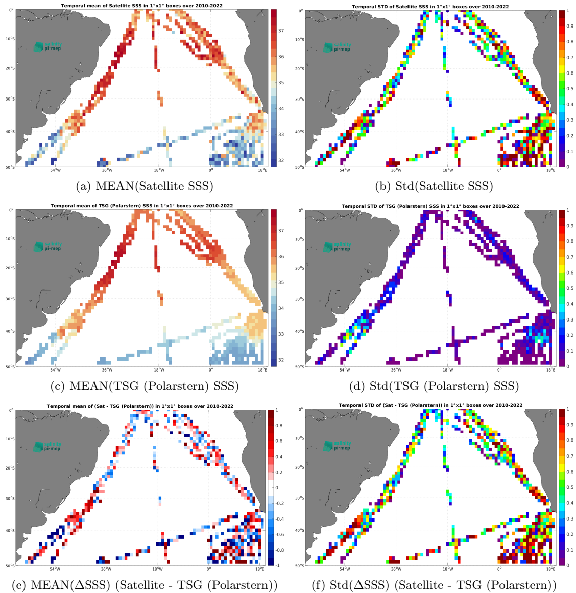
Figure 6: Temporal mean (left) and Std (right) of SSS from SMOS SSS L2Q v331 - With FLAG (CMEMS-CATDS-CPDC) (top), TSG (Polarstern) (middle), and of \Delta SSS (Satellite - TSG (Polarstern)). Only match-up pairs are used to generate these maps.
