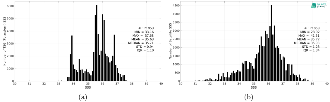
Figure 2: Histograms of SSS from TSG (Polarstern) (a) and SMOS SSS L2Q v331 - With FLAG (CMEMS-CATDS-CPDC) (b) considering all match-up pairs per bins of 0.1 over the South Atlantic Ocean Pi-MEP region and for the full satellite product period.
