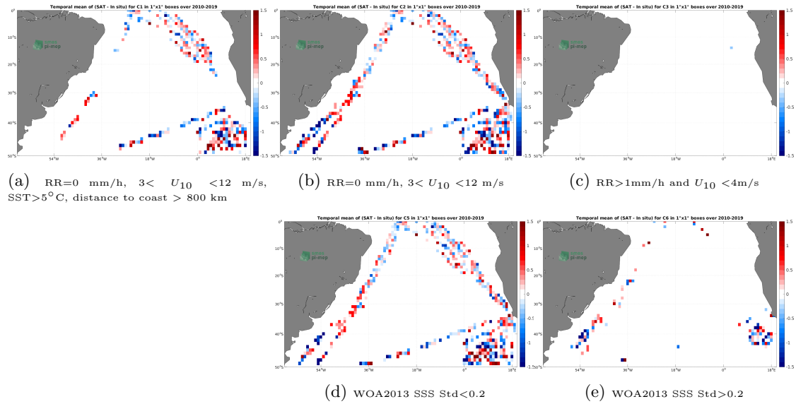
Figure 12: Temporal mean gridded over spatial boxes of size 1^\circ \times 1^\circ of \Delta\text{SSS} (SMOS SSS L2Q v331 - With FLAG (CMEMS-CATDS-CPDC) - TSG (Polarstern)) for 5 different subdatasets corresponding to:RR=0 mm/h, 3 < U_{10} < 12 m/s, SST >5^\circ\text{C} , distance to coast > 800 km (a), RR=0 mm/h, 3 < U_{10} < 12 m/s (b), RR >1 mm/h and U_{10} < 4 m/s (c), WOA2013 SSS Std <0.2 (d), WOA2013 SSS Std >0.2 (e).
