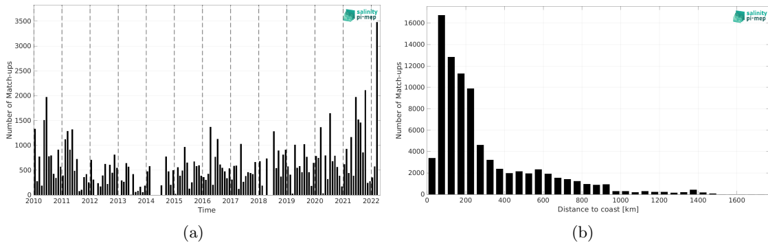
Figure 2: Number of match-ups between TSG (LEGOS-DM) and SMOS SSS L2Q v331 - With FLAG (CMEMS-CATDS-CPDC) SSS as a function of time (a) and as function of the distance to coast (b) over the South Atlantic Ocean Pi-MEP region and for the full satellite product period.
