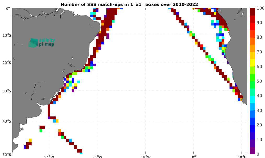
Figure 4: Number of SSS match-ups between TSG (LEGOS-DM) SSS and the SMOS SSS L2Q v331 - With FLAG (CMEMS-CATDS-CPDC) SSS product for the South Atlantic Ocean Pi-MEP region over 1^\circ \times 1^\circ boxes and for the full satellite product period.
