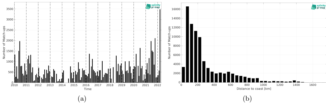
Figure 1: Number of match-ups between TSG (LEGOS-DM) and SMOS SSS L2Q v331 - With FLAG (CMEMS-CATDS-CPDC) SSS as a function of time (a) and as function of the distance to coast (b) over the South Atlantic Ocean Pi-MEP region and for the full satellite product period.
