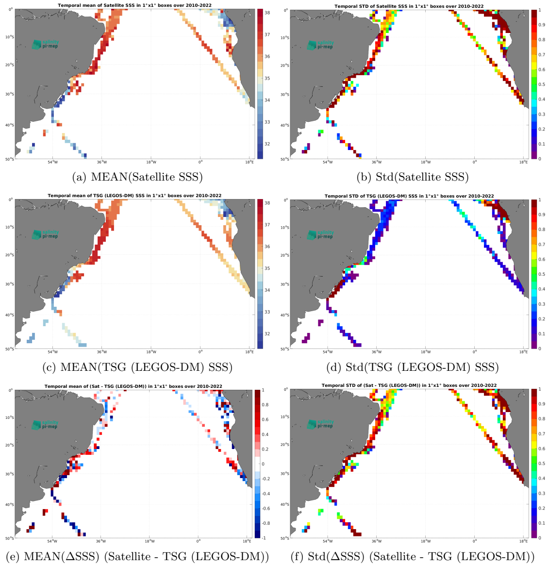
Figure 6: Temporal mean (left) and Std (right) of SSS from SMOS SSS L2Q v331 - With FLAG (CMEMS-CATDS-CPDC) (top), TSG (LEGOS-DM) (middle), and of \Delta SSS (Satellite - TSG (LEGOS-DM)). Only match-up pairs are used to generate these maps.
