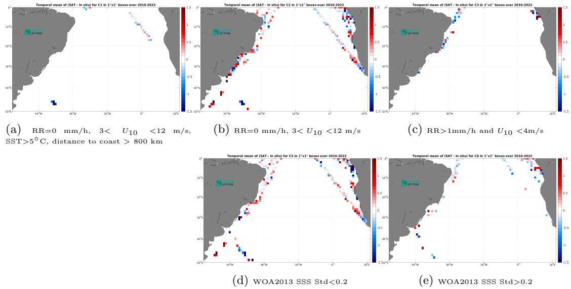
Figure 12: Temporal mean gridded over spatial boxes of size 1^\circ \times 1^\circ of \Delta\text{SSS} (SMOS SSS L2Q v331 - With FLAG (CMEMS-CATDS-CPDC) - TSG (LEGOS-DM)) for 5 different subdatasets corresponding to:RR=0 mm/h, 3 < U_{10} < 12 m/s, SST >5^\circ\text{C} , distance to coast > 800 km (a), RR=0 mm/h, 3 < U_{10} < 12 m/s (b), RR >1 mm/h and U_{10} < 4 m/s (c), WOA2013 SSS Std <0.2 (d), WOA2013 SSS Std >0.2 (e).
