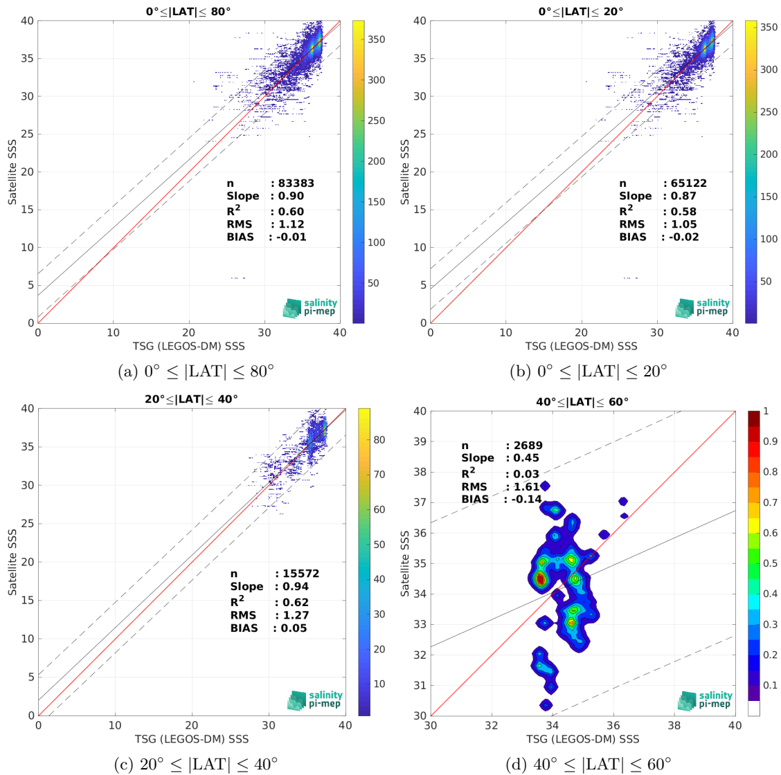
Figure 9: Contour maps of the concentration of SMOS SSS L2Q v331 - With FLAG (CMEMS-CATDS-CPDC) SSS (y-axis) versus TSG (LEGOS-DM) SSS (x-axis) at match-up pairs for different latitude bands. For each plot, the red line shows x=y . The black thin and dashed lines indicate a linear fit through the data cloud and the \pm 95\% confidence levels, respectively. The number match-up pairs n , the slope and R^2 coefficient of the linear fit, the root mean square (RMS) and the mean bias between satellite and in situ data are indicated for each latitude band in each plots.
