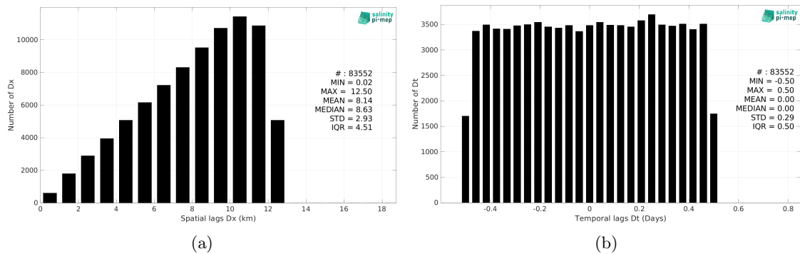
Figure 5: Histograms of the spatial (a) and temporal (b) lags between the location/time of the TSG (LEGOS-DM) measurement and the date of the corresponding SMOS SSS L2Q v331 - With FLAG (CMEMS-CATDS-CPDC) SSS pixel.
