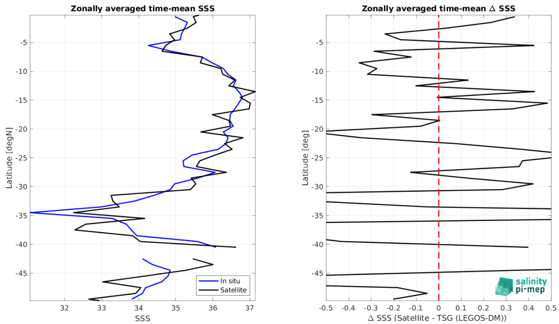
Figure 8: Left panel: Zonal mean SSS from SMOS SSS L2Q v331 - With FLAG (CMEMS-CATDS-CPDC) satellite product (black) and from TSG (LEGOS-DM) (blue). Right panel: Zonal mean of \Delta SSS (Satellite - TSG (LEGOS-DM)) for all the collected Pi-MEP match-up pairs estimated over the full satellite product period.
