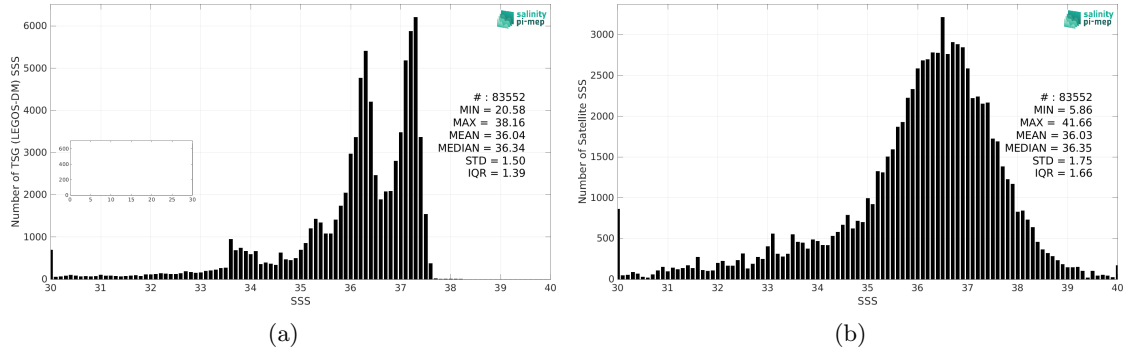
Figure 2: Histograms of SSS from TSG (LEGOS-DM) (a) and SMOS SSS L2Q v331 - With FLAG (CMEMS-CATDS-CPDC) (b) considering all match-up pairs per bins of 0.1 over the South Atlantic Ocean Pi-MEP region and for the full satellite product period.
