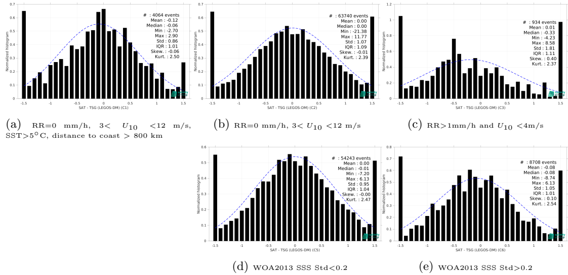
Figure 13: Normalized histogram of \Delta SSS (SMOS SSS L2Q v331 - With FLAG (CMEMS-CATDS-CPDC) - TSG (LEGOS-DM)) for 5 different subdatasets corresponding to: RR=0 mm/h, 3 < U_{10} < 12 m/s, SST>5°C, distance to coast > 800 km (a), RR=0 mm/h, 3 < U_{10} < 12 m/s (b), RR>1mm/h and U_{10} < 4 m/s (c), WOA2013 SSS Std<0.2 (d), WOA2013 SSS Std>0.2 (e).
