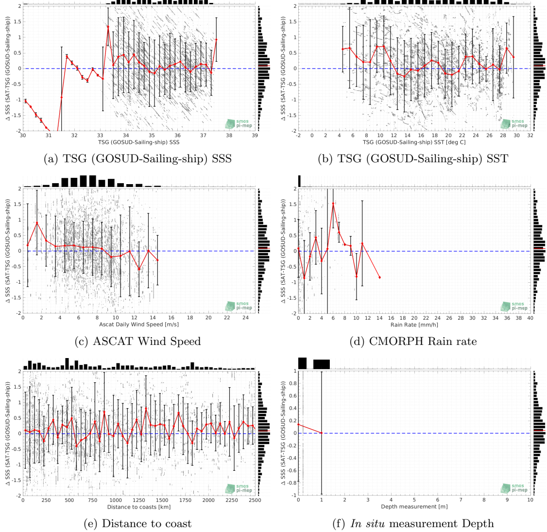
Figure 11: \Delta SSS (Satellite - TSG (GOSUD-Sailing-ship)) sorted as function of TSG (GOSUD-Sailing-ship) SSS values a), TSG (GOSUD-Sailing-ship) SST b), ASCAT Wind speed c), CMORPH rain rate d), distance to coast (e) and in situ measurement depth (f). In all plots the median and Std of \Delta SSS for each bin is indicated by the red curves and black vertical thick bars ( \pm 1 Std)
