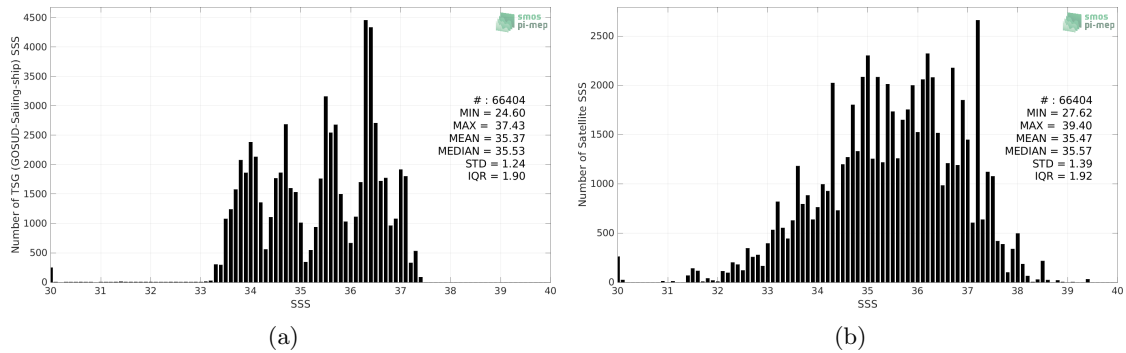
Figure 2: Histograms of SSS from TSG (GOSUD-Sailing-ship) (a) and SMOS SSS L2Q v331 - With FLAG (CMEMS-CATDS-CPDC) (b) considering all match-up pairs per bins of 0.1 over the South Atlantic Ocean Pi-MEP region and for the full satellite product period.
