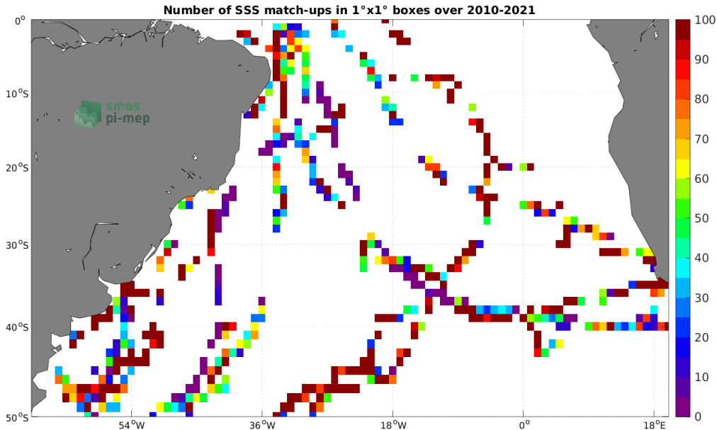
Figure 4: Number of SSS match-ups between TSG (GOSUD-Sailing-ship) SSS and the SMOS SSS L2Q v331 - With FLAG (CMEMS-CATDS-CPDC) SSS product for the South Atlantic Ocean Pi-MEP region over 1^\circ \times 1^\circ boxes and for the full satellite product period.
