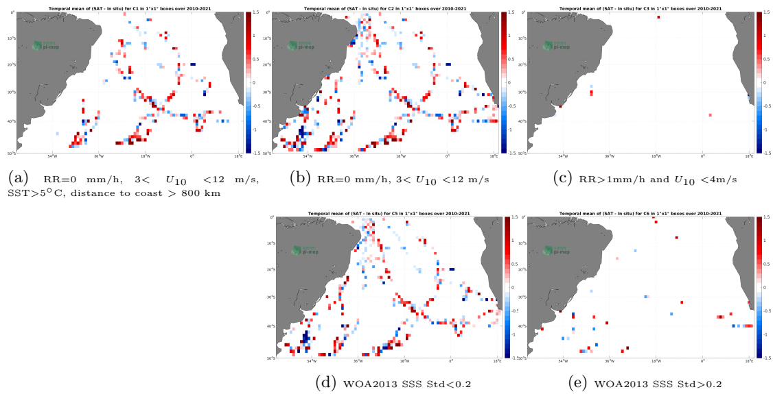
Figure 12: Temporal mean gridded over spatial boxes of size 1^\circ \times 1^\circ of \Delta\text{SSS} (SMOS SSS L2Q v331 - With FLAG (CMEMS-CATDS-CPDC) - TSG (GOSUD-Sailing-ship)) for 5 different subdatasets corresponding to:RR=0 mm/h, 3 < U_{10} < 12 m/s, SST >5^\circ\text{C} , distance to coast > 800 km (a), RR=0 mm/h, 3 < U_{10} < 12 m/s (b), RR >1 mm/h and U_{10} < 4 m/s (c), WOA2013 SSS Std <0.2 (d), WOA2013 SSS Std >0.2 (e).
