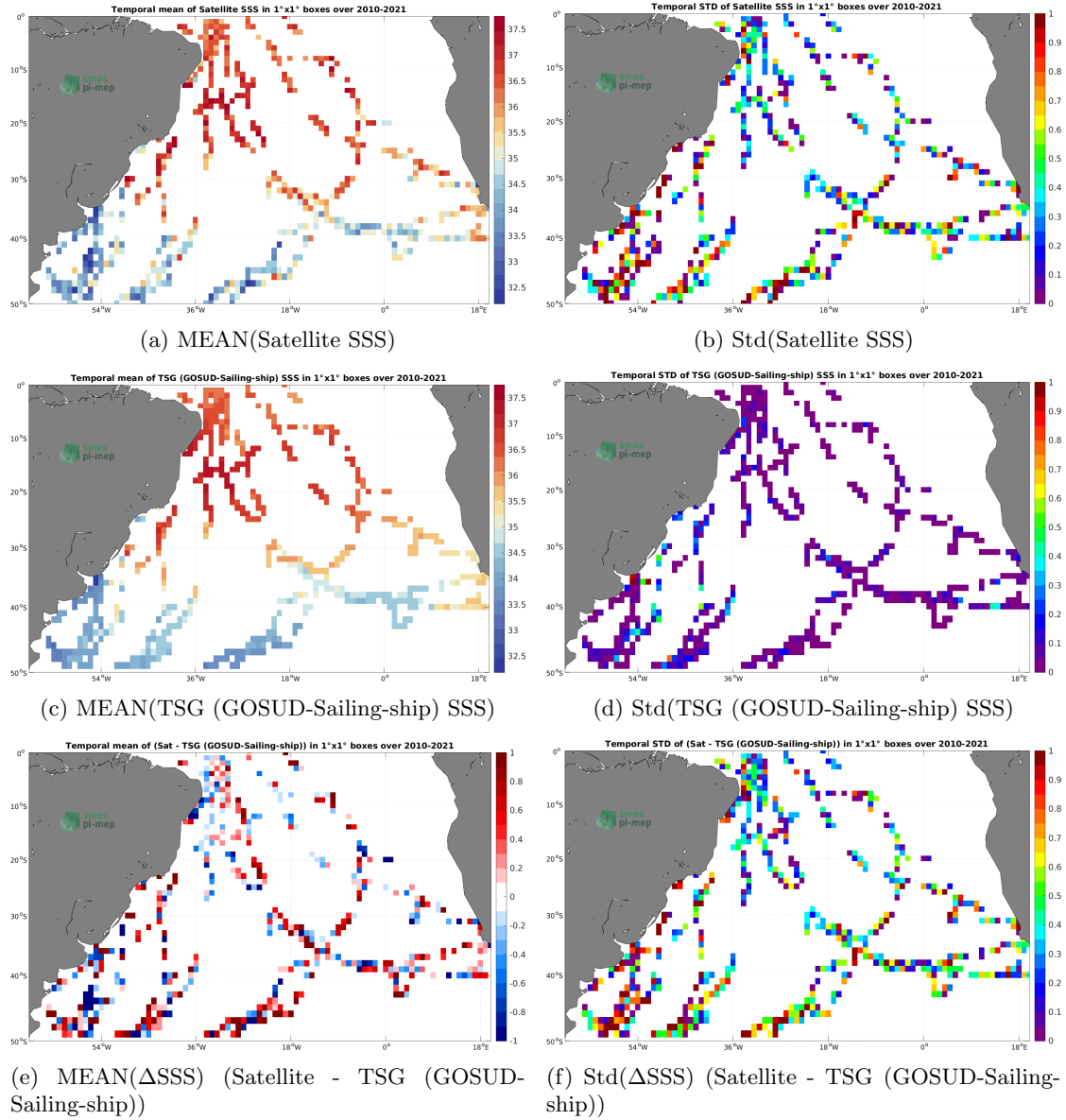
Figure 6: Temporal mean (left) and Std (right) of SSS from SMOS SSS L2Q v331 - With FLAG (CMEMS-CATDS-CPDC) (top), TSG (GOSUD-Sailing-ship) (middle), and of \Delta SSS (Satellite - TSG (GOSUD-Sailing-ship)). Only match-up pairs are used to generate these maps.
