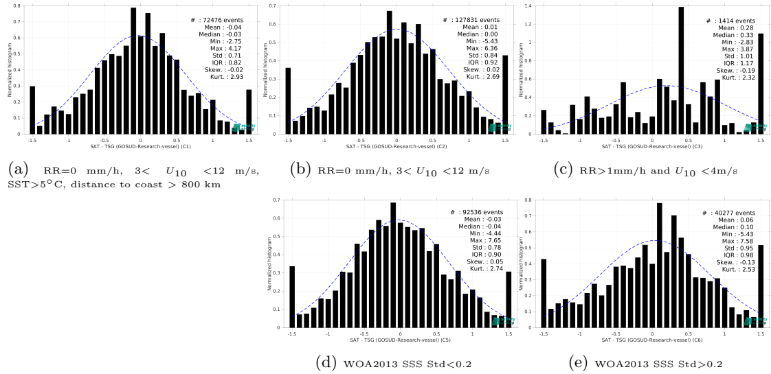
Figure 15: Normalized histogram of \Delta SSS (SMOS SSS L2Q v331 - With FLAG (CMEMS-CATDS-CPDC) - TSG (GOSUD-Research-vessel)) for 5 different subdatasets corresponding to: RR=0 mm/h, 3 < U_{10} < 12 m/s, SST>5°C, distance to coast > 800 km (a), RR=0 mm/h, 3 < U_{10} < 12 m/s (b), RR>1mm/h and U_{10} < 4 m/s (c), WOA2013 SSS Std<0.2 (d), WOA2013 SSS Std>0.2 (e).
