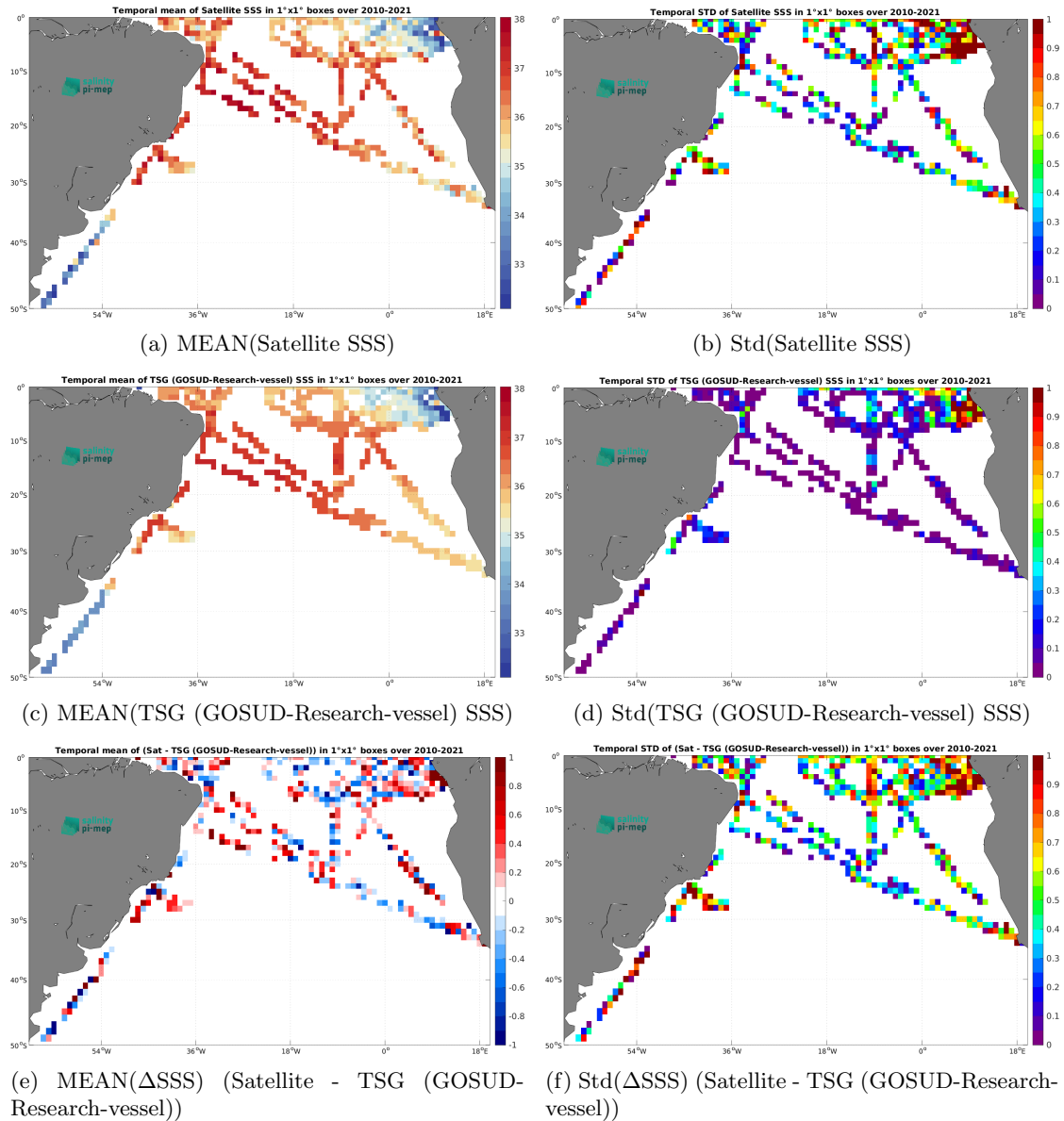
Figure 7: Temporal mean (left) and Std (right) of SSS from SMOS SSS L2Q v331 - With FLAG (CMEMS-CATDS-CPDC) (top), TSG (GOSUD-Research-vessel) (middle), and of \Delta SSS (Satellite - TSG (GOSUD-Research-vessel)). Only match-up pairs are used to generate these maps.
