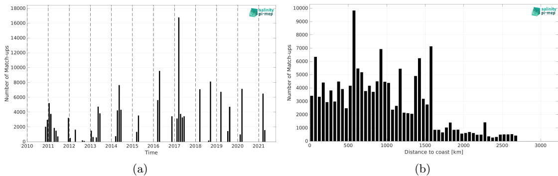
Figure 2: Number of match-ups between TSG (GOSUD-Research-vessel) and SMOS SSS L2Q v331 - With FLAG (CMEMS-CATDS-CPDC) SSS as a function of time (a) and as function of the distance to coast (b) over the South Atlantic Ocean Pi-MEP region and for the full satellite product period.
