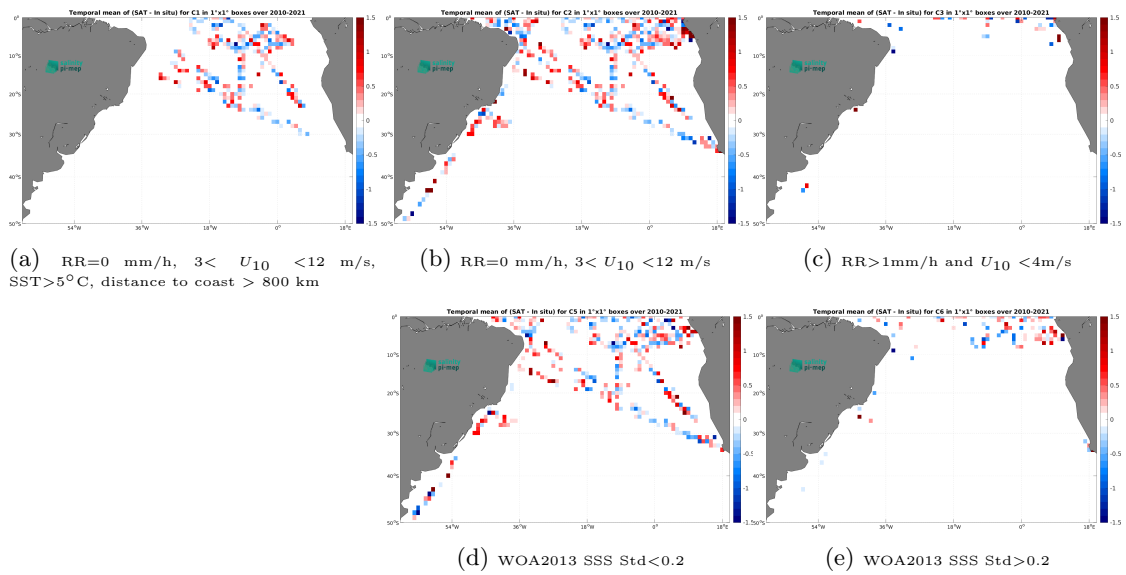
Figure 14: Temporal mean gridded over spatial boxes of size 1^\circ \times 1^\circ of \Delta SSS (SMOS SSS L2Q v331 - With FLAG (CMEMS-CATDS-CPDC) - TSG (GOSUD-Research-vessel)) for 5 different subdatasets corresponding to:RR=0 mm/h, 3 < U_{10} < 12 m/s, SST>5°C, distance to coast > 800 km (a), RR=0 mm/h, 3 < U_{10} < 12 m/s (b), RR>1mm/h and U_{10} < 4 m/s (c), WOA2013 SSS Std<0.2 (d), WOA2013 SSS Std>0.2 (e).
