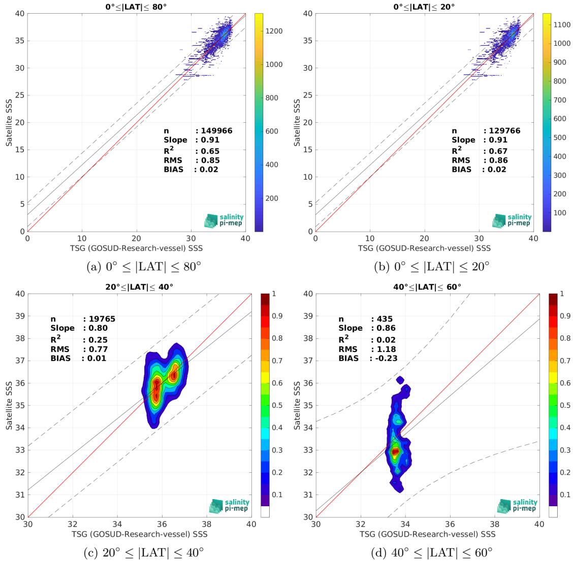
Figure 10: Contour maps of the concentration of SMOS SSS L2Q v331 - With FLAG (CMEMS-CATDS-CPDC) SSS (y-axis) versus TSG (GOSUD-Research-vessel) SSS (x-axis) at match-up pairs for different latitude bands. For each plot, the red line shows x=y . The black thin and dashed lines indicate a linear fit through the data cloud and the \pm 95\% confidence levels, respectively. The number match-up pairs n , the slope and R^2 coefficient of the linear fit, the root mean square (RMS) and the mean bias between satellite and in situ data are indicated for each latitude band in each plots.
