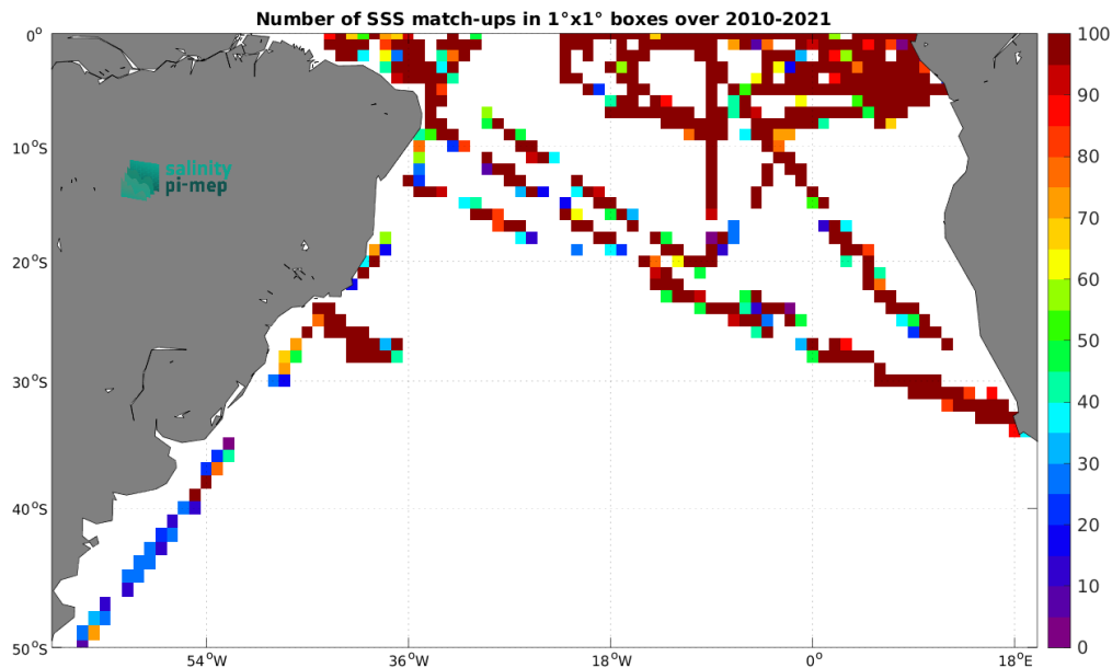
Figure 5: Number of SSS match-ups between TSG (GOSUD-Research-vessel) SSS and the SMOS SSS L2Q v331 - With FLAG (CMEMS-CATDS-CPDC) SSS product for the South Atlantic Ocean Pi-MEP region over 1^\circ \times 1^\circ boxes and for the full satellite product period.
