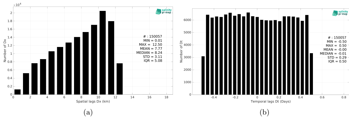
Figure 6: Histograms of the spatial (a) and temporal (b) lags between the location/time of the TSG (GOSUD-Research-vessel) measurement and the date of the corresponding SMOS SSS L2Q v331 - With FLAG (CMEMS-CATDS-CPDC) SSS pixel.
