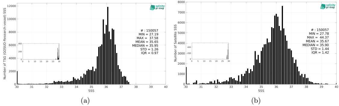
Figure 3: Histograms of SSS from TSG (GOSUD-Research-vessel) (a) and SMOS SSS L2Q v331 - With FLAG (CMEMS-CATDS-CPDC) (b) considering all match-up pairs per bins of 0.1 over the South Atlantic Ocean Pi-MEP region and for the full satellite product period.
