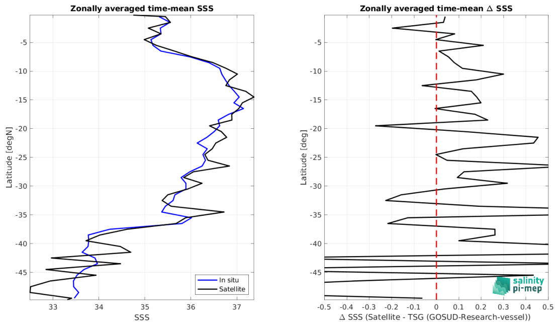
Figure 9: Left panel: Zonal mean SSS from SMOS SSS L2Q v331 - With FLAG (CMEMS-CATDS-CPDC) satellite product (black) and from TSG (GOSUD-Research-vessel) (blue). Right panel: Zonal mean of \Delta SSS (Satellite - TSG (GOSUD-Research-vessel)) for all the collected Pi-MEP match-up pairs estimated over the full satellite product period.
