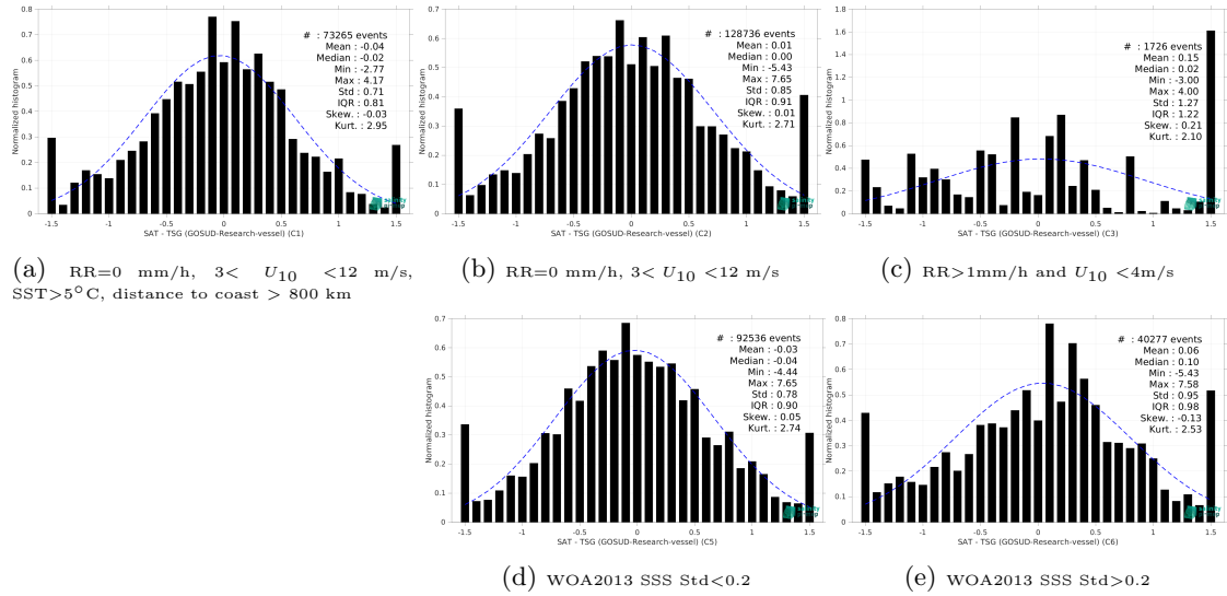
Figure 13: Normalized histogram of \Delta\text{SSS} (SMOS SSS L2Q v331 - With FLAG (CMEMS-CATDS-CPDC) - TSG (GOSUD-Research-vessel)) for 5 different subdatasets corresponding to: RR=0 mm/h, 3 < U_{10} < 12 m/s, SST > 5^\circ\text{C} , distance to coast > 800 km (a), RR=0 mm/h, 3 < U_{10} < 12 m/s (b), RR > 1 mm/h and U_{10} < 4 m/s (c), WOA2013 SSS Std < 0.2 (d), WOA2013 SSS Std > 0.2 (e).
