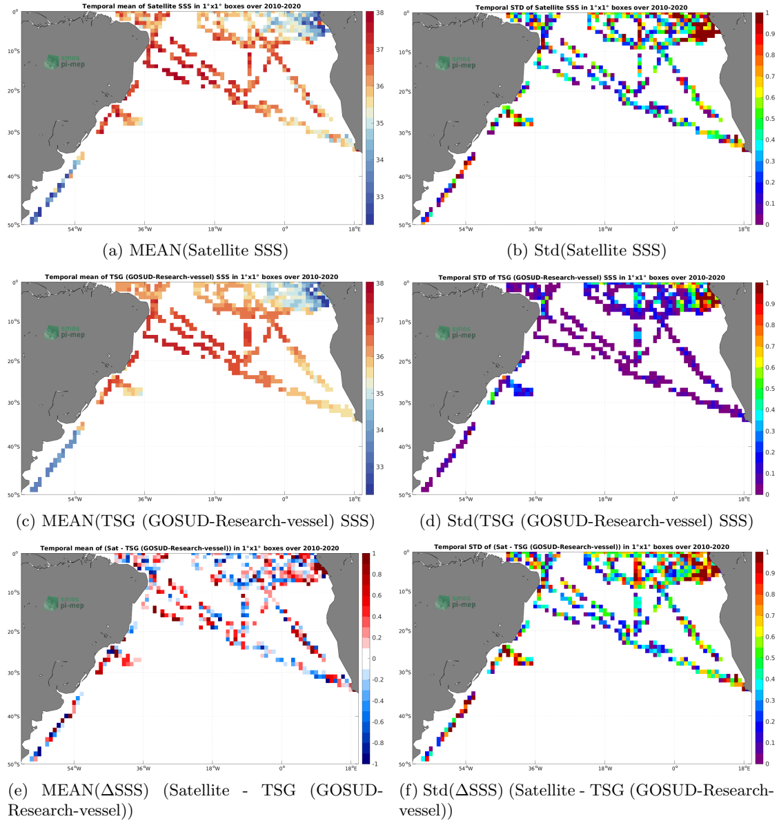
Figure 6: Temporal mean (left) and Std (right) of SSS from SMOS SSS L2Q v331 - With FLAG (CMEMS-CATDS-CPDC) (top), TSG (GOSUD-Research-vessel) (middle), and of \Delta SSS (Satellite - TSG (GOSUD-Research-vessel)). Only match-up pairs are used to generate these maps.
