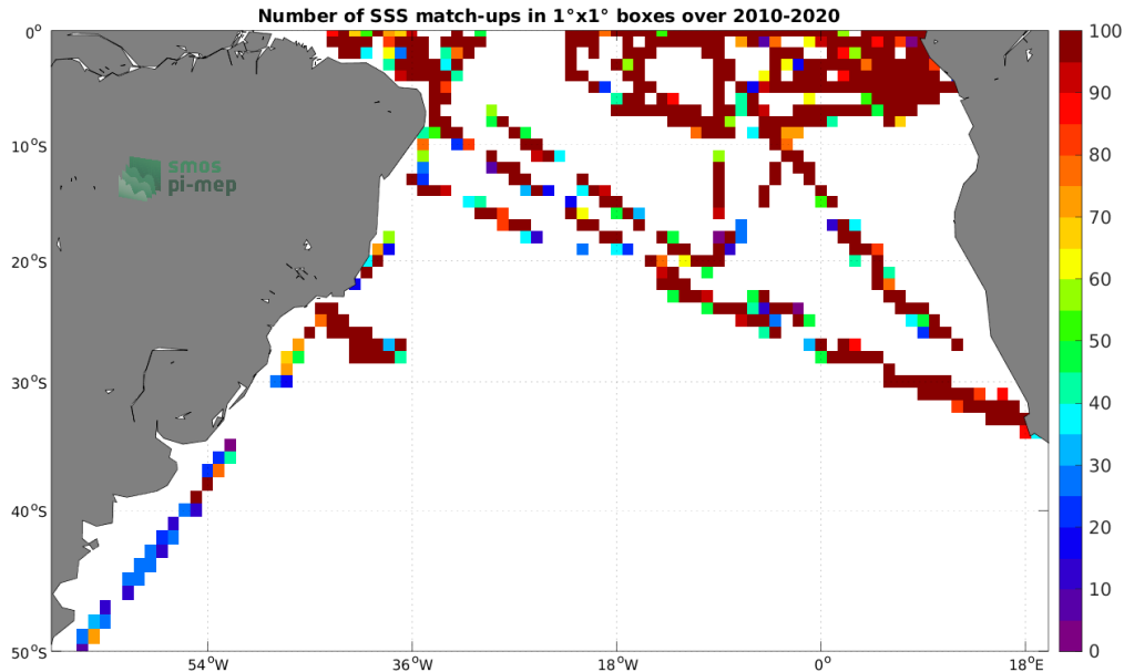
Figure 4: Number of SSS match-ups between TSG (GOSUD-Research-vessel) SSS and the SMOS SSS L2Q v331 - With FLAG (CMEMS-CATDS-CPDC) SSS product for the South Atlantic Ocean Pi-MEP region over 1^\circ \times 1^\circ boxes and for the full satellite product period.
