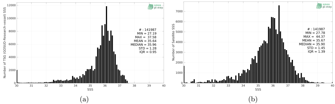
Figure 2: Histograms of SSS from TSG (GOSUD-Research-vessel) (a) and SMOS SSS L2Q v331 - With FLAG (CMEMS-CATDS-CPDC) (b) considering all match-up pairs per bins of 0.1 over the South Atlantic Ocean Pi-MEP region and for the full satellite product period.
