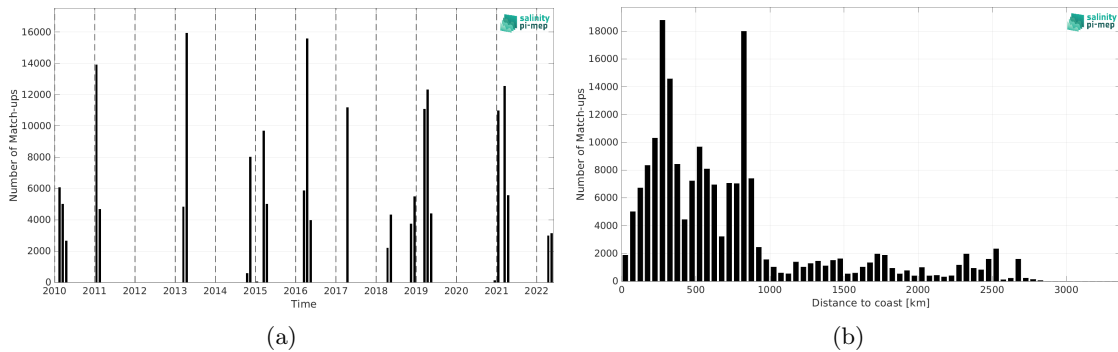
Figure 2: Number of match-ups between TSG (CSIC-UTM) and SMOS SSS L2Q v331 - With FLAG (CMEMS-CATDS-CPDC) SSS as a function of time (a) and as function of the distance to coast (b) over the South Atlantic Ocean Pi-MEP region and for the full satellite product period.
