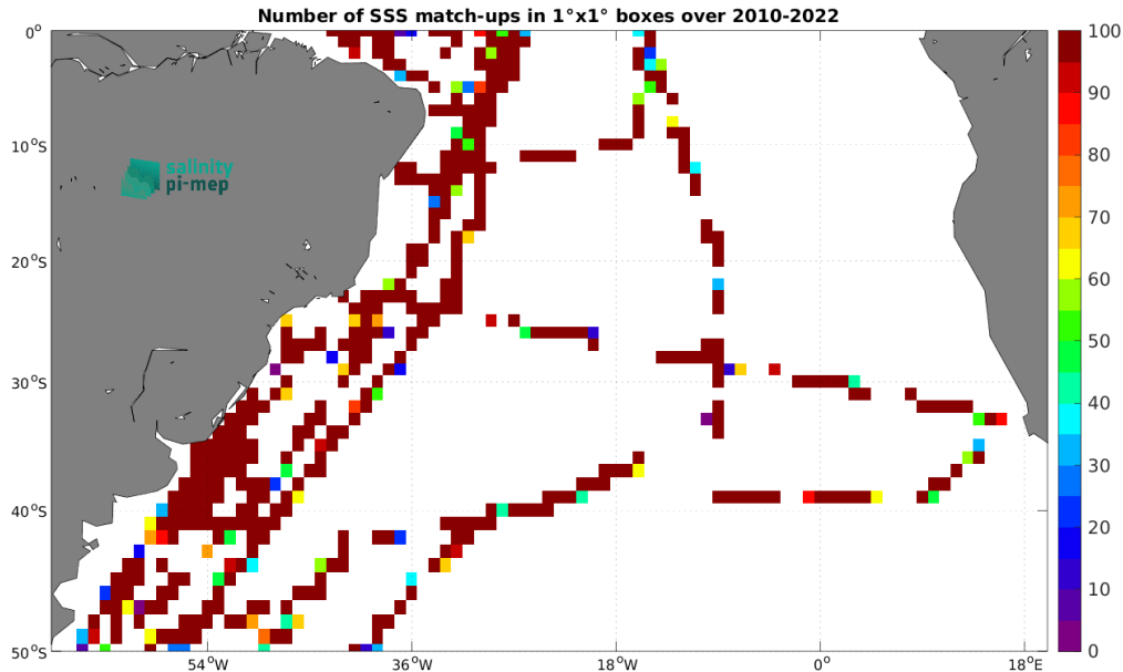
Figure 5: Number of SSS match-ups between TSG (CSIC-UTM) SSS and the SMOS SSS L2Q v331 - With FLAG (CMEMS-CATDS-CPDC) SSS product for the South Atlantic Ocean Pi-MEP region over 1^{\circ} \times 1^{\circ} boxes and for the full satellite product period.
