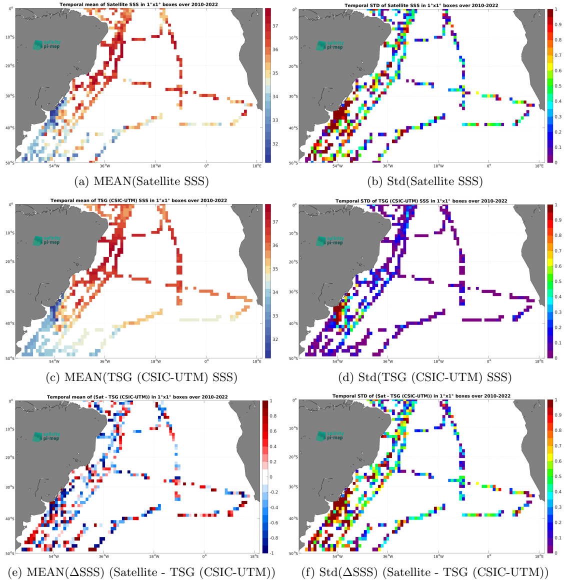
Figure 7: Temporal mean (left) and Std (right) of SSS from SMOS SSS L2Q v331 - With FLAG (CMEMS-CATDS-CPDC) (top), TSG (CSIC-UTM) (middle), and of \Delta SSS (Satellite - TSG (CSIC-UTM)). Only match-up pairs are used to generate these maps.
