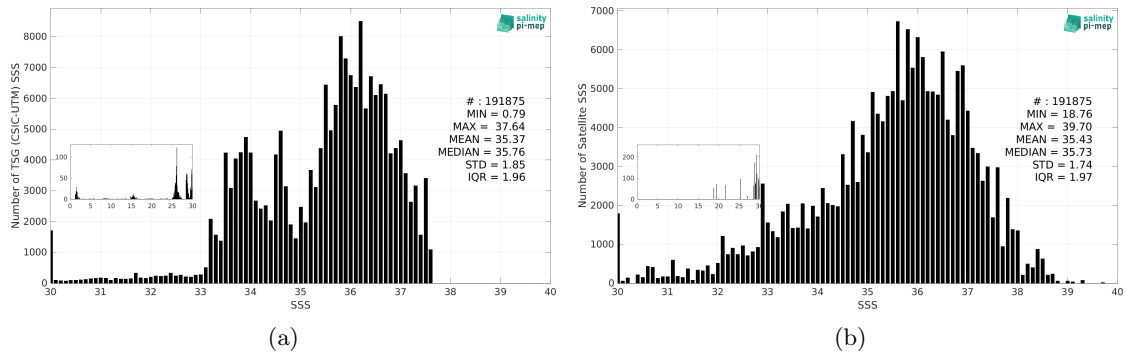
Figure 3: Histograms of SSS from TSG (CSIC-UTM) (a) and SMOS SSS L2Q v331 - With FLAG (CMEMS-CATDS-CPDC) (b) considering all match-up pairs per bins of 0.1 over the South Atlantic Ocean Pi-MEP region and for the full satellite product period.
