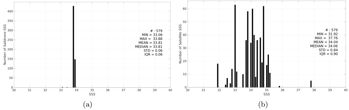
Figure 3: Histograms of SSS from Sairdrone (a) and SMOS SSS L2Q v331 - With FLAG (CMEMS-CATDS-CPDC) (b) considering all match-up pairs per bins of 0.1 over the South Atlantic Ocean Pi-MEP region and for the full satellite product period.
