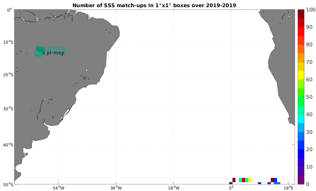
Figure 5: Number of SSS match-ups between Saildrone SSS and the SMOS SSS L2Q v331 - With FLAG (CMEMS-CATDS-CPDC) SSS product for the South Atlantic Ocean Pi-MEP region over 1^\circ \times 1^\circ boxes and for the full satellite product period.
