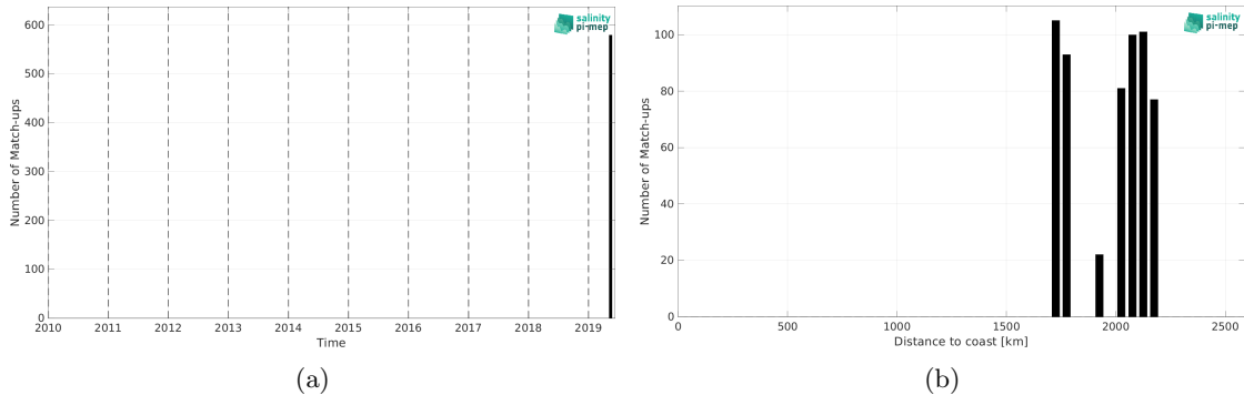
Figure 2: Number of match-ups between Saildrone and SMOS SSS L2Q v331 - With FLAG (CMEMS-CATDS-CPDC) SSS as a function of time (a) and as function of the distance to coast (b) over the South Atlantic Ocean Pi-MEP region and for the full satellite product period.
