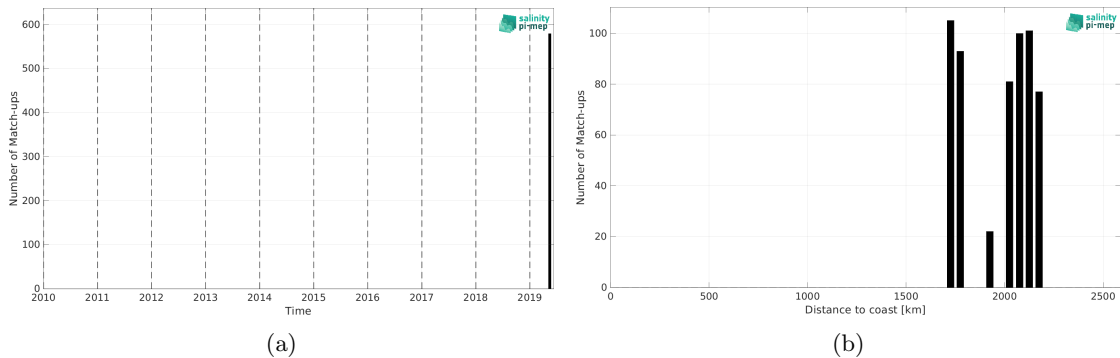
Figure 1: Number of match-ups between Saildrone and SMOS SSS L2Q v331 - With FLAG (CMEMS-CATDS-CPDC) SSS as a function of time (a) and as function of the distance to coast (b) over the South Atlantic Ocean Pi-MEP region and for the full satellite product period.
