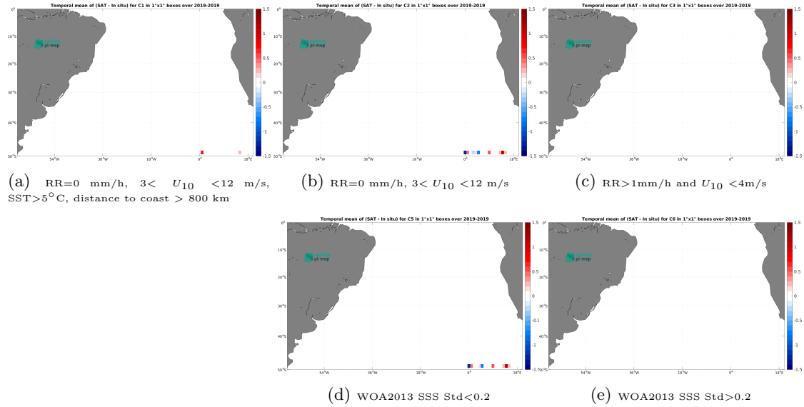
Figure 12: Temporal mean gridded over spatial boxes of size 1^{\circ}\times 1^{\circ} of \Delta\text{SSS} (SMOS SSS L2Q v331 - With FLAG (CMEMS-CATDS-CPDC) - Saildrone) for 5 different subdatasets corresponding to: RR=0 mm/h, 3 < U_{10} < 12 m/s, SST > 5^{\circ}\text{C} , distance to coast > 800 km (a), RR=0 mm/h, 3 < U_{10} < 12 m/s (b), RR > 1 mm/h and U_{10} < 4 m/s (c), WOA2013 SSS Std < 0.2 (d), WOA2013 SSS Std > 0.2 (e).
