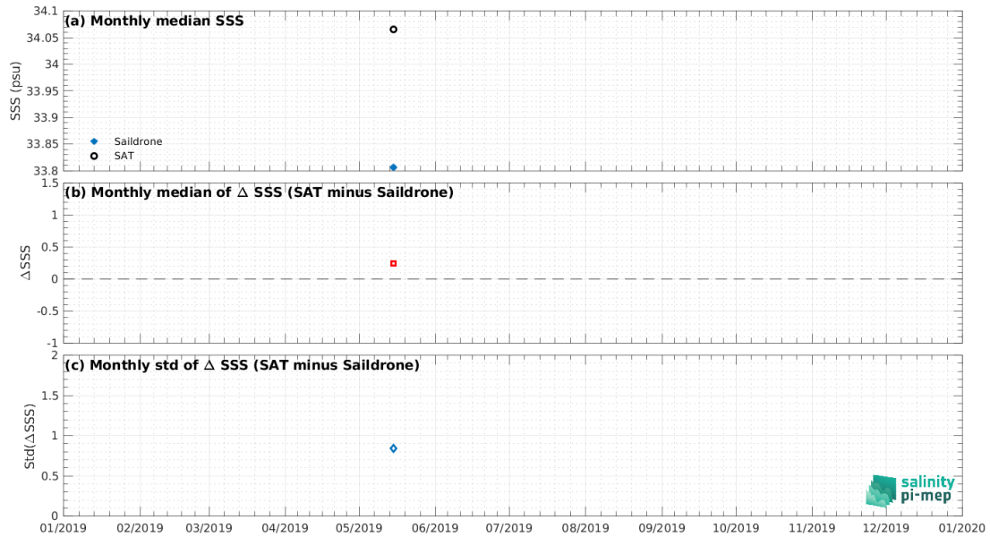
Figure 7: Time series of the monthly median SSS (top), median of \Delta SSS (Satellite - SAILDRONE) and Std of \Delta SSS (Satellite - SAILDRONE) over the South Atlantic Ocean Pi-MEP region considering all match-ups collected by the Pi-MEP.
