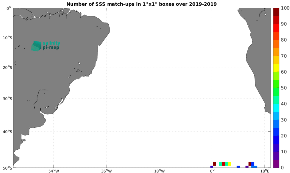
Figure 4: Number of SSS match-ups between Saildrone SSS and the SMOS SSS L2Q v331 - With FLAG (CMEMS-CATDS-CPDC) SSS product for the South Atlantic Ocean Pi-MEP region over 1^\circ \times 1^\circ boxes and for the full satellite product period.
