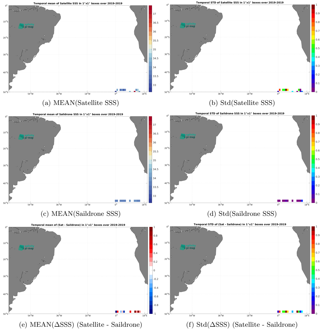
Figure 6: Temporal mean (left) and Std (right) of SSS from SMOS SSS L2Q v331 - With FLAG (CMEMS-CATDS-CPDC) (top), Saildrone (middle), and of \Delta SSS (Satellite - Saildrone). Only match-up pairs are used to generate these maps.
