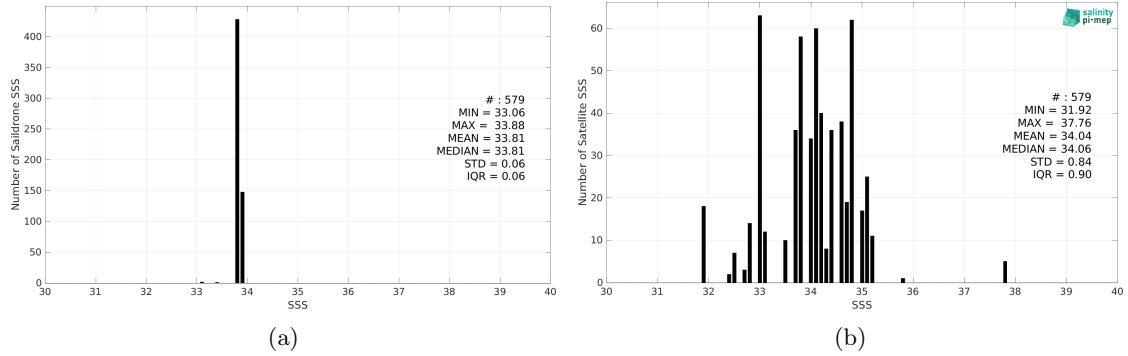
Figure 2: Histograms of SSS from Saildrone (a) and SMOS SSS L2Q v331 - With FLAG (CMEMS-CATDS-CPDC) (b) considering all match-up pairs per bins of 0.1 over the South Atlantic Ocean Pi-MEP region and for the full satellite product period.
