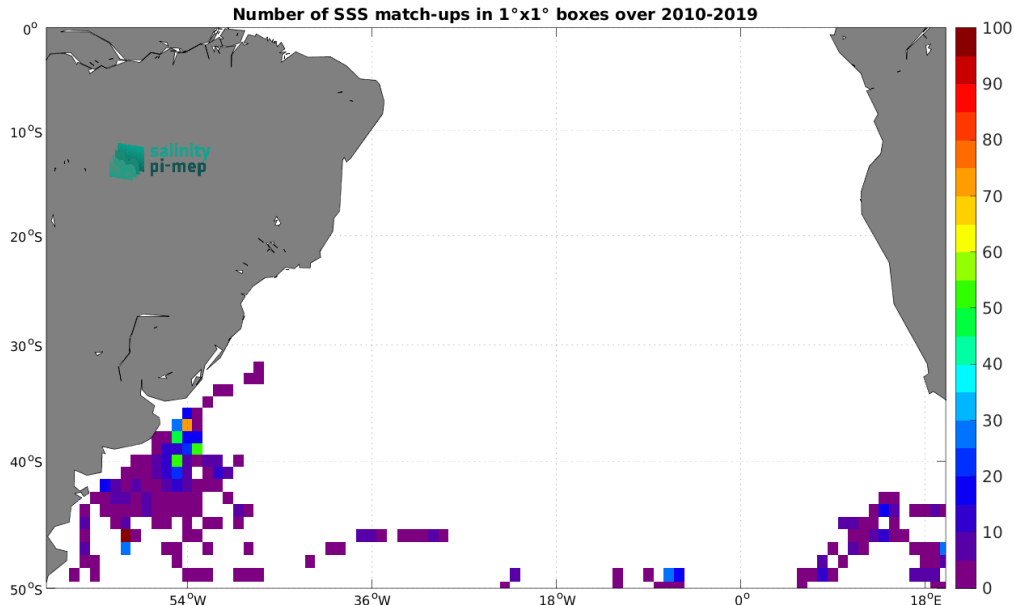
Figure 4: Number of SSS match-ups between Marine mammals SSS and the SMOS SSS L2Q v331 - With FLAG (CMEMS-CATDS-CPDC) SSS product for the South Atlantic Ocean Pi-MEP region over 1^\circ \times 1^\circ boxes and for the full satellite product period.
