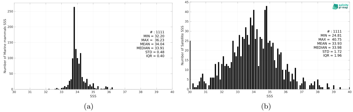
Figure 2: Histograms of SSS from Marine mammals (a) and SMOS SSS L2Q v331 - With FLAG (CMEMS-CATDS-CPDC) (b) considering all match-up pairs per bins of 0.1 over the South Atlantic Ocean Pi-MEP region and for the full satellite product period.
