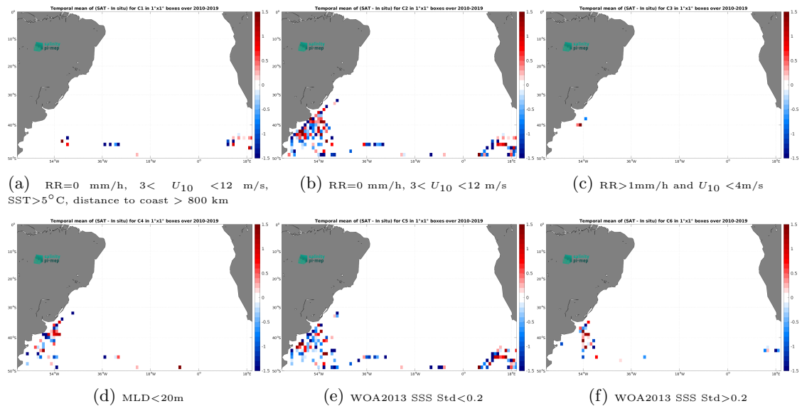
Figure 12: Temporal mean gridded over spatial boxes of size 1^{\circ}\times 1^{\circ} of \Delta\text{SSS} (SMOS SSS L2Q v331 - With FLAG (CMEMS-CATDS-CPDC) - Marine mammals) for 6 different subdatasets corresponding to:RR=0 mm/h, 3 < U_{10} < 12 m/s, SST >5^{\circ}\text{C} , distance to coast > 800 km (a), RR=0 mm/h, 3 < U_{10} < 12 m/s (b), RR >1 mm/h and U_{10} < 4 m/s (c),MLD <20 m (d),WOA2013 SSS Std <0.2 (e),WOA2013 SSS Std >0.2 (f).
