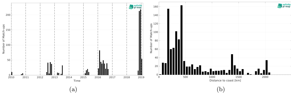
Figure 1: Number of match-ups between Marine mammals and SMOS SSS L2Q v331 - With FLAG (CMEMS-CATDS-CPDC) SSS as a function of time (a) and as function of the distance to coast (b) over the South Atlantic Ocean Pi-MEP region and for the full satellite product period.
