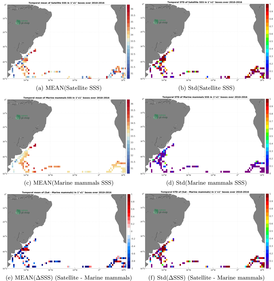
Figure 6: Temporal mean (left) and Std (right) of SSS from SMOS SSS L2Q v331 - With FLAG (CMEMS-CATDS-CPDC) (top), Marine mammals (middle), and of \Delta SSS (Satellite - Marine mammals). Only match-up pairs are used to generate these maps.
