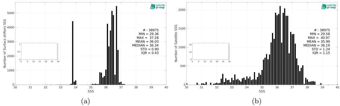
Figure 3: Histograms of SSS from Surface drifters (a) and SMOS SSS L2Q v331 - With FLAG (CMEMS-CATDS-CPDC) (b) considering all match-up pairs per bins of 0.1 over the South Atlantic Ocean Pi-MEP region and for the full satellite product period.
