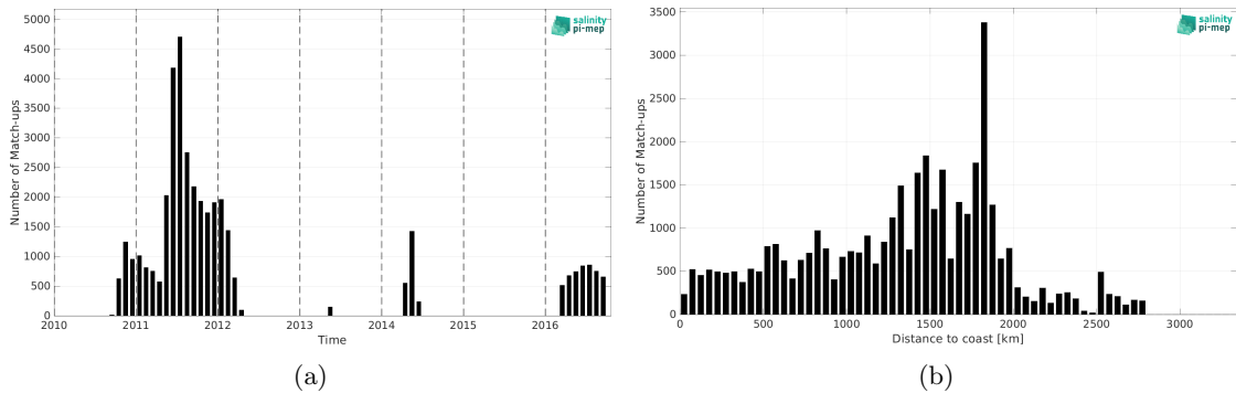
Figure 2: Number of match-ups between Surface drifters and SMOS SSS L2Q v331 - With FLAG (CMEMS-CATDS-CPDC) SSS as a function of time (a) and as function of the distance to coast (b) over the South Atlantic Ocean Pi-MEP region and for the full satellite product period.
