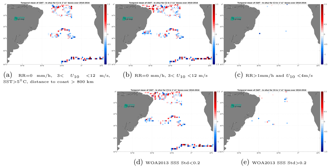
Figure 13: Temporal mean gridded over spatial boxes of size 1^\circ \times 1^\circ of \Delta\text{SSS} (SMOS SSS L2Q v331 - With FLAG (CMEMS-CATDS-CPDC) - Surface drifters) for 5 different subdatasets corresponding to:RR=0 mm/h, 3 < U_{10} < 12 m/s, SST >5^\circ\text{C} , distance to coast > 800 km (a), RR=0 mm/h, 3 < U_{10} < 12 m/s (b), RR >1 mm/h and U_{10} < 4 m/s (c), WOA2013 SSS Std <0.2 (d), WOA2013 SSS Std >0.2 (e).
