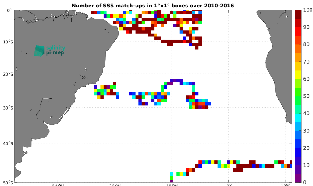
Figure 4: Number of SSS match-ups between Surface drifters SSS and the SMOS SSS L2Q v331 - With FLAG (CMEMS-CATDS-CPDC) SSS product for the South Atlantic Ocean Pi-MEP region over 1^\circ \times 1^\circ boxes and for the full satellite product period.
