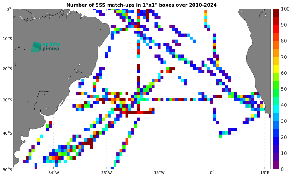
Figure 5: Number of SSS match-ups between TSG (SAMOS) SSS and the SMOS SSS L2Q v331 - No FLAG (CMEMS-CATDS-CPDC) SSS product for the South Atlantic Ocean Pi-MEP region over 1^\circ \times 1^\circ boxes and for the full satellite product period.
