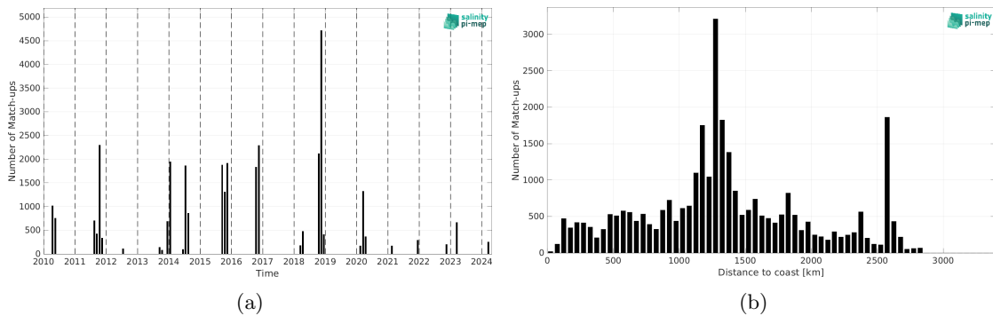
Figure 2: Number of match-ups between TSG (SAMOS) and SMOS SSS L2Q v331 - No FLAG (CMEMS-CATDS-CPDC) SSS as a function of time (a) and as function of the distance to coast (b) over the South Atlantic Ocean Pi-MEP region and for the full satellite product period.
