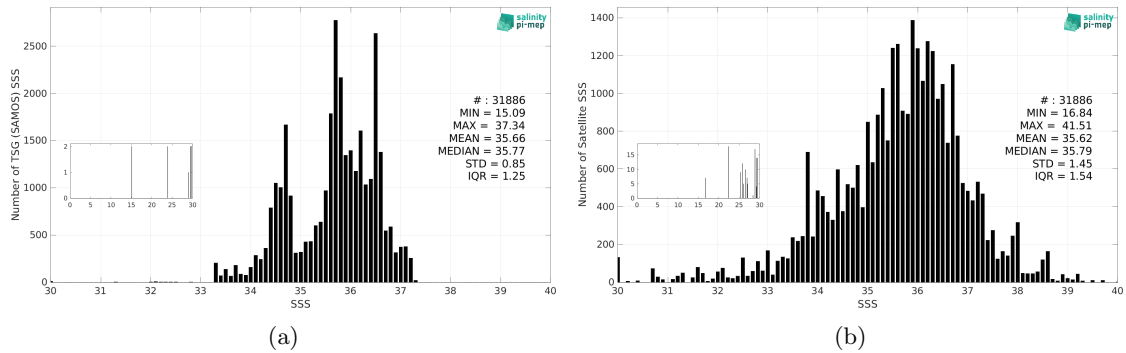
Figure 3: Histograms of SSS from TSG (SAMOS) (a) and SMOS SSS L2Q v331 - No FLAG (CMEMS-CATDS-CPDC) (b) considering all match-up pairs per bins of 0.1 over the South Atlantic Ocean Pi-MEP region and for the full satellite product period.
