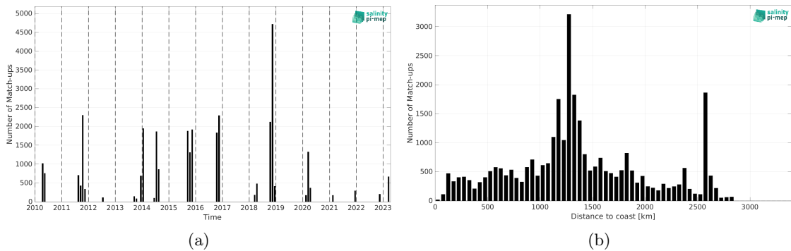
Figure 1: Number of match-ups between TSG (SAMOS) and SMOS SSS L2Q v331 - No FLAG (CMEMS-CATDS-CPDC) SSS as a function of time (a) and as function of the distance to coast (b) over the South Atlantic Ocean Pi-MEP region and for the full satellite product period.
