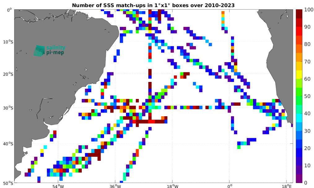
Figure 4: Number of SSS match-ups between TSG (SAMOS) SSS and the SMOS SSS L2Q v331 - No FLAG (CMEMS-CATDS-CPDC) SSS product for the South Atlantic Ocean Pi-MEP region over 1^\circ \times 1^\circ boxes and for the full satellite product period.
