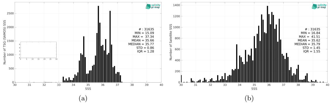
Figure 2: Histograms of SSS from TSG (SAMOS) (a) and SMOS SSS L2Q v331 - No FLAG (CMEMS-CATDS-CPDC) (b) considering all match-up pairs per bins of 0.1 over the South Atlantic Ocean Pi-MEP region and for the full satellite product period.
