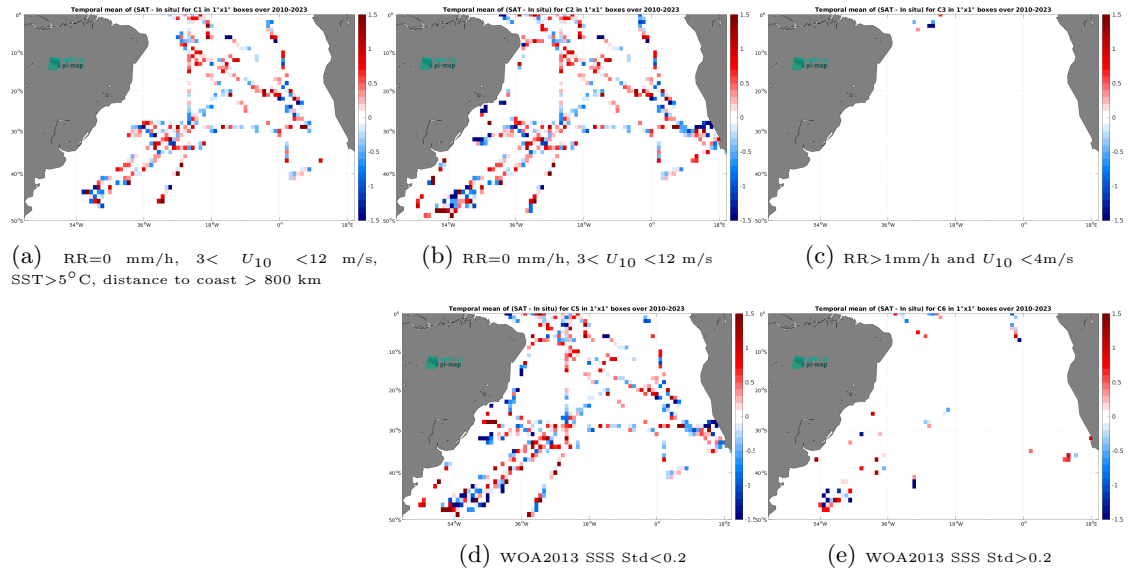
Figure 12: Temporal mean gridded over spatial boxes of size 1^\circ \times 1^\circ of \Delta\text{SSS} (SMOS SSS L2Q v331 - No FLAG (CMEMS-CATDS-CPDC) - TSG (SAMOS)) for 5 different subdatasets corresponding to:RR=0 mm/h, 3 < U_{10} < 12 m/s, SST >5^\circ\text{C} , distance to coast > 800 km (a), RR=0 mm/h, 3 < U_{10} < 12 m/s (b), RR >1 mm/h and U_{10} < 4 m/s (c), WOA2013 SSS Std <0.2 (d), WOA2013 SSS Std >0.2 (e).
