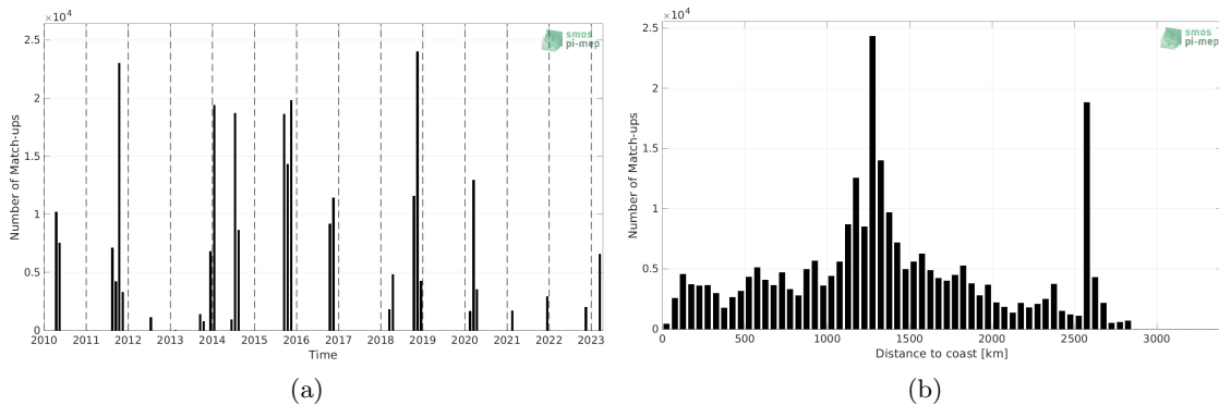
Figure 1: Number of match-ups between TSG (SAMOS) and SMOS SSS L2Q v331 - No FLAG (CMEMS-CATDS-CPDC) SSS as a function of time (a) and as function of the distance to coast (b) over the South Atlantic Ocean Pi-MEP region and for the full satellite product period.
