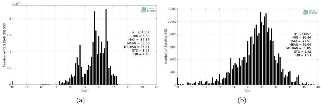
Figure 2: Histograms of SSS from TSG (SAMOS) (a) and SMOS SSS L2Q v331 - No FLAG (CMEMS-CATDS-CPDC) (b) considering all match-up pairs per bins of 0.1 over the South Atlantic Ocean Pi-MEP region and for the full satellite product period.
