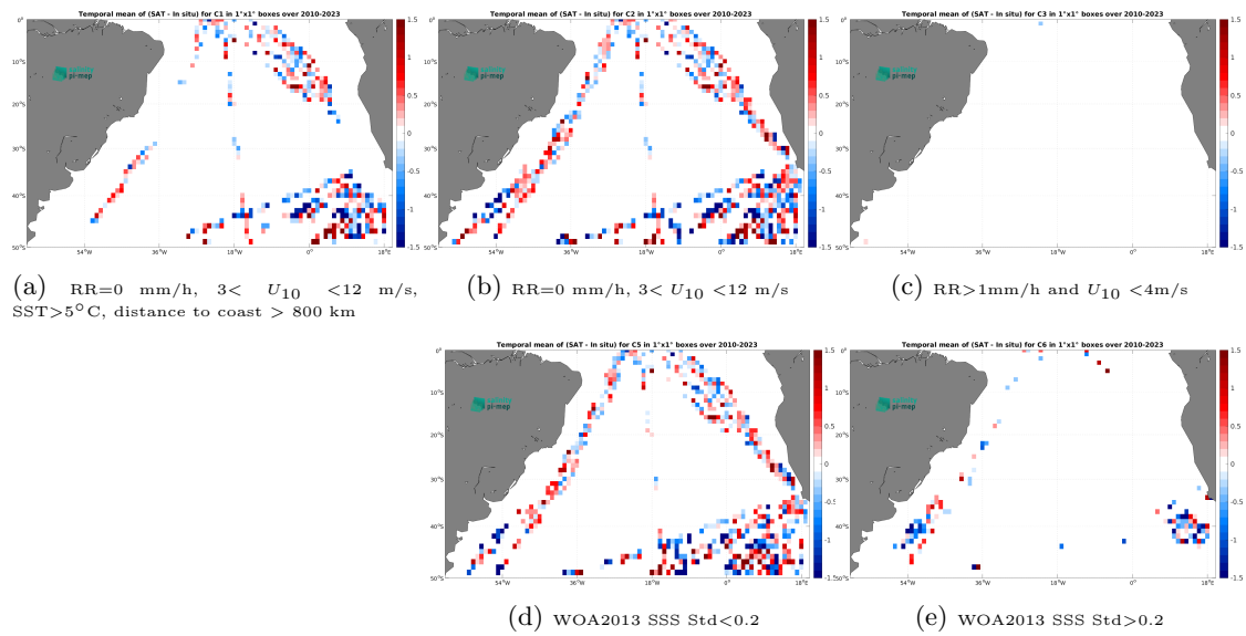
Figure 14: Temporal mean gridded over spatial boxes of size 1^\circ \times 1^\circ of \Delta\text{SSS} (SMOS SSS L2Q v331 - No FLAG (CMEMS-CATDS-CPDC) - TSG (Polarstern)) for 5 different subdatasets corresponding to:RR=0 mm/h, 3 < U_{10} < 12 m/s, SST >5^\circ\text{C} , distance to coast > 800 km (a), RR=0 mm/h, 3 < U_{10} < 12 m/s (b), RR >1 mm/h and U_{10} < 4 m/s (c), WOA2013 SSS Std <0.2 (d), WOA2013 SSS Std >0.2 (e).
