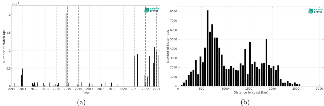
Figure 2: Number of match-ups between TSG (Polarstern) and SMOS SSS L2Q v331 - No FLAG (CMEMS-CATDS-CPDC) SSS as a function of time (a) and as function of the distance to coast (b) over the South Atlantic Ocean Pi-MEP region and for the full satellite product period.
