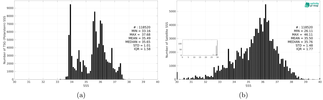
Figure 3: Histograms of SSS from TSG (Polarstern) (a) and SMOS SSS L2Q v331 - No FLAG (CMEMS-CATDS-CPDC) (b) considering all match-up pairs per bins of 0.1 over the South Atlantic Ocean Pi-MEP region and for the full satellite product period.
