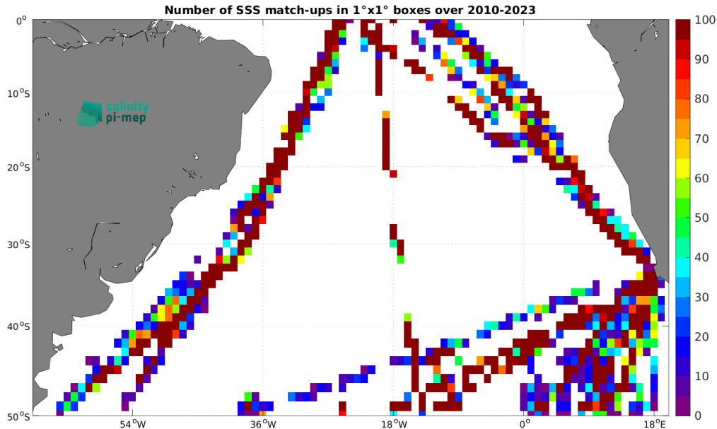
Figure 5: Number of SSS match-ups between TSG (Polarstern) SSS and the SMOS SSS L2Q v331 - No FLAG (CMEMS-CATDS-CPDC) SSS product for the South Atlantic Ocean Pi-MEP region over 1^\circ \times 1^\circ boxes and for the full satellite product period.
