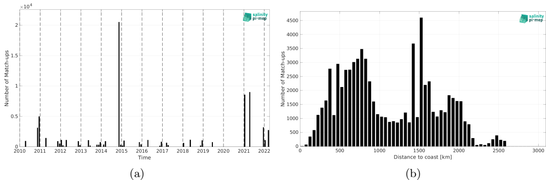
Figure 1: Number of match-ups between TSG (Polarstern) and SMOS SSS L2Q v331 - No FLAG (CMEMS-CATDS-CPDC) SSS as a function of time (a) and as function of the distance to coast (b) over the South Atlantic Ocean Pi-MEP region and for the full satellite product period.
