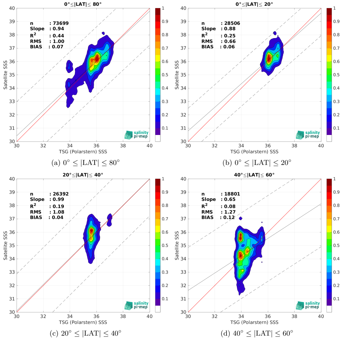
Figure 9: Contour maps of the concentration of SMOS SSS L2Q v331 - No FLAG (CMEMS-CATDS-CPDC) SSS (y-axis) versus TSG (Polarstern) SSS (x-axis) at match-up pairs for different latitude bands. For each plot, the red line shows x=y . The black thin and dashed lines indicate a linear fit through the data cloud and the \pm 95\% confidence levels, respectively. The number match-up pairs n , the slope and R^2 coefficient of the linear fit, the root mean square (RMS) and the mean bias between satellite and in situ data are indicated for each latitude band in each plots.
