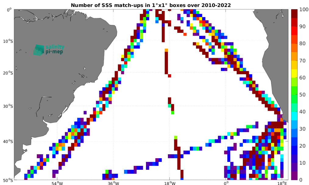
Figure 4: Number of SSS match-ups between TSG (Polarstern) SSS and the SMOS SSS L2Q v331 - No FLAG (CMEMS-CATDS-CPDC) SSS product for the South Atlantic Ocean Pi-MEP region over 1^\circ \times 1^\circ boxes and for the full satellite product period.
