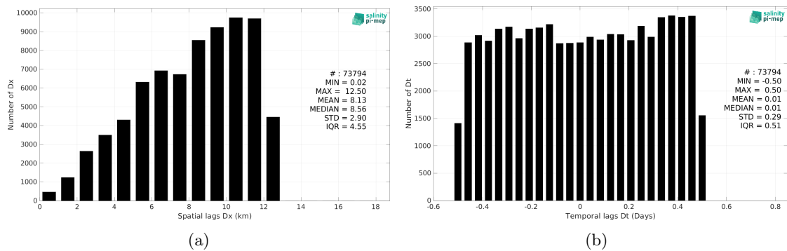
Figure 5: Histograms of the spatial (a) and temporal (b) lags between the location/time of the TSG (Polarstern) measurement and the date of the corresponding SMOS SSS L2Q v331 - No FLAG (CMEMS-CATDS-CPDC) SSS pixel.
