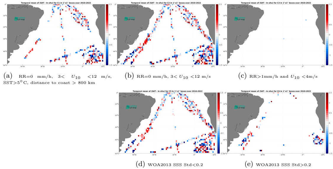
Figure 12: Temporal mean gridded over spatial boxes of size 1^\circ \times 1^\circ of \Delta SSS (SMOS SSS L2Q v331 - No FLAG (CMEMS-CATDS-CPDC) - TSG (Polarstern)) for 5 different subdatasets corresponding to:RR=0 mm/h, 3 < U_{10} < 12 m/s, SST >5^\circ\text{C} , distance to coast > 800 km (a), RR=0 mm/h, 3 < U_{10} < 12 m/s (b), RR >1 mm/h and U_{10} < 4 m/s (c), WOA2013 SSS Std <0.2 (d), WOA2013 SSS Std >0.2 (e).
