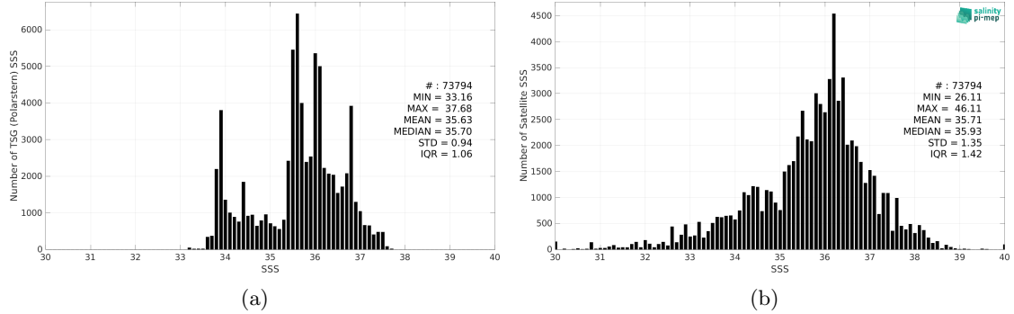
Figure 2: Histograms of SSS from TSG (Polarstern) (a) and SMOS SSS L2Q v331 - No FLAG (CMEMS-CATDS-CPDC) (b) considering all match-up pairs per bins of 0.1 over the South Atlantic Ocean Pi-MEP region and for the full satellite product period.
