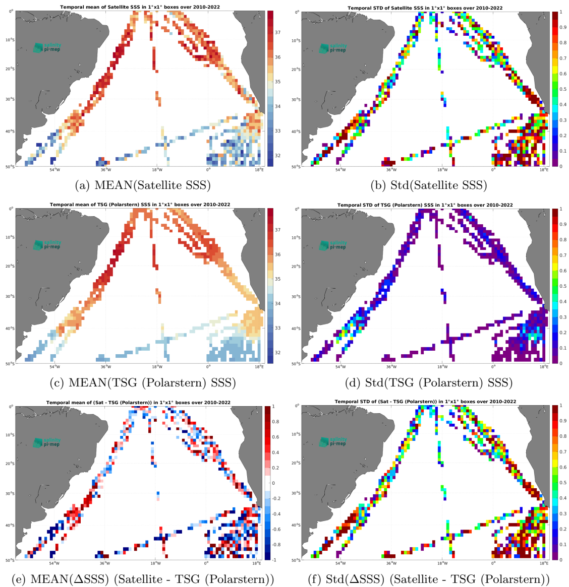
Figure 6: Temporal mean (left) and Std (right) of SSS from SMOS SSS L2Q v331 - No FLAG (CMEMS-CATDS-CPDC) (top), TSG (Polarstern) (middle), and of \Delta SSS (Satellite - TSG (Polarstern)). Only match-up pairs are used to generate these maps.
