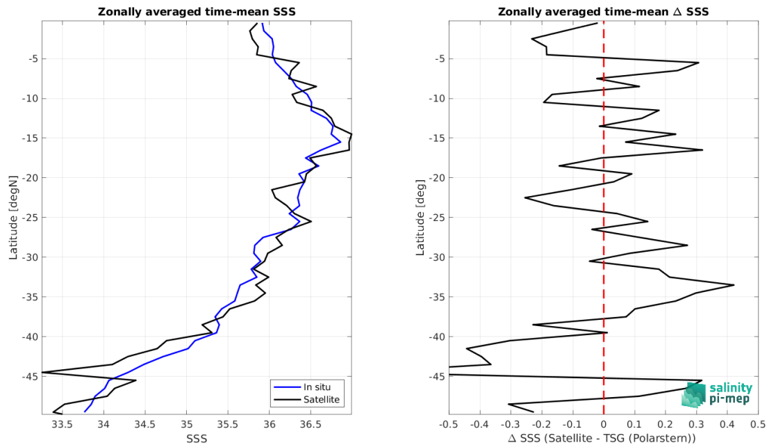
Figure 8: Left panel: Zonal mean SSS from SMOS SSS L2Q v331 - No FLAG (CMEMS-CATDS-CPDC) satellite product (black) and from TSG (Polarstern) (blue). Right panel: Zonal mean of \Delta SSS (Satellite - TSG (Polarstern)) for all the collected Pi-MEP match-up pairs estimated over the full satellite product period.
