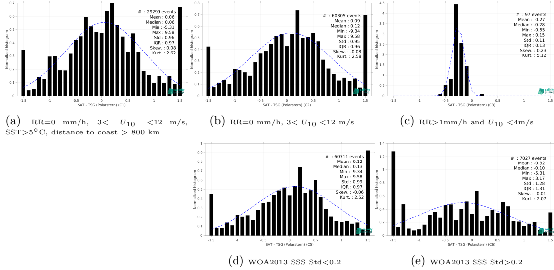
Figure 13: Normalized histogram of \Delta SSS (SMOS SSS L2Q v331 - No FLAG (CMEMS-CATDS-CPDC) - TSG (Polarstern)) for 5 different subdatasets corresponding to: RR=0 mm/h, 3 < U_{10} < 12 m/s, SST > 5°C, distance to coast > 800 km (a), RR=0 mm/h, 3 < U_{10} < 12 m/s (b), RR > 1mm/h and U_{10} < 4 m/s (c), WOA2013 SSS Std < 0.2 (d), WOA2013 SSS Std > 0.2 (e).
