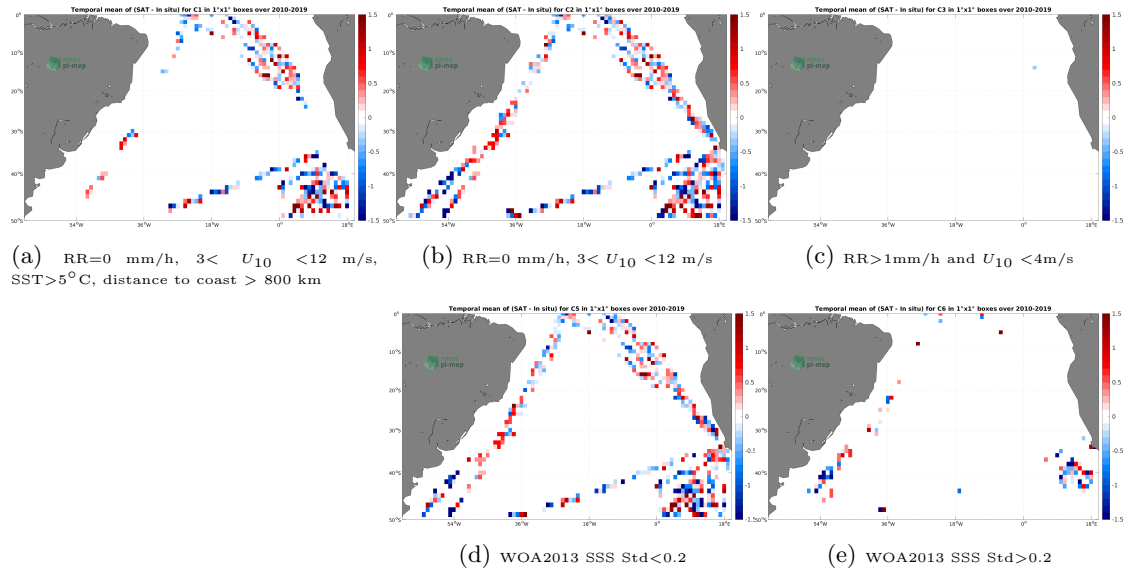
Figure 12: Temporal mean gridded over spatial boxes of size 1^\circ \times 1^\circ of \Delta\text{SSS} (SMOS SSS L2Q v331 - No FLAG (CMEMS-CATDS-CPDC) - TSG (Polarstern)) for 5 different subdatasets corresponding to:RR=0 mm/h, 3 < U_{10} < 12 m/s, SST >5^\circ\text{C} , distance to coast > 800 km (a), RR=0 mm/h, 3 < U_{10} < 12 m/s (b), RR >1 mm/h and U_{10} < 4 m/s (c), WOA2013 SSS Std <0.2 (d), WOA2013 SSS Std >0.2 (e).
