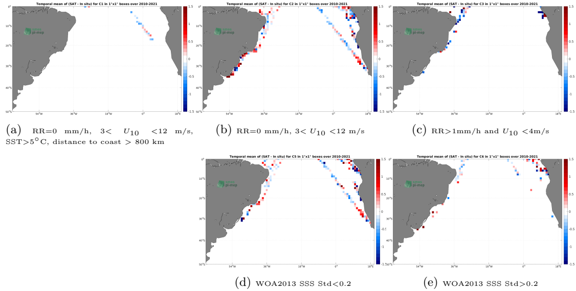
Figure 12: Temporal mean gridded over spatial boxes of size 1^{\circ}\times 1^{\circ} of \Delta\text{SSS} (SMOS SSS L2Q v331 - No FLAG (CMEMS-CATDS-CPDC) - TSG (LEGOS-DM)) for 5 different subdatasets corresponding to:RR=0 mm/h, 3 < U_{10} < 12 m/s, SST >5^{\circ}\text{C} , distance to coast > 800 km (a), RR=0 mm/h, 3 < U_{10} < 12 m/s (b), RR >1 mm/h and U_{10} < 4 m/s (c), WOA2013 SSS Std <0.2 (d), WOA2013 SSS Std >0.2 (e).
