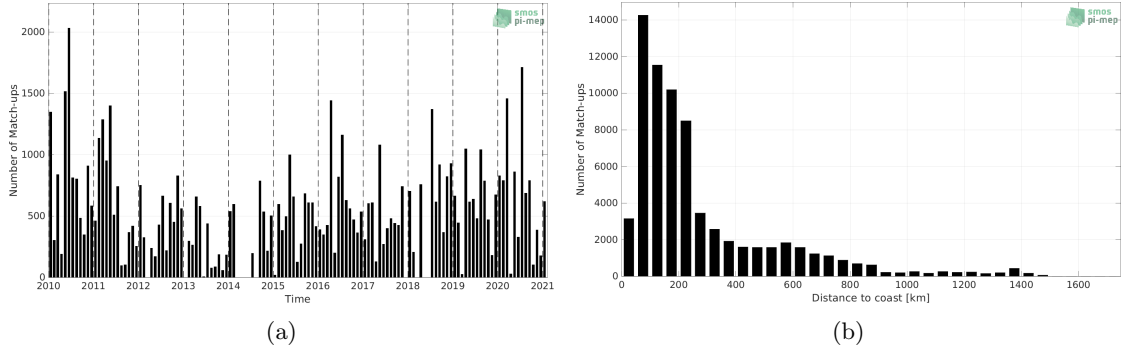
Figure 1: Number of match-ups between TSG (LEGOS-DM) and SMOS SSS L2Q v331 - No FLAG (CMEMS-CATDS-CPDC) SSS as a function of time (a) and as function of the distance to coast (b) over the South Atlantic Ocean Pi-MEP region and for the full satellite product period.
