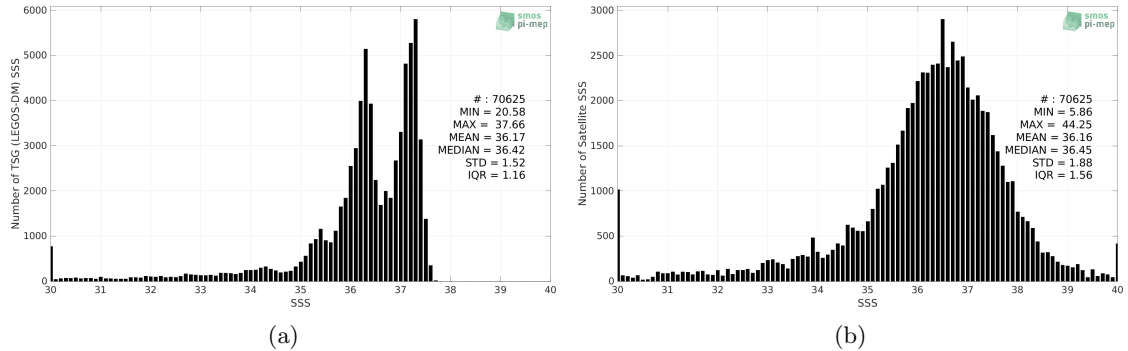
Figure 2: Histograms of SSS from TSG (LEGOS-DM) (a) and SMOS SSS L2Q v331 - No FLAG (CMEMS-CATDS-CPDC) (b) considering all match-up pairs per bins of 0.1 over the South Atlantic Ocean Pi-MEP region and for the full satellite product period.
