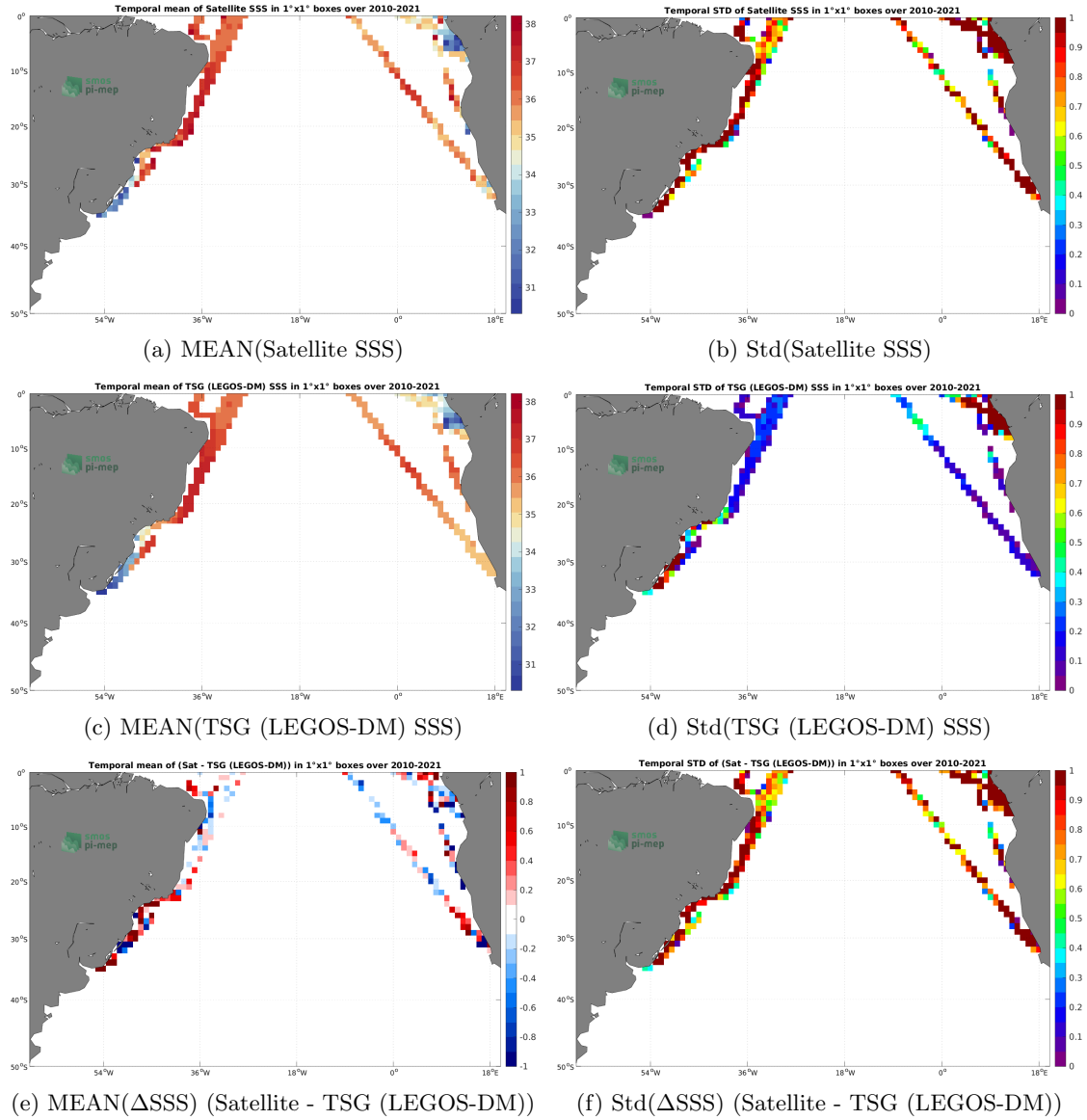
Figure 6: Temporal mean (left) and Std (right) of SSS from SMOS SSS L2Q v331 - No FLAG (CMEMS-CATDS-CPDC) (top), TSG (LEGOS-DM) (middle), and of \Delta SSS (Satellite - TSG (LEGOS-DM)). Only match-up pairs are used to generate these maps.
