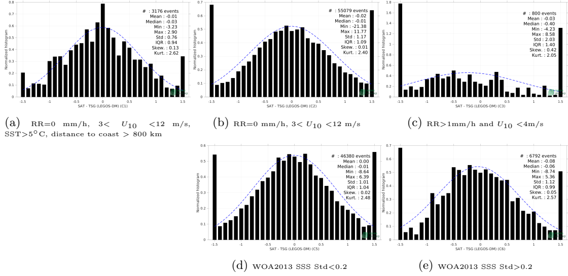
Figure 13: Normalized histogram of \Delta SSS (SMOS SSS L2Q v331 - No FLAG (CMEMS-CATDS-CPDC) - TSG (LEGOS-DM)) for 5 different subdatasets corresponding to: RR=0 mm/h, 3 < U_{10} < 12 m/s, SST > 5°C, distance to coast > 800 km (a), RR=0 mm/h, 3 < U_{10} < 12 m/s (b), RR > 1mm/h and U_{10} < 4 m/s (c), WOA2013 SSS Std < 0.2 (d), WOA2013 SSS Std > 0.2 (e).
