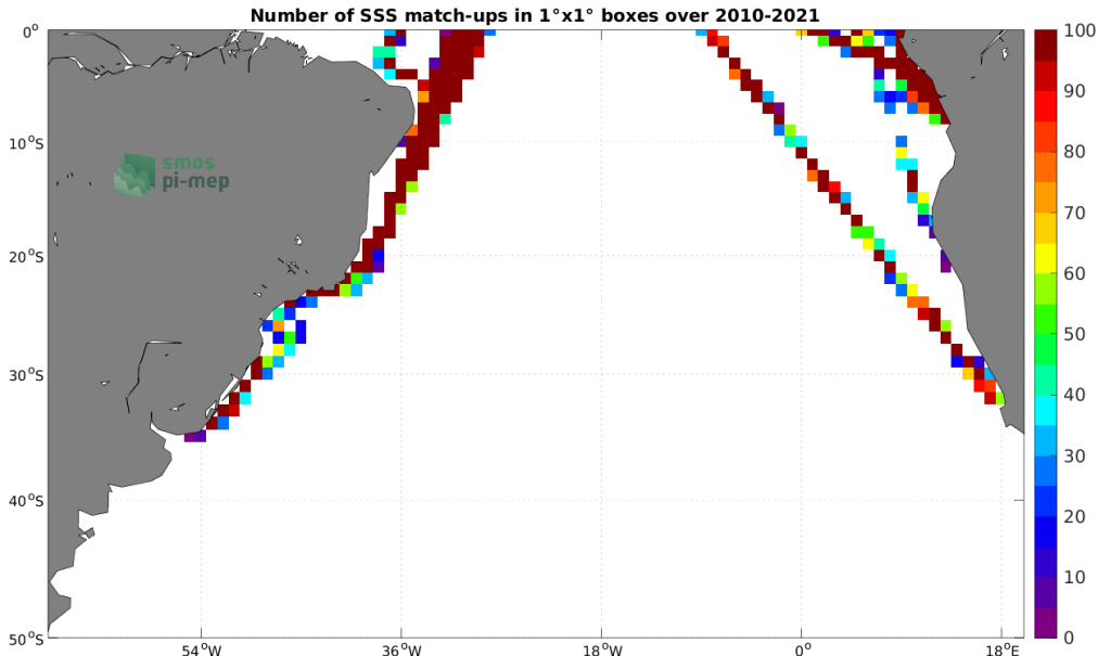
Figure 4: Number of SSS match-ups between TSG (LEGOS-DM) SSS and the SMOS SSS L2Q v331 - No FLAG (CMEMS-CATDS-CPDC) SSS product for the South Atlantic Ocean Pi-MEP region over 1^\circ \times 1^\circ boxes and for the full satellite product period.
