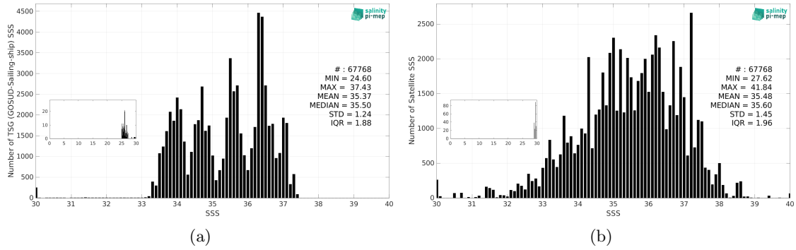
Figure 3: Histograms of SSS from TSG (GOSUD-Sailing-ship) (a) and SMOS SSS L2Q v331 - No FLAG (CMEMS-CATDS-CPDC) (b) considering all match-up pairs per bins of 0.1 over the South Atlantic Ocean Pi-MEP region and for the full satellite product period.
