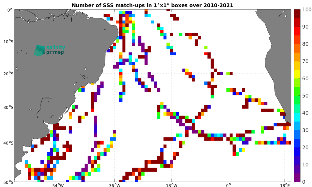
Figure 5: Number of SSS match-ups between TSG (GOSUD-Sailing-ship) SSS and the SMOS SSS L2Q v331 - No FLAG (CMEMS-CATDS-CPDC) SSS product for the South Atlantic Ocean Pi-MEP region over 1^\circ \times 1^\circ boxes and for the full satellite product period.
