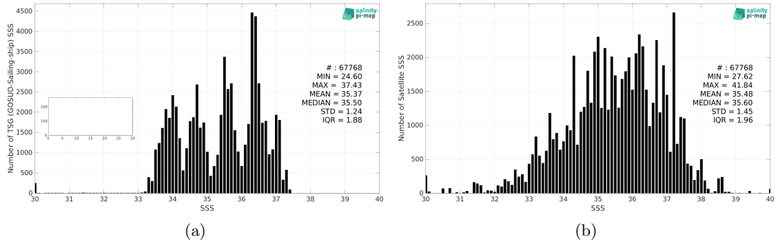
Figure 2: Histograms of SSS from TSG (GOSUD-Sailing-ship) (a) and SMOS SSS L2Q v331 - No FLAG (CMEMS-CATDS-CPDC) (b) considering all match-up pairs per bins of 0.1 over the South Atlantic Ocean Pi-MEP region and for the full satellite product period.
