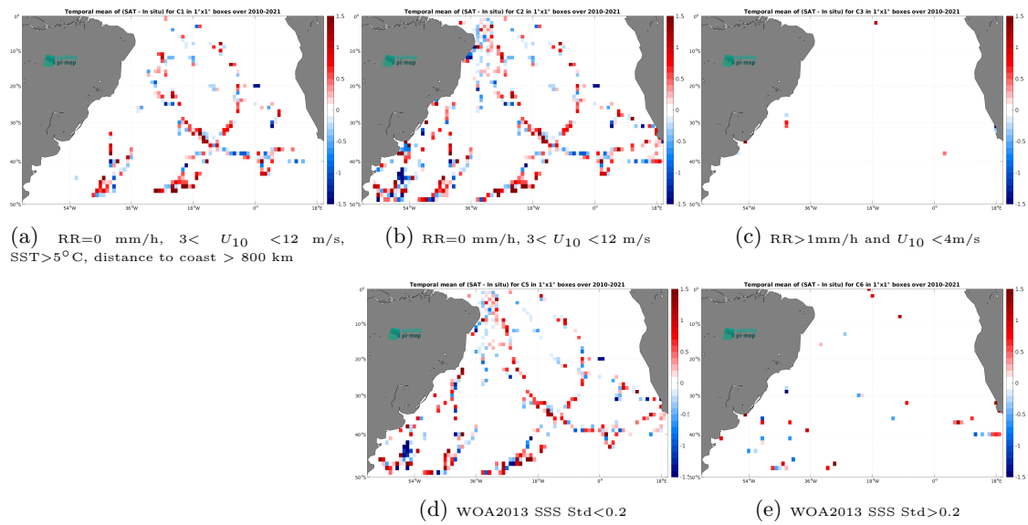
Figure 12: Temporal mean gridded over spatial boxes of size 1^\circ \times 1^\circ of \Delta\text{SSS} (SMOS SSS L2Q v331 - No FLAG (CMEMS-CATDS-CPDC) - TSG (GOSUD-Sailing-ship)) for 5 different sub-datasets corresponding to:RR=0 mm/h, 3 < U_{10} < 12 m/s, SST>5°C, distance to coast > 800 km (a), RR=0 mm/h, 3 < U_{10} < 12 m/s (b), RR>1mm/h and U_{10} < 4 m/s (c), WOA2013 SSS Std<0.2 (d), WOA2013 SSS Std>0.2 (e).
