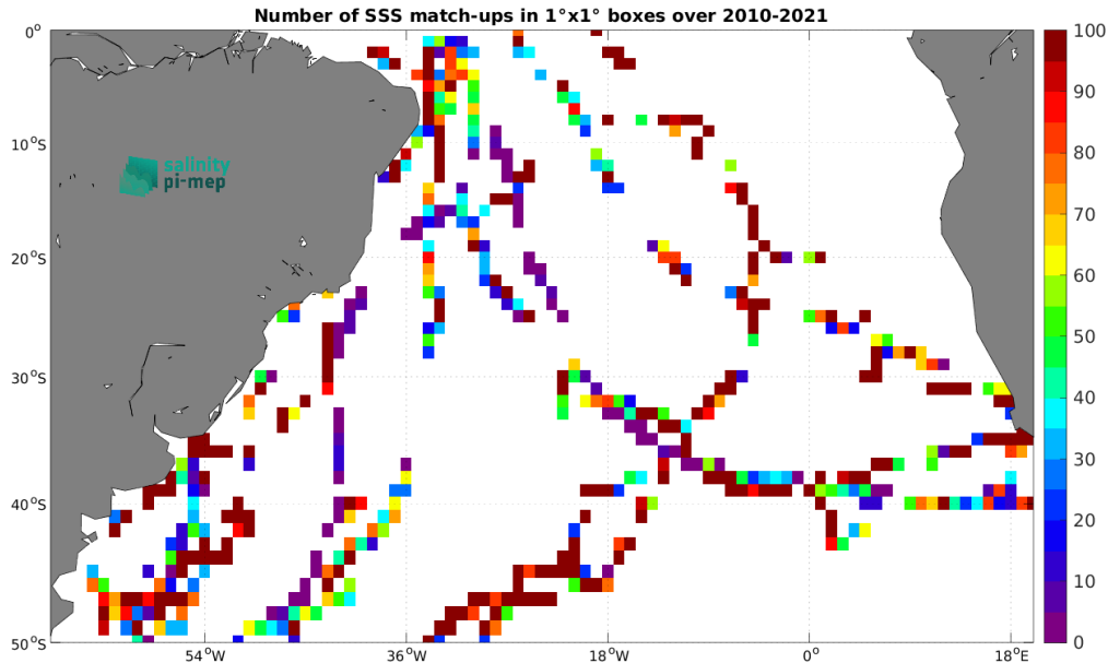
Figure 4: Number of SSS match-ups between TSG (GOSUD-Sailing-ship) SSS and the SMOS SSS L2Q v331 - No FLAG (CMEMS-CATDS-CPDC) SSS product for the South Atlantic Ocean Pi-MEP region over 1^\circ \times 1^\circ boxes and for the full satellite product period.
