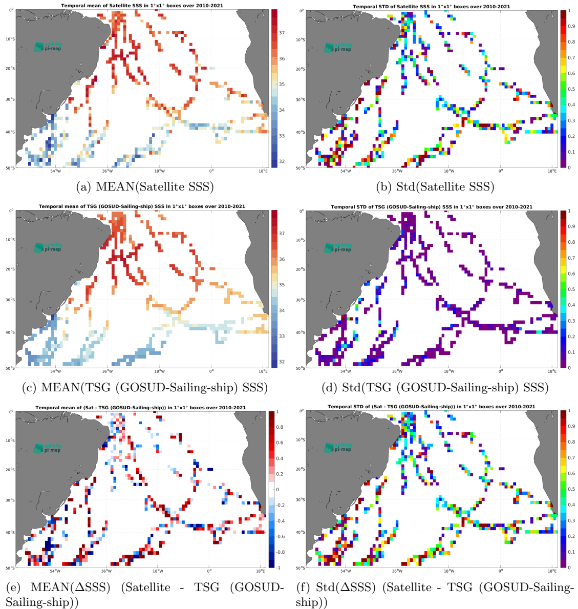
Figure 6: Temporal mean (left) and Std (right) of SSS from SMOS SSS L2Q v331 - No FLAG (CMEMS-CATDS-CPDC) (top), TSG (GOSUD-Sailing-ship) (middle), and of \Delta SSS (Satellite - TSG (GOSUD-Sailing-ship)). Only match-up pairs are used to generate these maps.
