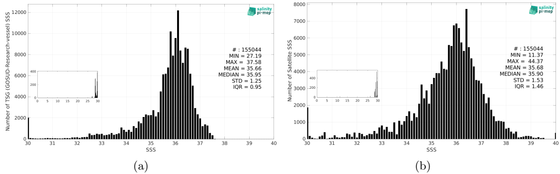
Figure 3: Histograms of SSS from TSG (GOSUD-Research-vessel) (a) and SMOS SSS L2Q v331 - No FLAG (CMEMS-CATDS-CPDC) (b) considering all match-up pairs per bins of 0.1 over the South Atlantic Ocean Pi-MEP region and for the full satellite product period.
