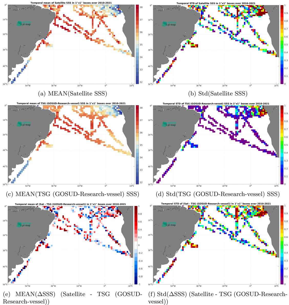
Figure 7: Temporal mean (left) and Std (right) of SSS from SMOS SSS L2Q v331 - No FLAG (CMEMS-CATDS-CPDC) (top), TSG (GOSUD-Research-vessel) (middle), and of \Delta SSS (Satellite - TSG (GOSUD-Research-vessel)). Only match-up pairs are used to generate these maps.
