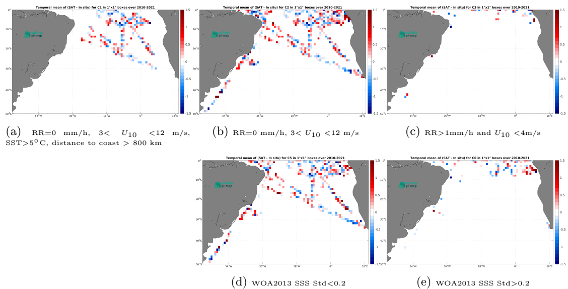
Figure 14: Temporal mean gridded over spatial boxes of size 1^\circ \times 1^\circ of \Delta\text{SSS} (SMOS SSS L2Q v331 - No FLAG (CMEMS-CATDS-CPDC) - TSG (GOSUD-Research-vessel)) for 5 different subdatasets corresponding to:RR=0 mm/h, 3 < U_{10} < 12 m/s, SST>5°C, distance to coast > 800 km (a), RR=0 mm/h, 3 < U_{10} < 12 m/s (b), RR>1mm/h and U_{10} < 4 m/s (c), WOA2013 SSS Std<0.2 (d), WOA2013 SSS Std>0.2 (e).
