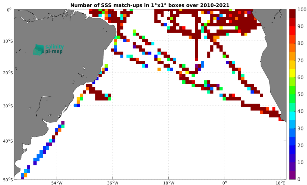
Figure 4: Number of SSS match-ups between TSG (GOSUD-Research-vessel) SSS and the SMOS SSS L2Q v331 - No FLAG (CMEMS-CATDS-CPDC) SSS product for the South Atlantic Ocean Pi-MEP region over 1^{\circ} \times 1^{\circ} boxes and for the full satellite product period.
