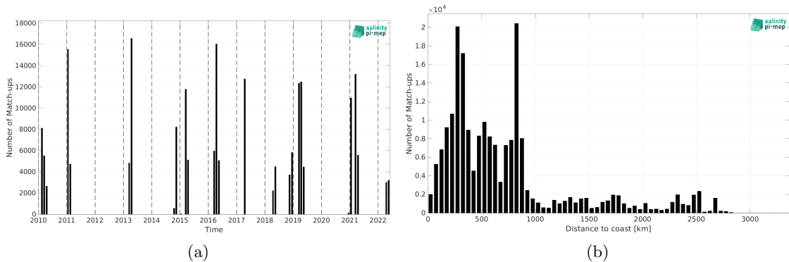
Figure 2: Number of match-ups between TSG (CSIC-UTM) and SMOS SSS L2Q v331 - No FLAG (CMEMS-CATDS-CPDC) SSS as a function of time (a) and as function of the distance to coast (b) over the South Atlantic Ocean Pi-MEP region and for the full satellite product period.
