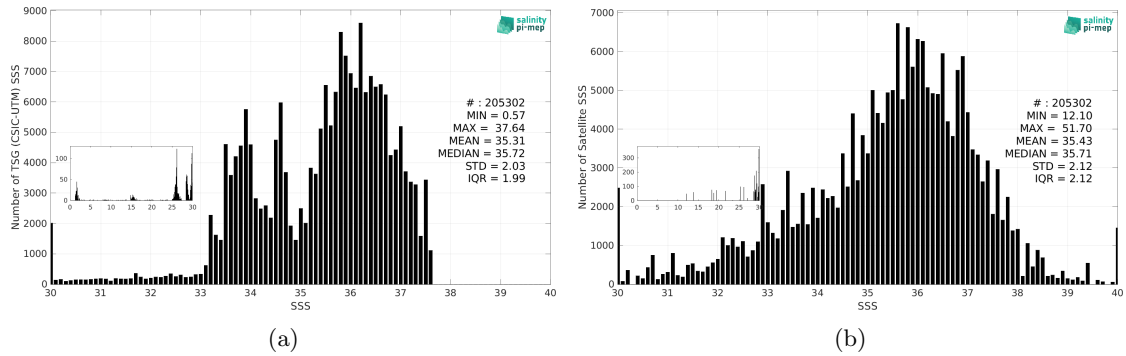
Figure 3: Histograms of SSS from TSG (CSIC-UTM) (a) and SMOS SSS L2Q v331 - No FLAG (CMEMS-CATDS-CPDC) (b) considering all match-up pairs per bins of 0.1 over the South Atlantic Ocean Pi-MEP region and for the full satellite product period.
