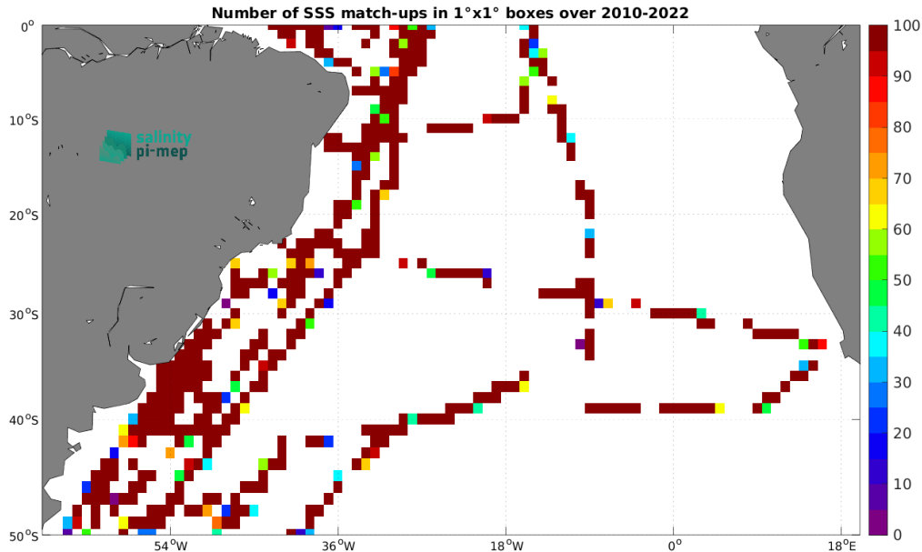
Figure 4: Number of SSS match-ups between TSG (CSIC-UTM) SSS and the SMOS SSS L2Q v331 - No FLAG (CMEMS-CATDS-CPDC) SSS product for the South Atlantic Ocean Pi-MEP region over 1^{\circ} \times 1^{\circ} boxes and for the full satellite product period.
