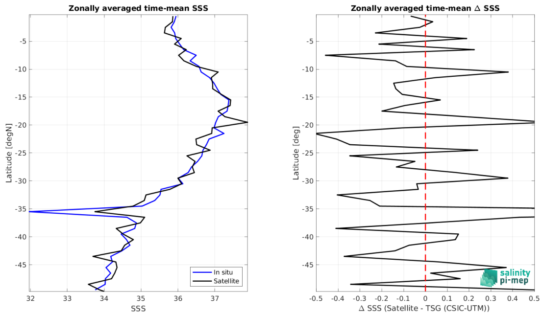
Figure 8: Left panel: Zonal mean SSS from SMOS SSS L2Q v331 - No FLAG (CMEMS-CATDS-CPDC) satellite product (black) and from TSG (CSIC-UTM) (blue). Right panel: Zonal mean of \Delta SSS (Satellite - TSG (CSIC-UTM)) for all the collected Pi-MEP match-up pairs estimated over the full satellite product period.
