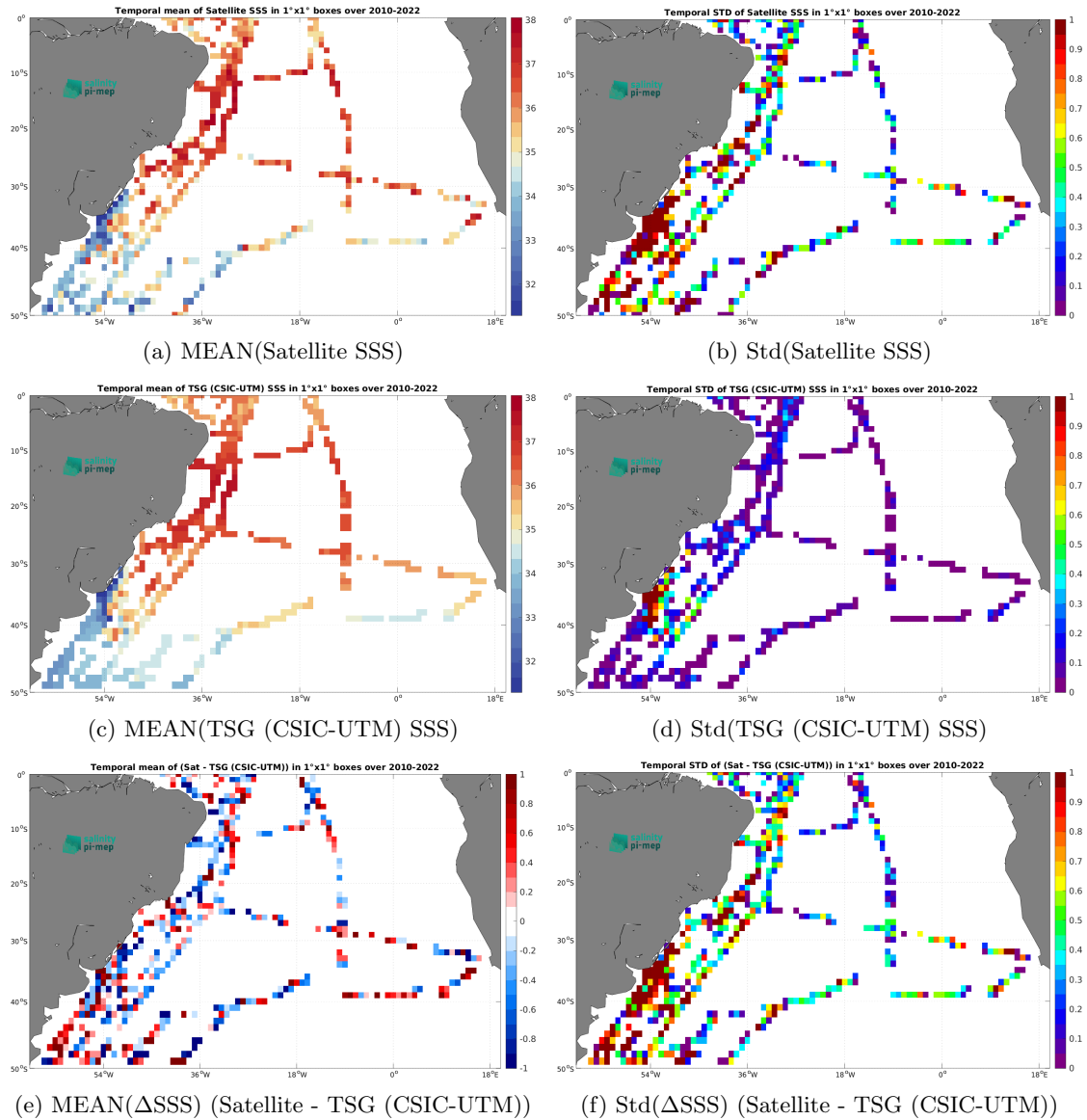
Figure 6: Temporal mean (left) and Std (right) of SSS from SMOS SSS L2Q v331 - No FLAG (CMEMS-CATDS-CPDC) (top), TSG (CSIC-UTM) (middle), and of \Delta SSS (Satellite - TSG (CSIC-UTM)). Only match-up pairs are used to generate these maps.
