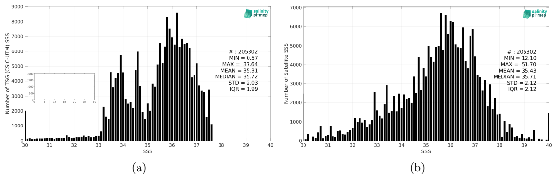
Figure 2: Histograms of SSS from TSG (CSIC-UTM) (a) and SMOS SSS L2Q v331 - No FLAG (CMEMS-CATDS-CPDC) (b) considering all match-up pairs per bins of 0.1 over the South Atlantic Ocean Pi-MEP region and for the full satellite product period.
