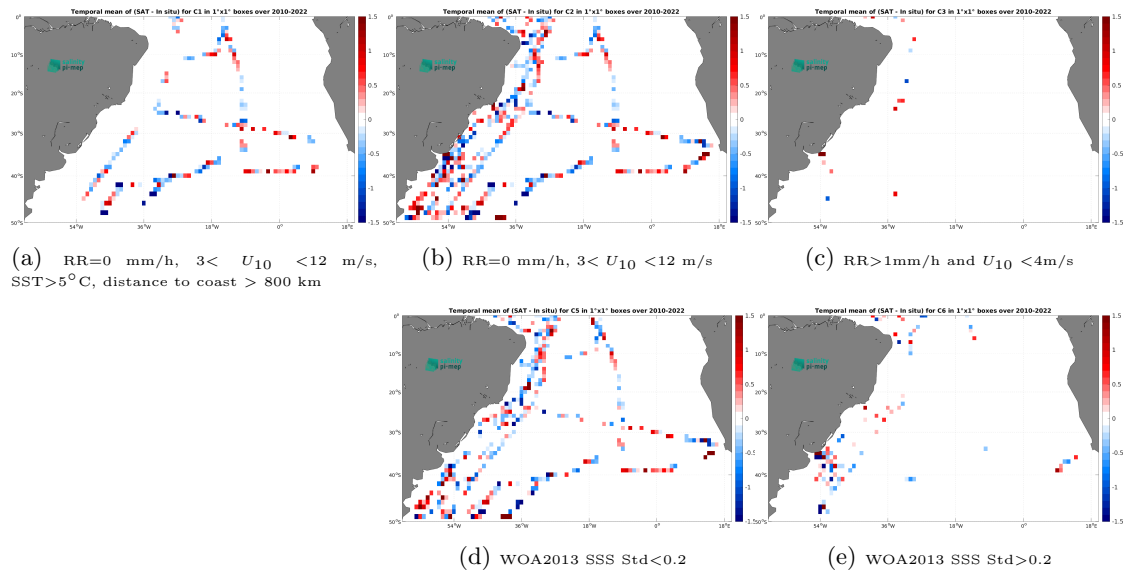
Figure 12: Temporal mean gridded over spatial boxes of size 1^\circ \times 1^\circ of \Delta SSS (SMOS SSS L2Q v331 - No FLAG (CMEMS-CATDS-CPDC) - TSG (CSIC-UTM)) for 5 different subdatasets corresponding to:RR=0 mm/h, 3 < U_{10} < 12 m/s, SST >5^\circ\text{C} , distance to coast > 800 km (a), RR=0 mm/h, 3 < U_{10} < 12 m/s (b), RR >1 mm/h and U_{10} < 4 m/s (c), WOA2013 SSS Std <0.2 (d), WOA2013 SSS Std >0.2 (e).
