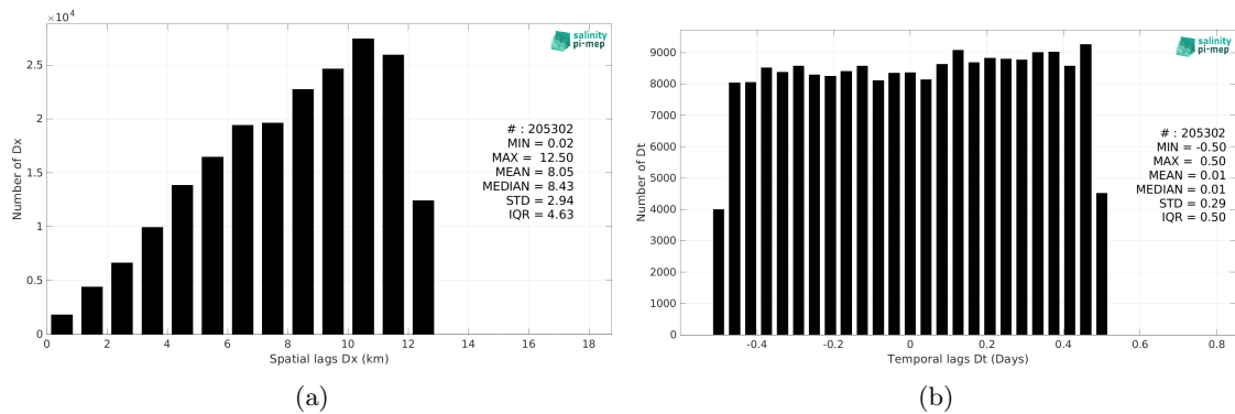
Figure 5: Histograms of the spatial (a) and temporal (b) lags between the location/time of the TSG (CSIC-UTM) measurement and the date of the corresponding SMOS SSS L2Q v331 - No FLAG (CMEMS-CATDS-CPDC) SSS pixel.
