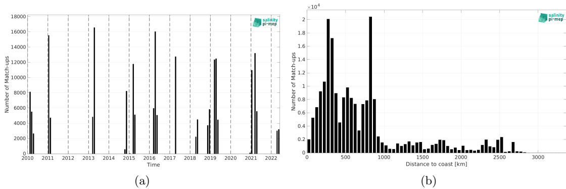
Figure 1: Number of match-ups between TSG (CSIC-UTM) and SMOS SSS L2Q v331 - No FLAG (CMEMS-CATDS-CPDC) SSS as a function of time (a) and as function of the distance to coast (b) over the South Atlantic Ocean Pi-MEP region and for the full satellite product period.
