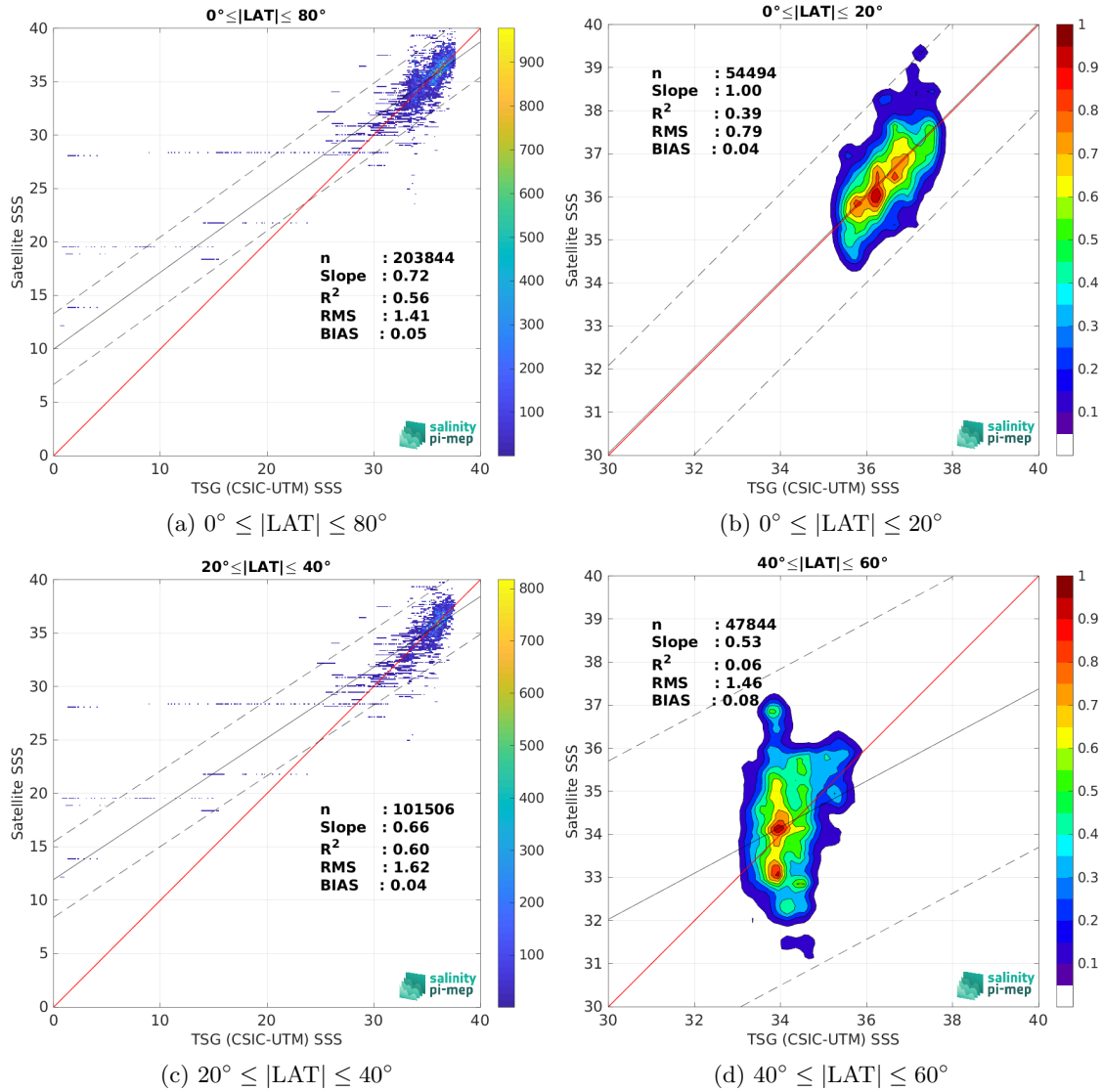
Figure 9: Contour maps of the concentration of SMOS SSS L2Q v331 - No FLAG (CMEMS-CATDS-CPDC) SSS (y-axis) versus TSG (CSIC-UTM) SSS (x-axis) at match-up pairs for different latitude bands. For each plot, the red line shows x=y . The black thin and dashed lines indicate a linear fit through the data cloud and the \pm 95\% confidence levels, respectively. The number match-up pairs n , the slope and R^2 coefficient of the linear fit, the root mean square (RMS) and the mean bias between satellite and in situ data are indicated for each latitude band in each plots.
