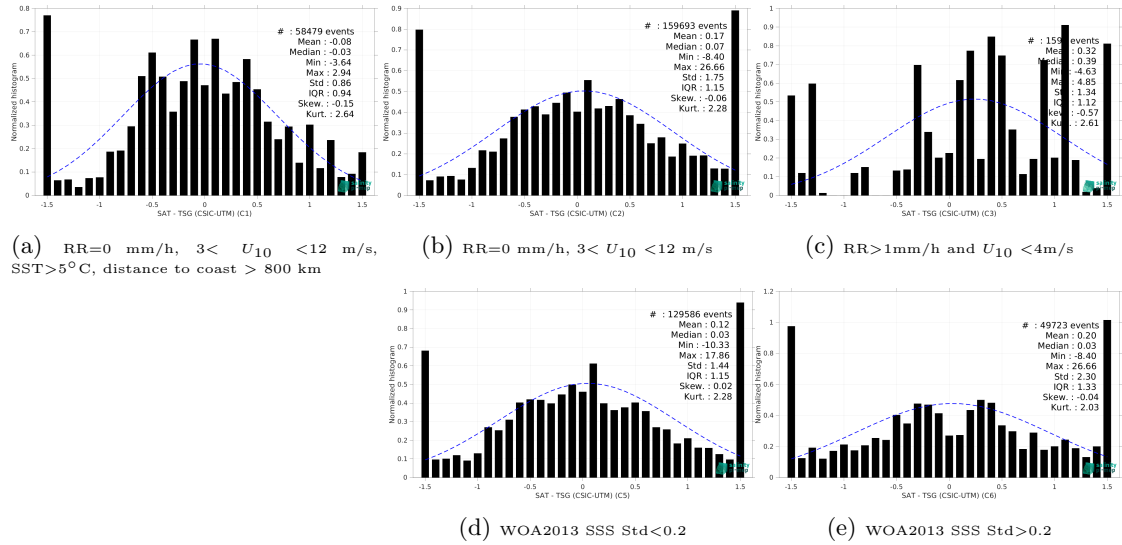
Figure 13: Normalized histogram of \Delta SSS (SMOS SSS L2Q v331 - No FLAG (CMEMS-CATDS-CPDC) - TSG (CSIC-UTM)) for 5 different subdatasets corresponding to: RR=0 mm/h, 3 < U_{10} < 12 m/s, SST > 5°C, distance to coast > 800 km (a), RR=0 mm/h, 3 < U_{10} < 12 m/s (b), RR > 1mm/h and U_{10} < 4 m/s (c), WOA2013 SSS Std < 0.2 (d), WOA2013 SSS Std > 0.2 (e).
