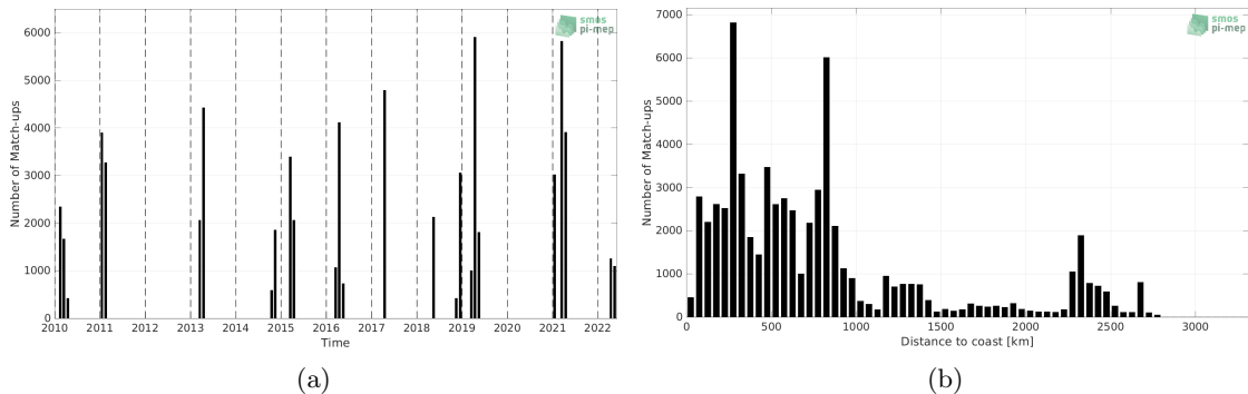
Figure 1: Number of match-ups between TSG (CSIC-UTM) and SMOS SSS L2Q v331 - No FLAG (CMEMS-CATDS-CPDC) SSS as a function of time (a) and as function of the distance to coast (b) over the South Atlantic Ocean Pi-MEP region and for the full satellite product period.
