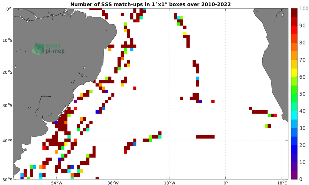
Figure 4: Number of SSS match-ups between TSG (CSIC-UTM) SSS and the SMOS SSS L2Q v331 - No FLAG (CMEMS-CATDS-CPDC) SSS product for the South Atlantic Ocean Pi-MEP region over 1^\circ \times 1^\circ boxes and for the full satellite product period.
