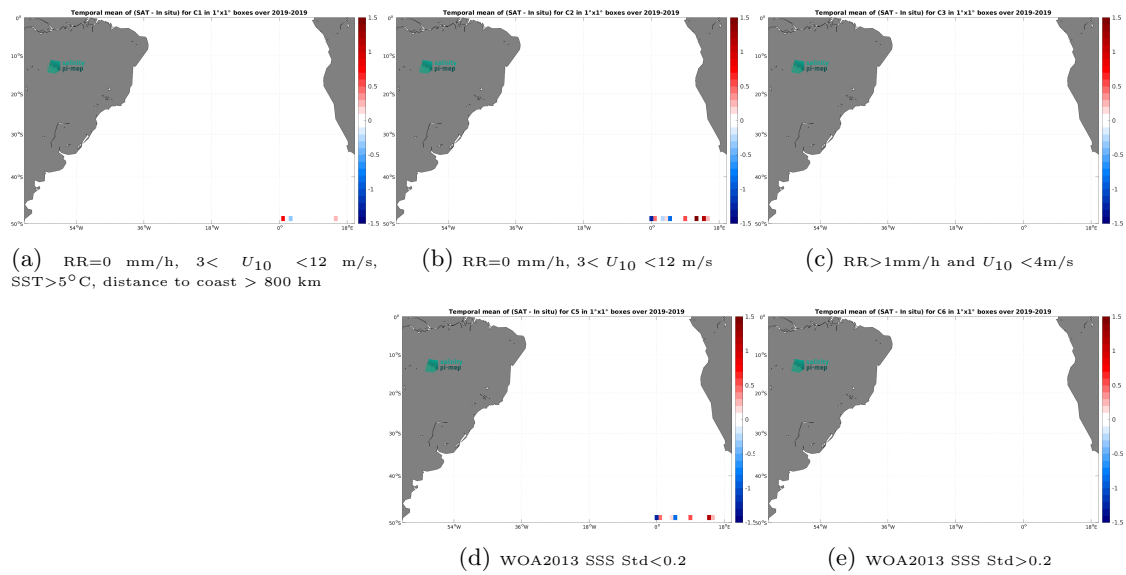
Figure 14: Temporal mean gridded over spatial boxes of size 1^\circ \times 1^\circ of \Delta SSS (SMOS SSS L2Q v331 - No FLAG (CMEMS-CATDS-CPDC) - Saildrone) for 5 different subdatasets corresponding to:RR=0 mm/h, 3 < U_{10} < 12 m/s, SST >5^\circ\text{C} , distance to coast > 800 km (a), RR=0 mm/h, 3 < U_{10} < 12 m/s (b), RR >1 mm/h and U_{10} < 4 m/s (c), WOA2013 SSS Std <0.2 (d), WOA2013 SSS Std >0.2 (e).
