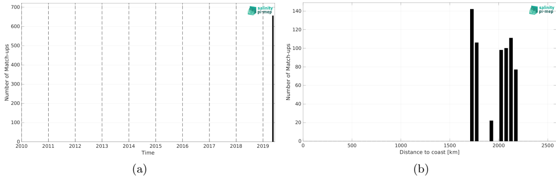
Figure 2: Number of match-ups between Saildrone and SMOS SSS L2Q v331 - No FLAG (CMEMS-CATDS-CPDC) SSS as a function of time (a) and as function of the distance to coast (b) over the South Atlantic Ocean Pi-MEP region and for the full satellite product period.
