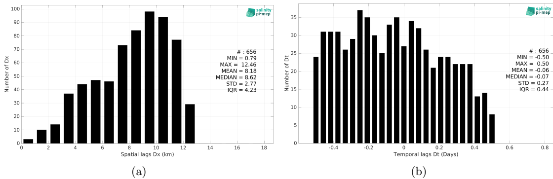
Figure 6: Histograms of the spatial (a) and temporal (b) lags between the location/time of the Sairdrone measurement and the date of the corresponding SMOS SSS L2Q v331 - No FLAG (CMEMS-CATDS-CPDC) SSS pixel.
