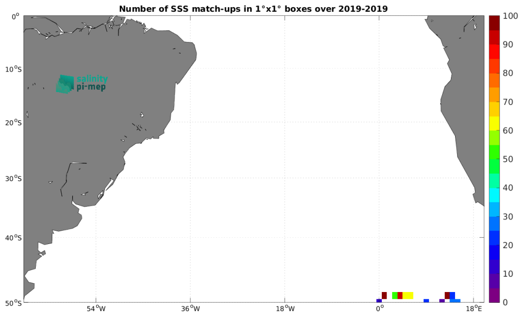
Figure 5: Number of SSS match-ups between Sairdrone SSS and the SMOS SSS L2Q v331 - No FLAG (CMEMS-CATDS-CPDC) SSS product for the South Atlantic Ocean Pi-MEP region over 1^\circ \times 1^\circ boxes and for the full satellite product period.
