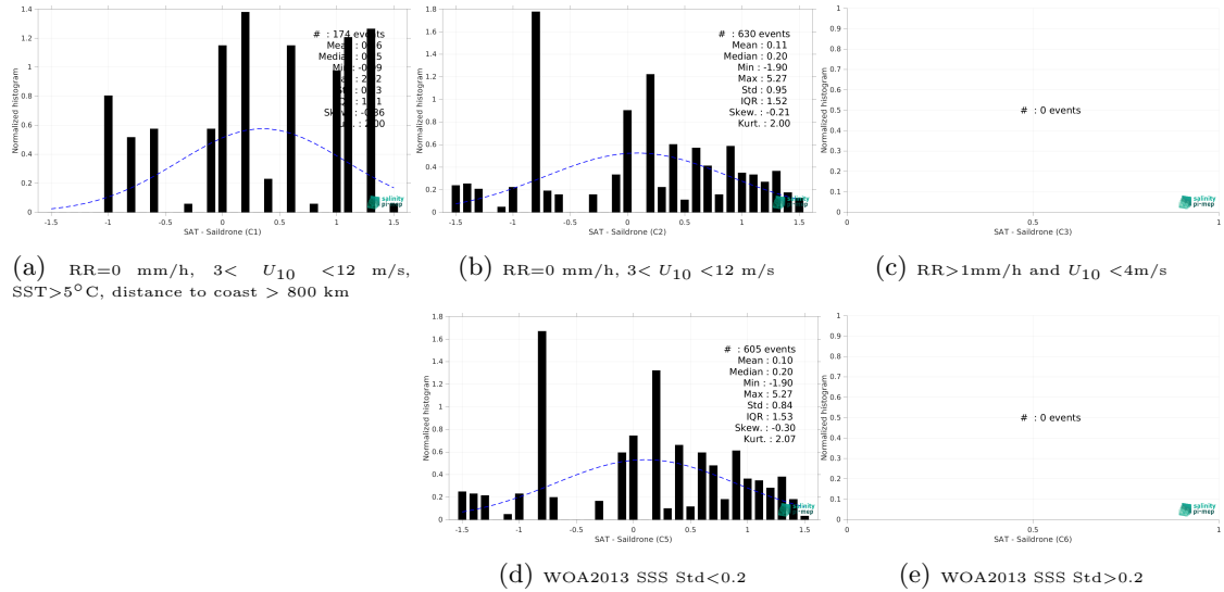
Figure 15: Normalized histogram of \Delta SSS (SMOS SSS L2Q v331 - No FLAG (CMEMS-CATDS-CPDC) - Saildrone) for 5 different subdatasets corresponding to: RR=0 mm/h, 3 < U_{10} < 12 m/s, SST > 5°C, distance to coast > 800 km (a), RR=0 mm/h, 3 < U_{10} < 12 m/s (b), RR > 1mm/h and U_{10} < 4 m/s (c), WOA2013 SSS Std < 0.2 (d), WOA2013 SSS Std > 0.2 (e).
