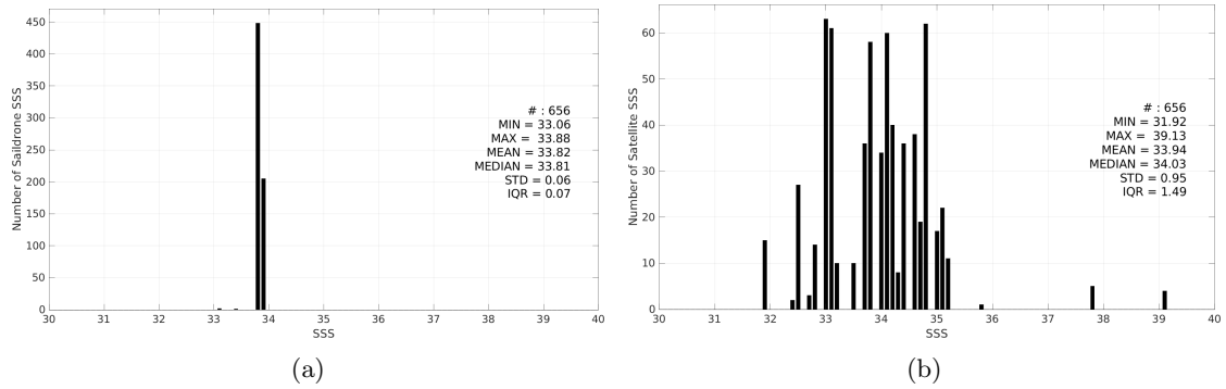
Figure 3: Histograms of SSS from Sailldrone (a) and SMOS SSS L2Q v331 - No FLAG (CMEMS-CATDS-CPDC) (b) considering all match-up pairs per bins of 0.1 over the South Atlantic Ocean Pi-MEP region and for the full satellite product period.
