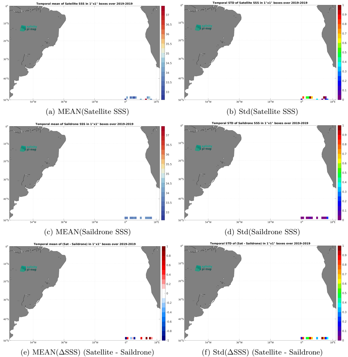
Figure 7: Temporal mean (left) and Std (right) of SSS from SMOS SSS L2Q v331 - No FLAG (CMEMS-CATDS-CPDC) (top), Saildrone (middle), and of \Delta SSS (Satellite - Saildrone). Only match-up pairs are used to generate these maps.
