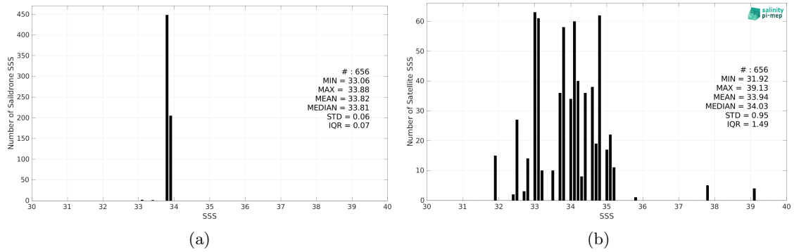
Figure 2: Histograms of SSS from Saïdrone (a) and SMOS SSS L2Q v331 - No FLAG (CMEMS-CATDS-CPDC) (b) considering all match-up pairs per bins of 0.1 over the South Atlantic Ocean Pi-MEP region and for the full satellite product period.
