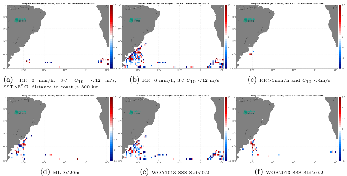
Figure 12: Temporal mean gridded over spatial boxes of size 1^{\circ}\times 1^{\circ} of \Delta\text{SSS} (SMOS SSS L2Q v331 - No FLAG (CMEMS-CATDS-CPDC) - Marine mammals) for 6 different subdatasets corresponding to:RR=0 mm/h, 3 < U_{10} < 12 m/s, SST >5^{\circ}\text{C} , distance to coast > 800 km (a), RR=0 mm/h, 3 < U_{10} < 12 m/s (b), RR >1 mm/h and U_{10} < 4 m/s (c),MLD <20 m (d),WOA2013 SSS Std <0.2 (e),WOA2013 SSS Std >0.2 (f).
