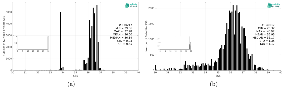
Figure 3: Histograms of SSS from Surface drifters (a) and SMOS SSS L2Q v331 - No FLAG (CMEMS-CATDS-CPDC) (b) considering all match-up pairs per bins of 0.1 over the South Atlantic Ocean Pi-MEP region and for the full satellite product period.
