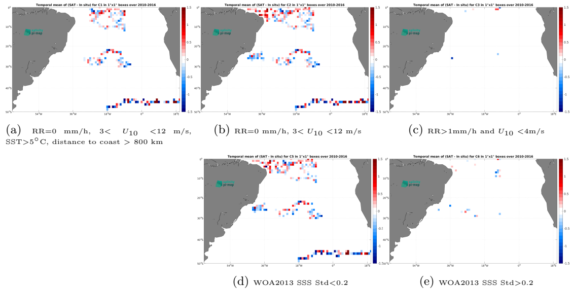
Figure 13: Temporal mean gridded over spatial boxes of size 1^\circ \times 1^\circ of \Delta SSS (SMOS SSS L2Q v331 - No FLAG (CMEMS-CATDS-CPDC) - Surface drifters) for 5 different subdatasets corresponding to:RR=0 mm/h, 3 < U_{10} < 12 m/s, SST >5^\circ\text{C} , distance to coast > 800 km (a), RR=0 mm/h, 3 < U_{10} < 12 m/s (b), RR >1 mm/h and U_{10} < 4 m/s (c), WOA2013 SSS Std <0.2 (d), WOA2013 SSS Std >0.2 (e).
