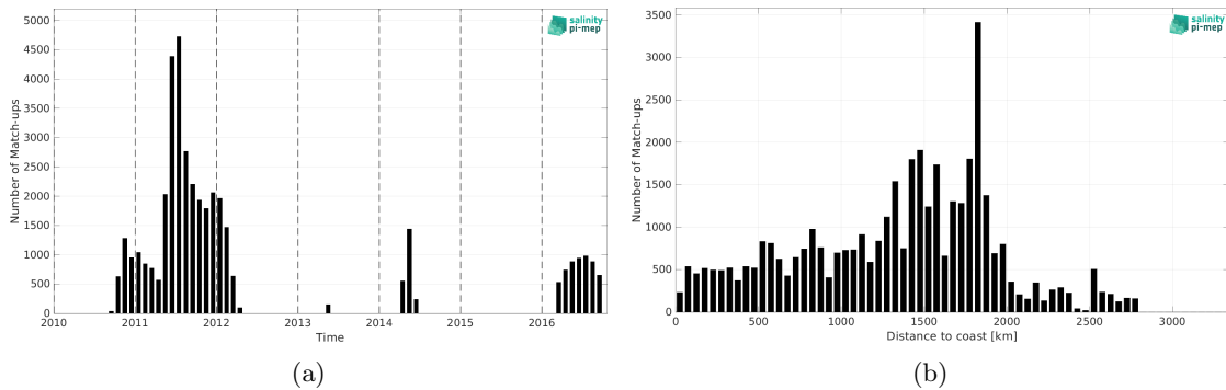
Figure 2: Number of match-ups between Surface drifters and SMOS SSS L2Q v331 - No FLAG (CMEMS-CATDS-CPDC) SSS as a function of time (a) and as function of the distance to coast (b) over the South Atlantic Ocean Pi-MEP region and for the full satellite product period.
