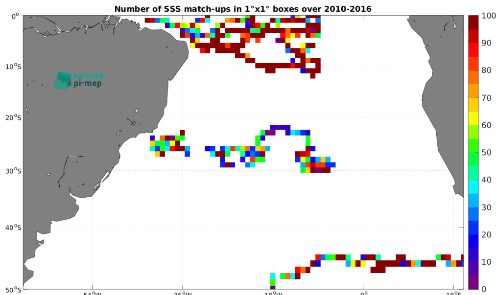
Figure 4: Number of SSS match-ups between Surface drifters SSS and the SMOS SSS L2Q v331 - No FLAG (CMEMS-CATDS-CPDC) SSS product for the South Atlantic Ocean Pi-MEP region over 1^\circ \times 1^\circ boxes and for the full satellite product period.
