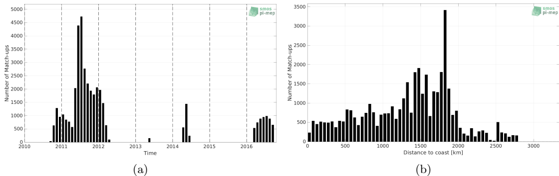
Figure 1: Number of match-ups between Surface drifters and SMOS SSS L2Q v331 - No FLAG (CMEMS-CATDS-CPDC) SSS as a function of time (a) and as function of the distance to coast (b) over the South Atlantic Ocean Pi-MEP region and for the full satellite product period.
