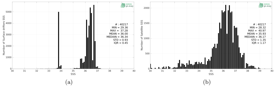
Figure 2: Histograms of SSS from Surface drifters (a) and SMOS SSS L2Q v331 - No FLAG (CMEMS-CATDS-CPDC) (b) considering all match-up pairs per bins of 0.1 over the South Atlantic Ocean Pi-MEP region and for the full satellite product period.
