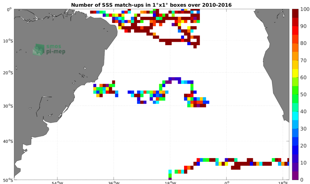
Figure 3: Number of SSS match-ups between Surface drifters SSS and the SMOS SSS L2Q v331 - No FLAG (CMEMS-CATDS-CPDC) SSS product for the South Atlantic Ocean Pi-MEP region over 1^\circ \times 1^\circ boxes and for the full satellite product period.
