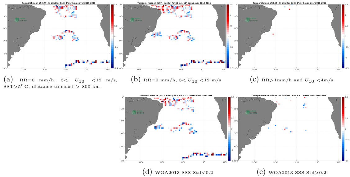
Figure 11: Temporal mean gridded over spatial boxes of size 1^\circ \times 1^\circ of \Delta\text{SSS} (SMOS SSS L2Q v331 - No FLAG (CMEMS-CATDS-CPDC) - Surface drifters) for 5 different subdatasets corresponding to:RR=0 mm/h, 3 < U_{10} < 12 m/s, SST >5^\circ\text{C} , distance to coast > 800 km (a), RR=0 mm/h, 3 < U_{10} < 12 m/s (b), RR >1 mm/h and U_{10} < 4 m/s (c), WOA2013 SSS Std <0.2 (d), WOA2013 SSS Std >0.2 (e).
