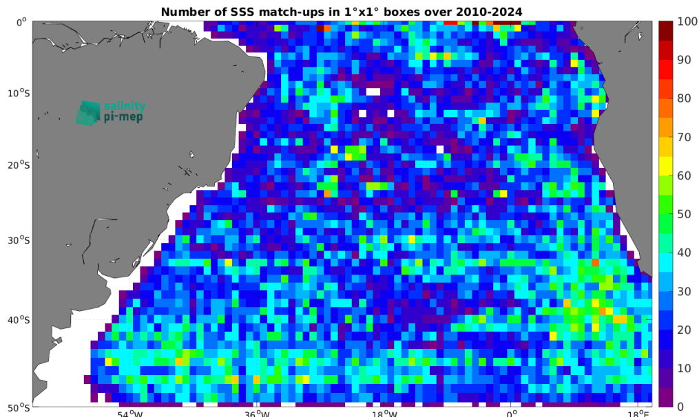
Figure 5: Number of SSS match-ups between Argo SSS and the SMOS SSS L2Q v331 - No FLAG (CMEMS-CATDS-CPDC) SSS product for the South Atlantic Ocean Pi-MEP region over 1^\circ \times 1^\circ boxes and for the full satellite product period.
