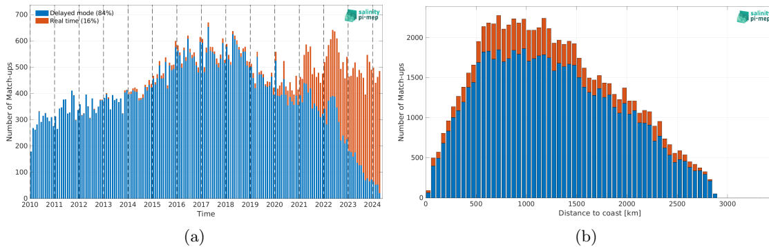
Figure 2: Number of match-ups between Argo and SMOS SSS L2Q v331 - No FLAG (CMEMS-CATDS-CPDC) SSS as a function of time (a) and as function of the distance to coast (b) over the South Atlantic Ocean Pi-MEP region and for the full satellite product period.
