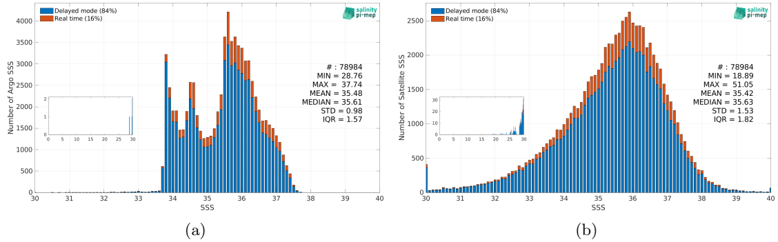
Figure 3: Histograms of SSS from Argo (a) and SMOS SSS L2Q v331 - No FLAG (CMEMS-CATDS-CPDC) (b) considering all match-up pairs per bins of 0.1 over the South Atlantic Ocean Pi-MEP region and for the full satellite product period.
