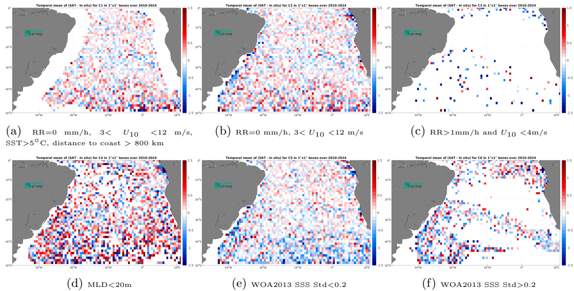
Figure 14: Temporal mean gridded over spatial boxes of size 1^\circ \times 1^\circ of \Delta SSS (SMOS SSS L2Q v331 - No FLAG (CMEMS-CATDS-CPDC) - Argo) for 6 different subdatasets corresponding to: RR=0 mm/h, 3 < U_{10} < 12 m/s, SST > 5°C, distance to coast > 800 km (a), RR=0 mm/h, 3 < U_{10} < 12 m/s (b), RR > 1mm/h and U_{10} < 4 m/s (c), MLD < 20m (d), WOA2013 SSS Std < 0.2 (e), WOA2013 SSS Std > 0.2 (f).
