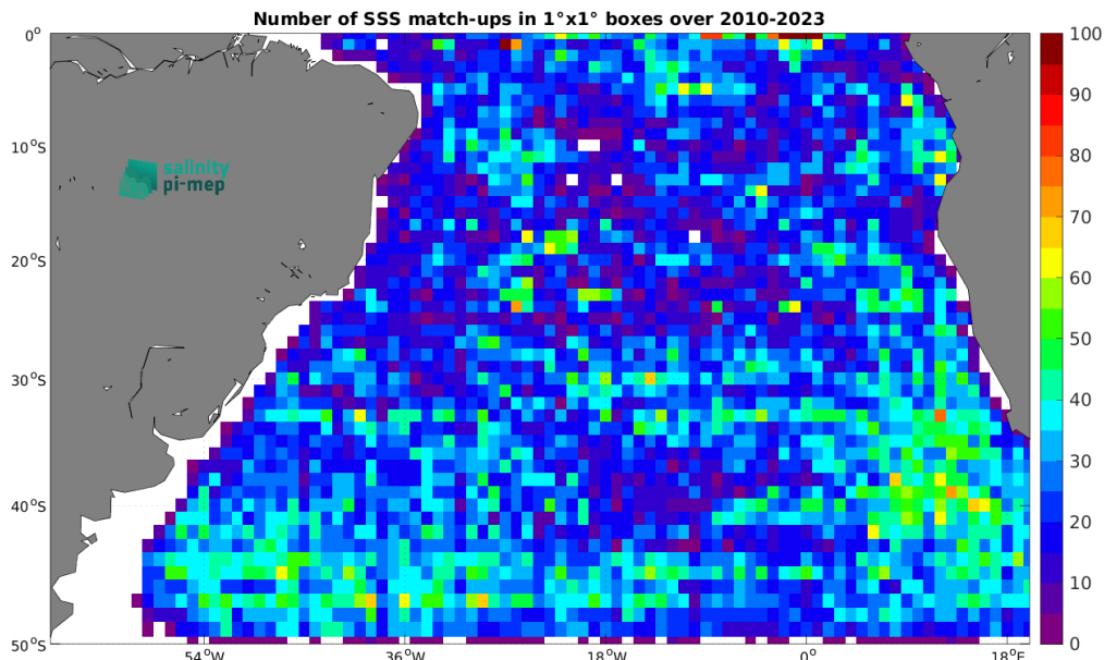
Figure 4: Number of SSS match-ups between Argo SSS and the SMOS SSS L2Q v331 - No FLAG (CMEMS-CATDS-CPDC) SSS product for the South Atlantic Ocean Pi-MEP region over 1^\circ \times 1^\circ boxes and for the full satellite product period.
