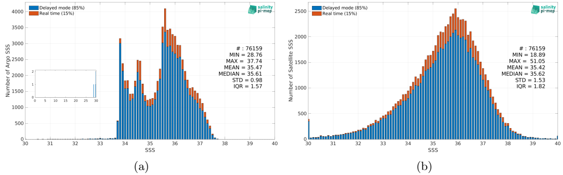
Figure 2: Histograms of SSS from Argo (a) and SMOS SSS L2Q v331 - No FLAG (CMEMS-CATDS-CPDC) (b) considering all match-up pairs per bins of 0.1 over the South Atlantic Ocean Pi-MEP region and for the full satellite product period.
