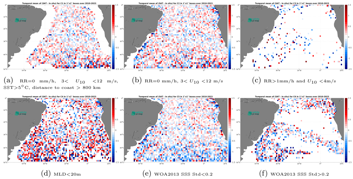
Figure 12: Temporal mean gridded over spatial boxes of size 1^\circ \times 1^\circ of \Delta SSS (SMOS SSS L2Q v331 - No FLAG (CMEMS-CATDS-CPDC) - Argo) for 6 different subdatasets corresponding to:RR=0 mm/h, 3 < U_{10} < 12 m/s, SST > 5^\circ\text{C} , distance to coast > 800 km (a), RR=0 mm/h, 3 < U_{10} < 12 m/s (b), RR > 1 mm/h and U_{10} < 4 m/s (c),MLD < 20 m (d),WOA2013 SSS Std < 0.2 (e),WOA2013 SSS Std > 0.2 (f).
