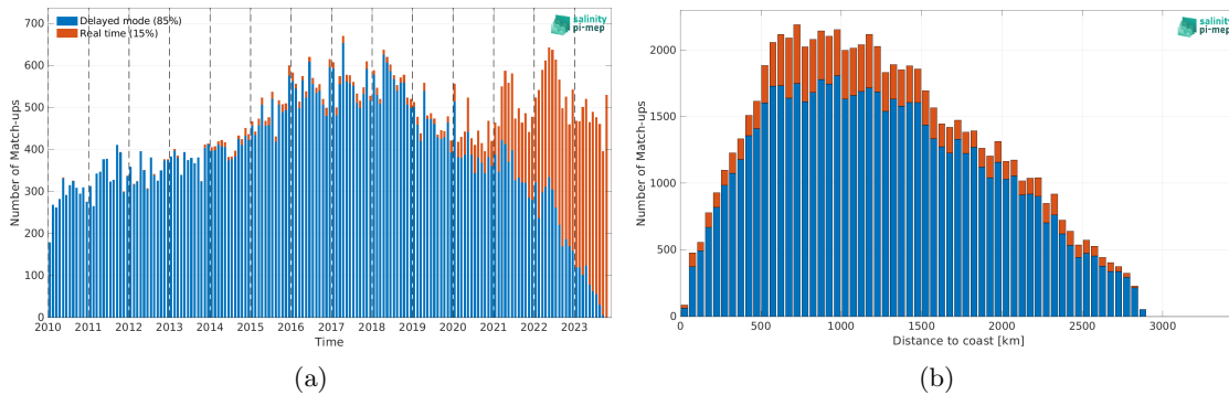
Figure 1: Number of match-ups between Argo and SMOS SSS L2Q v331 - No FLAG (CMEMS-CATDS-CPDC) SSS as a function of time (a) and as function of the distance to coast (b) over the South Atlantic Ocean Pi-MEP region and for the full satellite product period.
