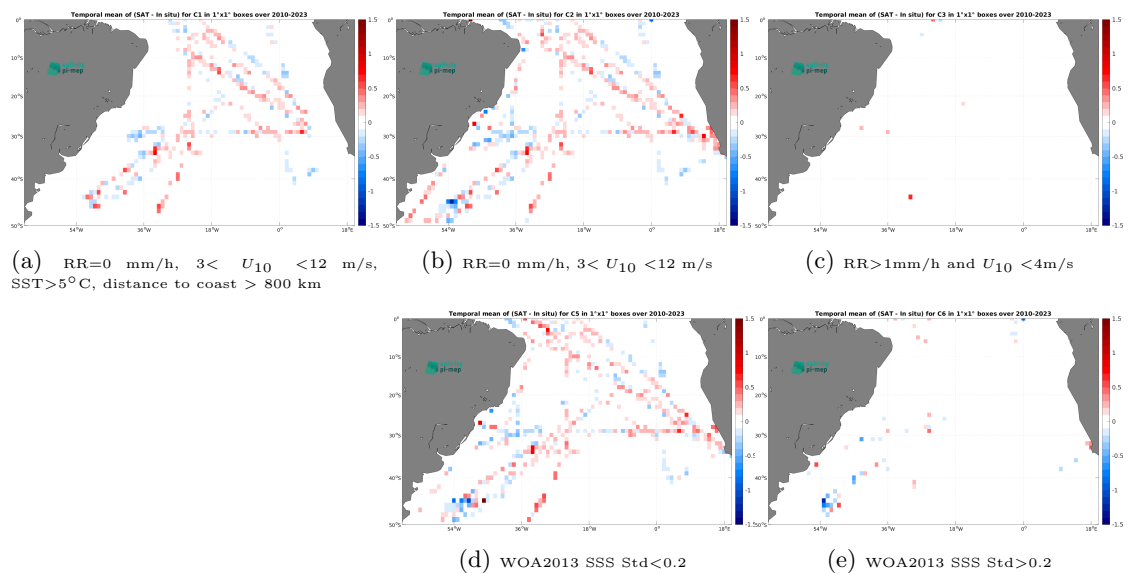
Figure 14: Temporal mean gridded over spatial boxes of size 1^\circ \times 1^\circ of \Delta SSS (SMOS SSS L3 v9 - 9 Days (CATDS-CEC-LOCEAN) - TSG (SAMOS)) for 5 different subdatasets corresponding to:RR=0 mm/h, 3 < U_{10} < 12 m/s, SST >5^\circ\text{C} , distance to coast > 800 km (a), RR=0 mm/h, 3 < U_{10} < 12 m/s (b), RR >1 mm/h and U_{10} < 4 m/s (c), WOA2013 SSS Std <0.2 (d), WOA2013 SSS Std >0.2 (e).
