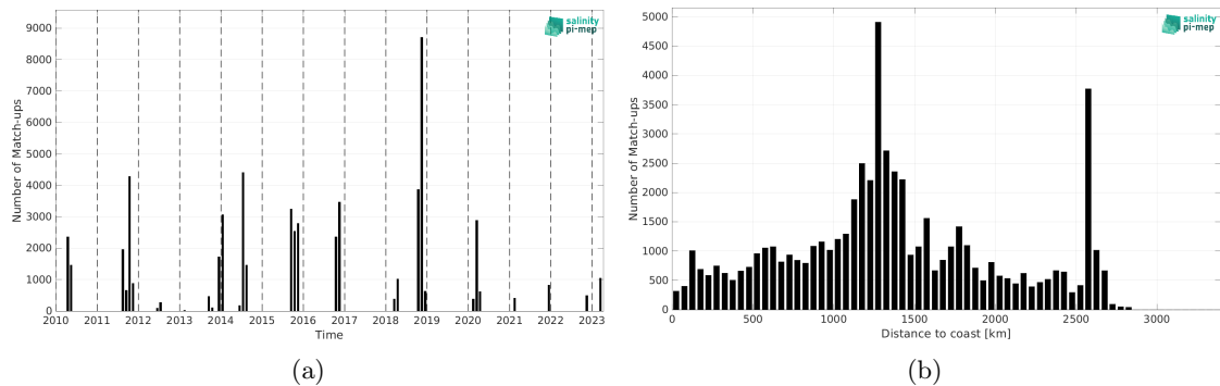
Figure 2: Number of match-ups between TSG (SAMOS) and SMOS SSS L3 v9 - 9 Days (CATDS-CEC-LOCEAN) SSS as a function of time (a) and as function of the distance to coast (b) over the South Atlantic Ocean Pi-MEP region and for the full satellite product period.
