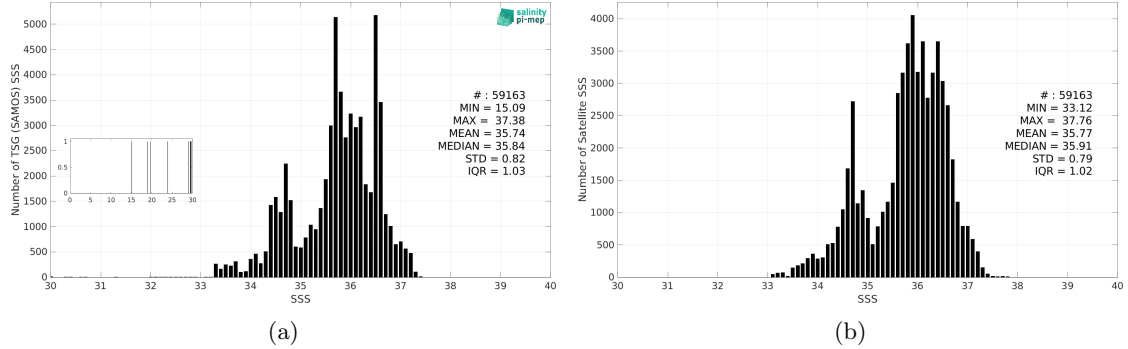
Figure 2: Histograms of SSS from TSG (SAMOS) (a) and SMOS SSS L3 v9 - 9 Days (CATDS-CEC-LOCEAN) (b) considering all match-up pairs per bins of 0.1 over the South Atlantic Ocean Pi-MEP region and for the full satellite product period.
