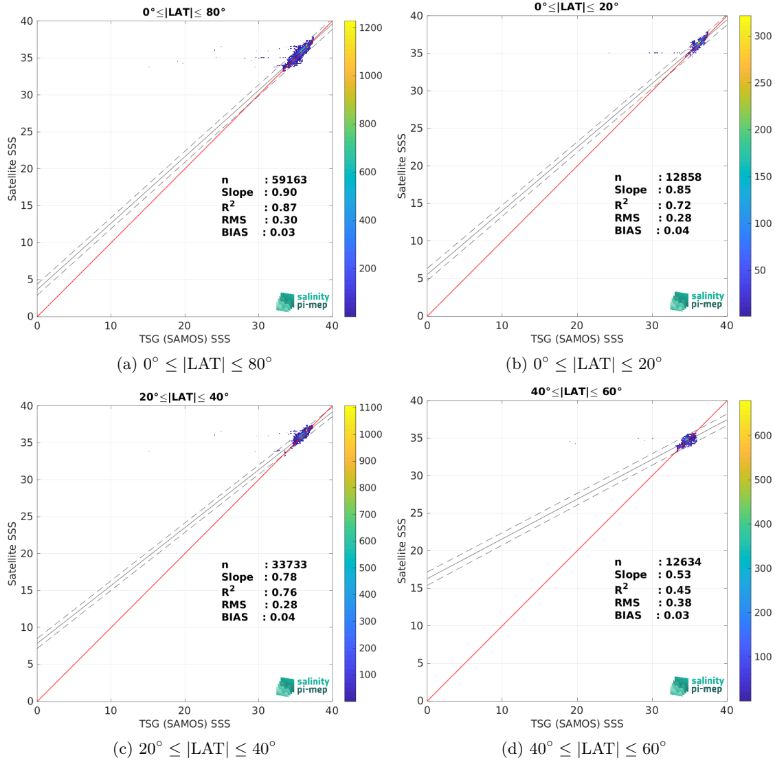
Figure 9: Contour maps of the concentration of SMOS SSS L3 v9 - 9 Days (CATDS-CEC-LOCEAN) SSS (y-axis) versus TSG (SAMOS) SSS (x-axis) at match-up pairs for different latitude bands. For each plot, the red line shows x=y . The black thin and dashed lines indicate a linear fit through the data cloud and the \pm 95\% confidence levels, respectively. The number match-up pairs n , the slope and R^2 coefficient of the linear fit, the root mean square (RMS) and the mean bias between satellite and in situ data are indicated for each latitude band in each plots.
