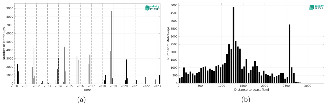
Figure 1: Number of match-ups between TSG (SAMOS) and SMOS SSS L3 v9 - 9 Days (CATDS-CEC-LOCEAN) SSS as a function of time (a) and as function of the distance to coast (b) over the South Atlantic Ocean Pi-MEP region and for the full satellite product period.
