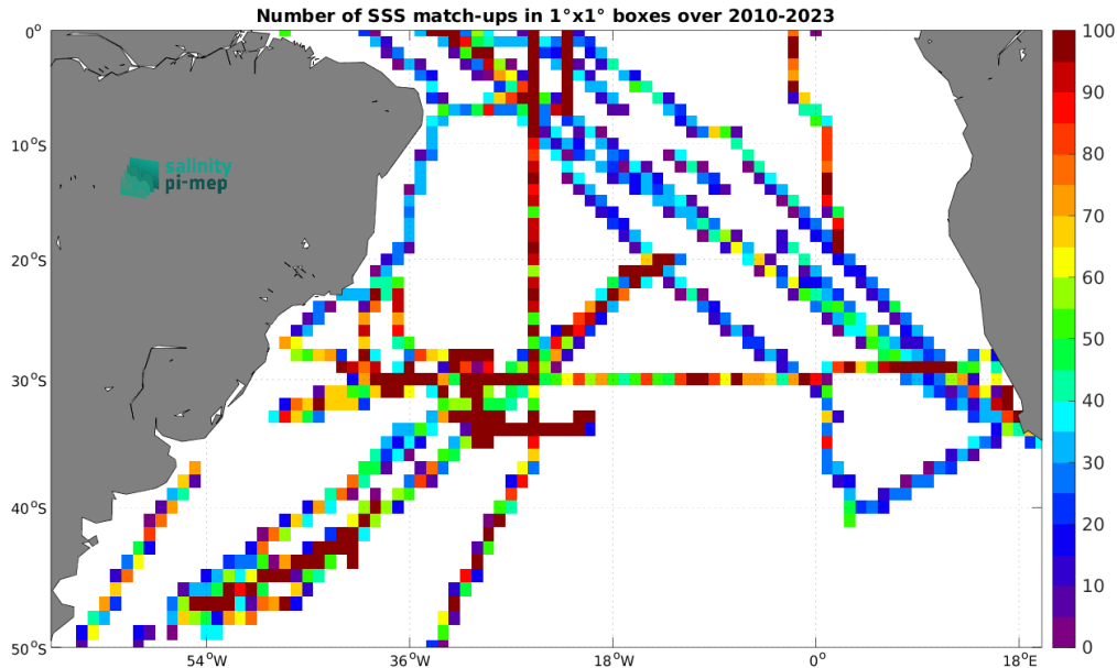
Figure 4: Number of SSS match-ups between TSG (SAMOS) SSS and the SMOS SSS L3 v9 - 9 Days (CATDS-CEC-LOCEAN) SSS product for the South Atlantic Ocean Pi-MEP region over 1^\circ \times 1^\circ boxes and for the full satellite product period.
