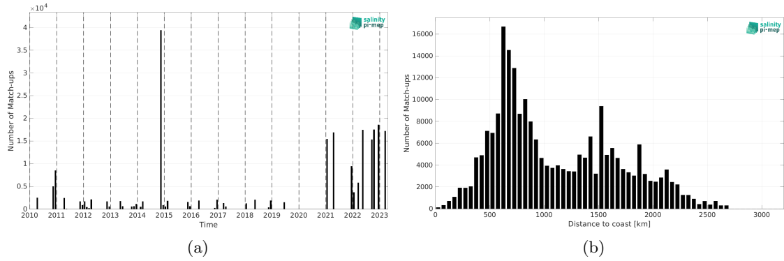
Figure 2: Number of match-ups between TSG (Polarstern) and SMOS SSS L3 v9 - 9 Days (CATDS-CEC-LOCEAN) SSS as a function of time (a) and as function of the distance to coast (b) over the South Atlantic Ocean Pi-MEP region and for the full satellite product period.
