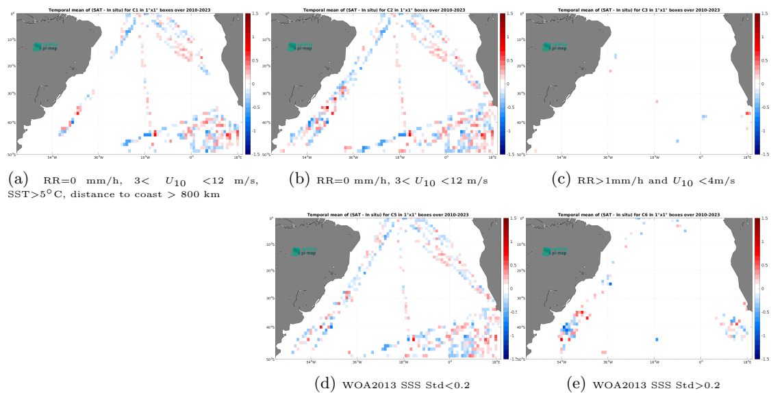
Figure 14: Temporal mean gridded over spatial boxes of size 1^\circ \times 1^\circ of \Delta\text{SSS} (SMOS SSS L3 v9 - 9 Days (CATDS-CEC-LOCEAN) - TSG (Polarstern)) for 5 different subdatasets corresponding to:RR=0 mm/h, 3 < U_{10} < 12 m/s, SST >5^\circ\text{C} , distance to coast > 800 km (a), RR=0 mm/h, 3 < U_{10} < 12 m/s (b), RR >1 mm/h and U_{10} < 4 m/s (c), WOA2013 SSS Std <0.2 (d), WOA2013 SSS Std >0.2 (e).
