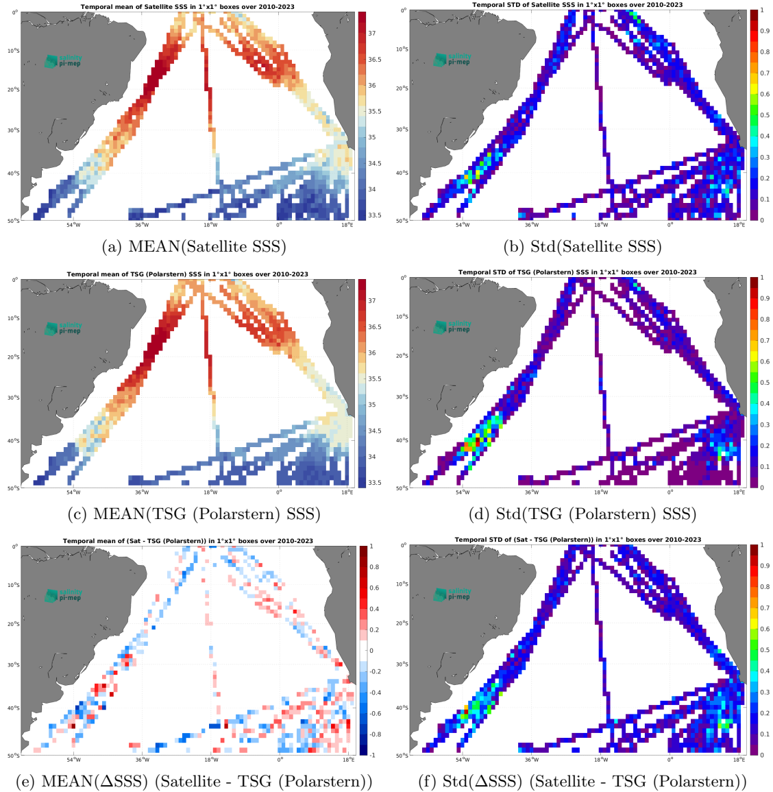
Figure 7: Temporal mean (left) and Std (right) of SSS from SMOS SSS L3 v9 - 9 Days (CATDS-CEC-LOCEAN) (top), TSG (Polarstern) (middle), and of \Delta SSS (Satellite - TSG (Polarstern)). Only match-up pairs are used to generate these maps.
