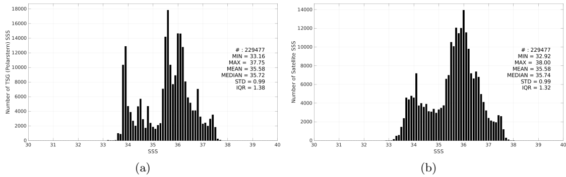
Figure 3: Histograms of SSS from TSG (Polarstern) (a) and SMOS SSS L3 v9 - 9 Days (CATDS-CEC-LOCEAN) (b) considering all match-up pairs per bins of 0.1 over the South Atlantic Ocean Pi-MEP region and for the full satellite product period.
