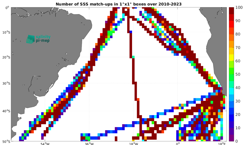
Figure 5: Number of SSS match-ups between TSG (Polarstern) SSS and the SMOS SSS L3 v9 - 9 Days (CATDS-CEC-LOCEAN) SSS product for the South Atlantic Ocean Pi-MEP region over 1^\circ \times 1^\circ boxes and for the full satellite product period.
