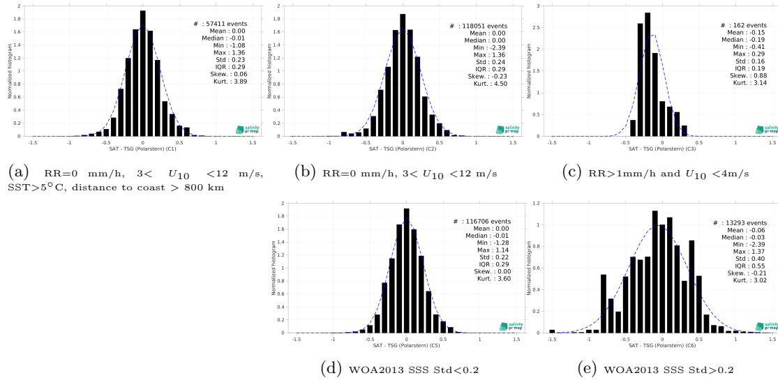
Figure 13: Normalized histogram of \Delta SSS (SMOS SSS L3 v9 - 9 Days (CATDS-CEC-LOCEAN) - TSG (Polarstern)) for 5 different subdatasets corresponding to: RR=0 mm/h, 3 < U_{10} < 12 m/s, SST>5°C, distance to coast > 800 km (a), RR=0 mm/h, 3 < U_{10} < 12 m/s (b), RR>1mm/h and U_{10} < 4 m/s (c), WOA2013 SSS Std<0.2 (d), WOA2013 SSS Std>0.2 (e).
