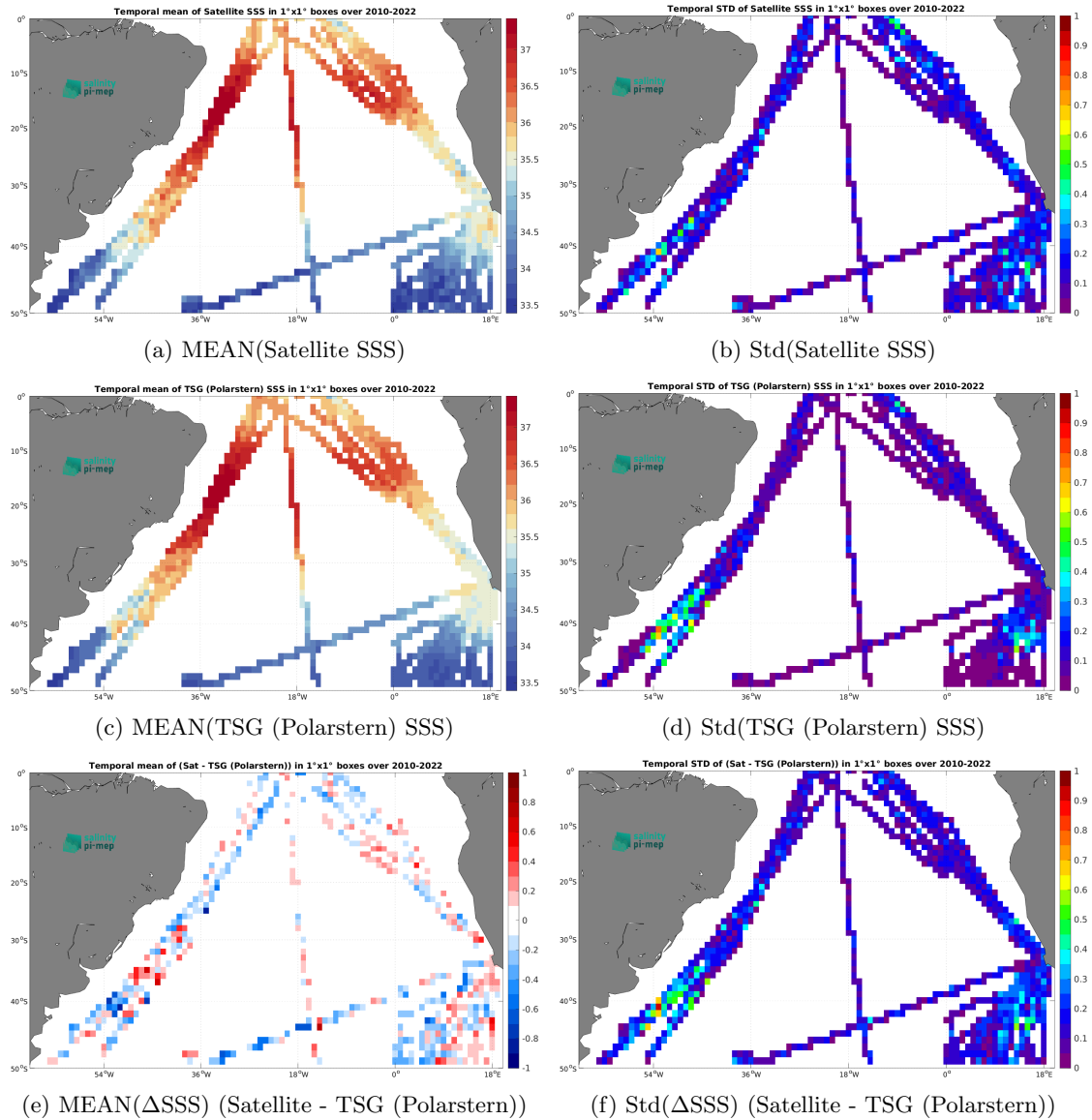
Figure 6: Temporal mean (left) and Std (right) of SSS from SMOS SSS L3 v9 - 9 Days (CATDS-CEC-LOCEAN) (top), TSG (Polarstern) (middle), and of \Delta SSS (Satellite - TSG (Polarstern)). Only match-up pairs are used to generate these maps.
