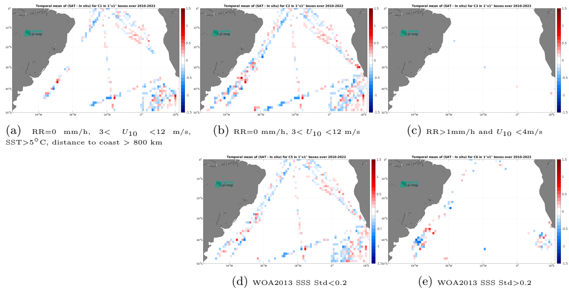
Figure 12: Temporal mean gridded over spatial boxes of size 1^\circ \times 1^\circ of \Delta SSS (SMOS SSS L3 v9 - 9 Days (CATDS-CEC-LOCEAN) - TSG (Polarstern)) for 5 different subdatasets corresponding to:RR=0 mm/h, 3 < U_{10} < 12 m/s, SST >5^\circ C, distance to coast > 800 km (a), RR=0 mm/h, 3 < U_{10} < 12 m/s (b), RR >1 mm/h and U_{10} < 4 m/s (c), WOA2013 SSS Std <0.2 (d), WOA2013 SSS Std >0.2 (e).
