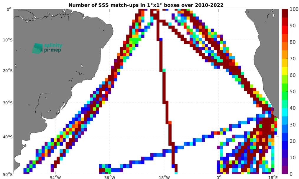
Figure 4: Number of SSS match-ups between TSG (Polarstern) SSS and the SMOS SSS L3 v9 - 9 Days (CATDS-CEC-LOCEAN) SSS product for the South Atlantic Ocean Pi-MEP region over 1^\circ \times 1^\circ boxes and for the full satellite product period.
