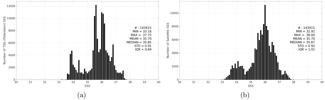
Figure 2: Histograms of SSS from TSG (Polarstern) (a) and SMOS SSS L3 v9 - 9 Days (CATDS-CEC-LOCEAN) (b) considering all match-up pairs per bins of 0.1 over the South Atlantic Ocean Pi-MEP region and for the full satellite product period.
