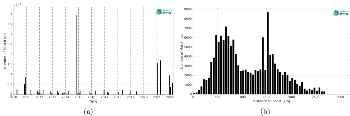
Figure 1: Number of match-ups between TSG (Polarstern) and SMOS SSS L3 v9 - 9 Days (CATDS-CEC-LOCEAN) SSS as a function of time (a) and as function of the distance to coast (b) over the South Atlantic Ocean Pi-MEP region and for the full satellite product period.
