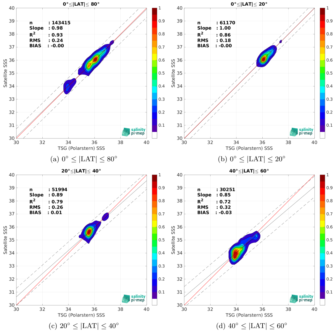
Figure 9: Contour maps of the concentration of SMOS SSS L3 v9 - 9 Days (CATDS-CEC-LOCEAN) SSS (y-axis) versus TSG (Polarstern) SSS (x-axis) at match-up pairs for different latitude bands. For each plot, the red line shows x=y . The black thin and dashed lines indicate a linear fit through the data cloud and the \pm 95\% confidence levels, respectively. The number match-up pairs n , the slope and R^2 coefficient of the linear fit, the root mean square (RMS) and the mean bias between satellite and in situ data are indicated for each latitude band in each plots.
