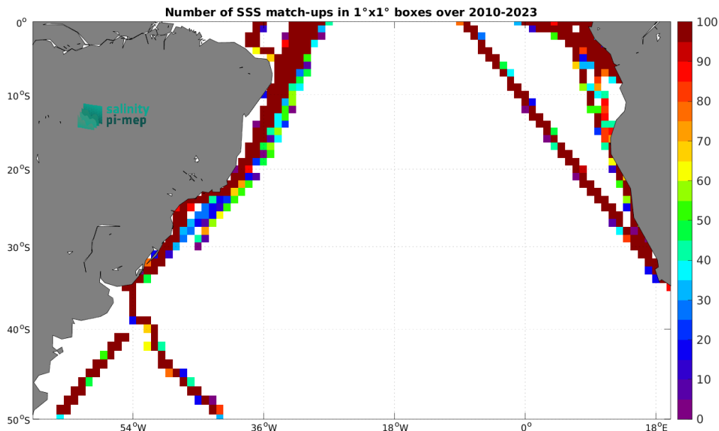
Figure 5: Number of SSS match-ups between TSG (LEGOS-DM) SSS and the SMOS SSS L3 v9 - 9 Days (CATDS-CEC-LOCEAN) SSS product for the South Atlantic Ocean Pi-MEP region over 1^\circ \times 1^\circ boxes and for the full satellite product period.
