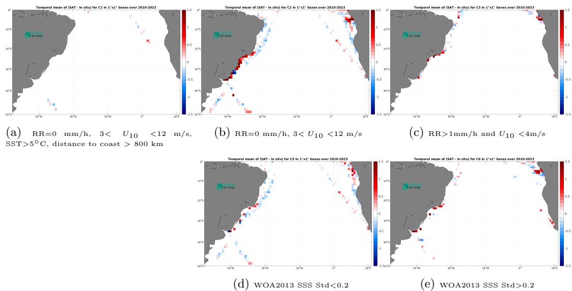
Figure 14: Temporal mean gridded over spatial boxes of size 1^\circ \times 1^\circ of \Delta\text{SSS} (SMOS SSS L3 v9 - 9 Days (CATDS-CEC-LOCEAN) - TSG (LEGOS-DM)) for 5 different subdatasets corresponding to:RR=0 mm/h, 3 < U_{10} < 12 m/s, SST >5^\circ\text{C} , distance to coast > 800 km (a), RR=0 mm/h, 3 < U_{10} < 12 m/s (b), RR >1 mm/h and U_{10} < 4 m/s (c), WOA2013 SSS Std <0.2 (d), WOA2013 SSS Std >0.2 (e).
