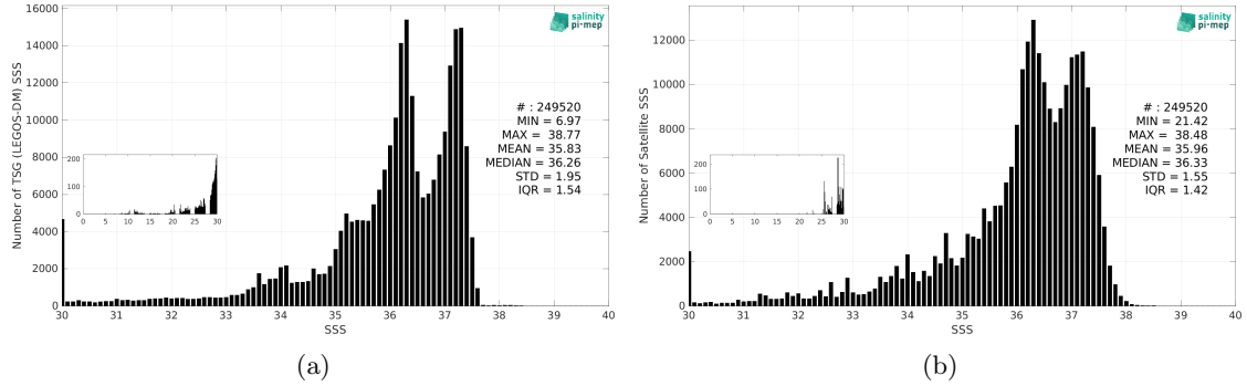
Figure 3: Histograms of SSS from TSG (LEGOS-DM) (a) and SMOS SSS L3 v9 - 9 Days (CATDS-CEC-LOCEAN) (b) considering all match-up pairs per bins of 0.1 over the South Atlantic Ocean Pi-MEP region and for the full satellite product period.
