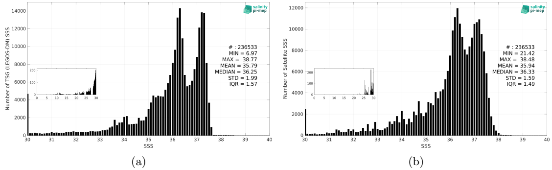
Figure 3: Histograms of SSS from TSG (LEGOS-DM) (a) and SMOS SSS L3 v9 - 9 Days (CATDS-CEC-LOCEAN) (b) considering all match-up pairs per bins of 0.1 over the South Atlantic Ocean Pi-MEP region and for the full satellite product period.
