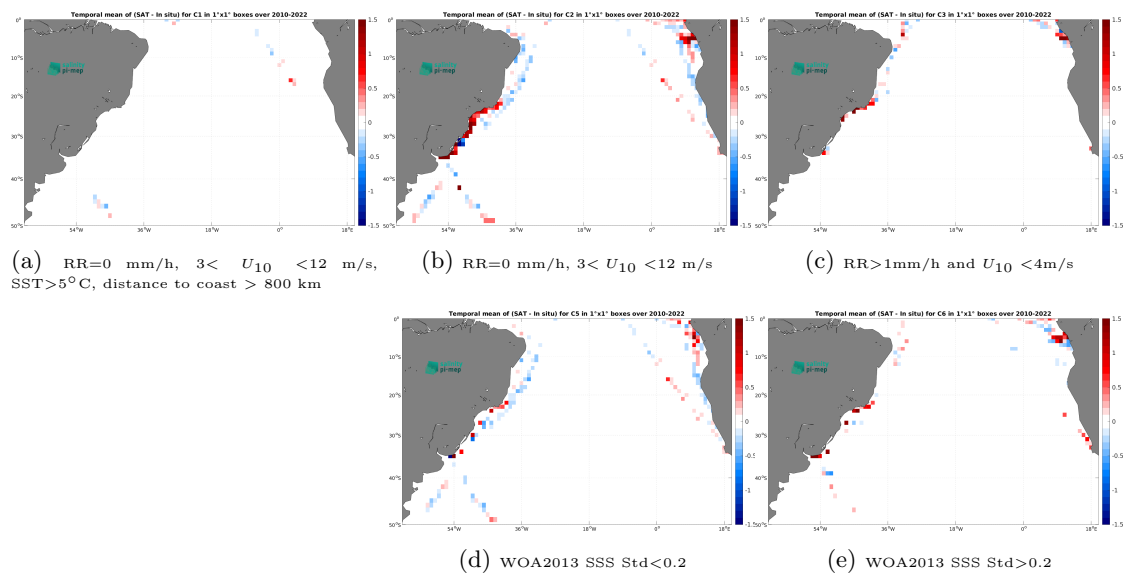
Figure 14: Temporal mean gridded over spatial boxes of size 1^\circ \times 1^\circ of \Delta SSS (SMOS SSS L3 v9 - 9 Days (CATDS-CEC-LOCEAN) - TSG (LEGOS-DM)) for 5 different subdatasets corresponding to:RR=0 mm/h, 3 < U_{10} < 12 m/s, SST>5°C, distance to coast > 800 km (a), RR=0 mm/h, 3 < U_{10} < 12 m/s (b), RR>1mm/h and U_{10} < 4 m/s (c), WOA2013 SSS Std<0.2 (d), WOA2013 SSS Std>0.2 (e).
