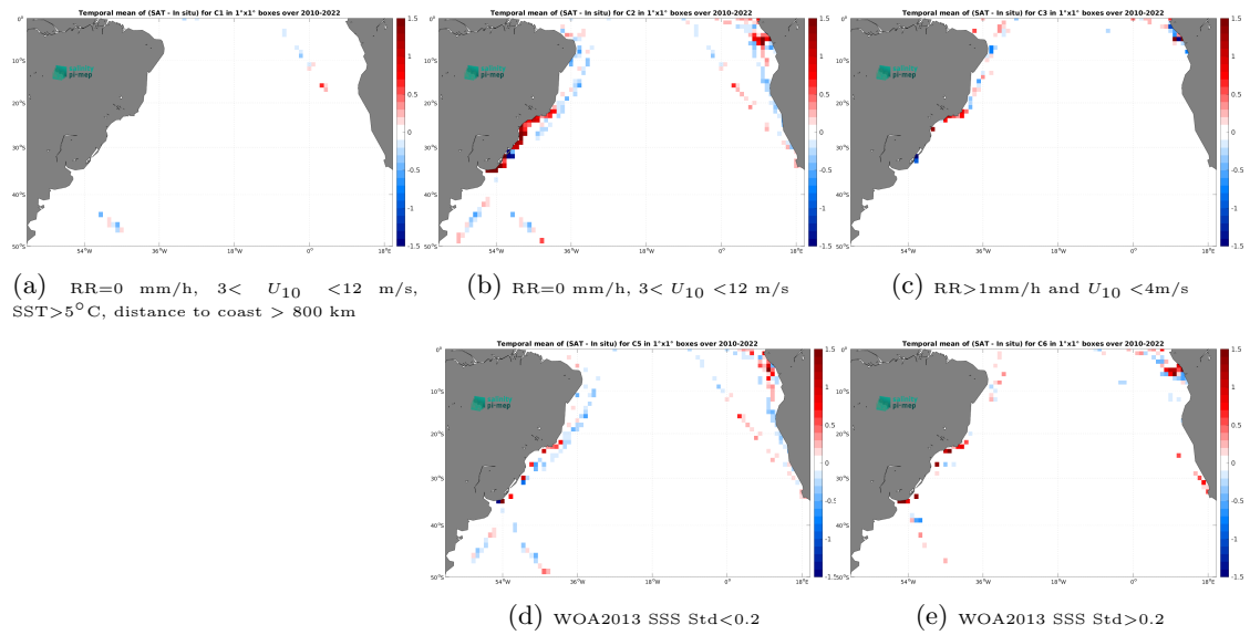
Figure 12: Temporal mean gridded over spatial boxes of size 1^\circ \times 1^\circ of \Delta SSS (SMOS SSS L3 v9 - 9 Days (CATDS-CEC-LOCEAN) - TSG (LEGOS-DM)) for 5 different subdatasets corresponding to:RR=0 mm/h, 3 < U_{10} < 12 m/s, SST >5^\circ C, distance to coast > 800 km (a), RR=0 mm/h, 3 < U_{10} < 12 m/s (b), RR >1 mm/h and U_{10} < 4 m/s (c), WOA2013 SSS Std <0.2 (d), WOA2013 SSS Std >0.2 (e).
