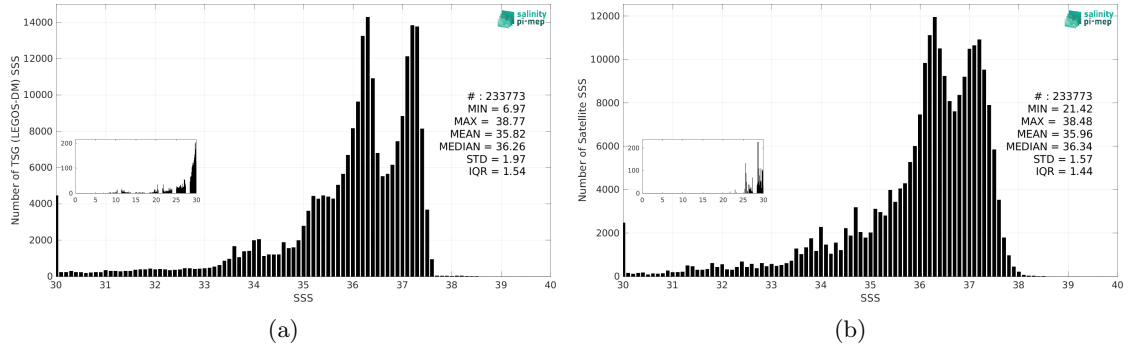
Figure 2: Histograms of SSS from TSG (LEGOS-DM) (a) and SMOS SSS L3 v9 - 9 Days (CATDS-CEC-LOCEAN) (b) considering all match-up pairs per bins of 0.1 over the South Atlantic Ocean Pi-MEP region and for the full satellite product period.
