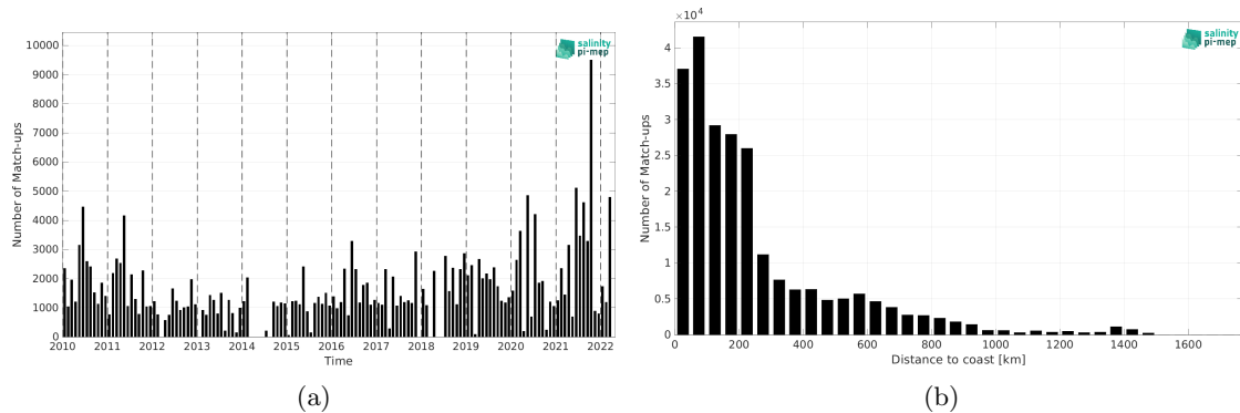
Figure 1: Number of match-ups between TSG (LEGOS-DM) and SMOS SSS L3 v9 - 9 Days (CATDS-CEC-LOCEAN) SSS as a function of time (a) and as function of the distance to coast (b) over the South Atlantic Ocean Pi-MEP region and for the full satellite product period.
