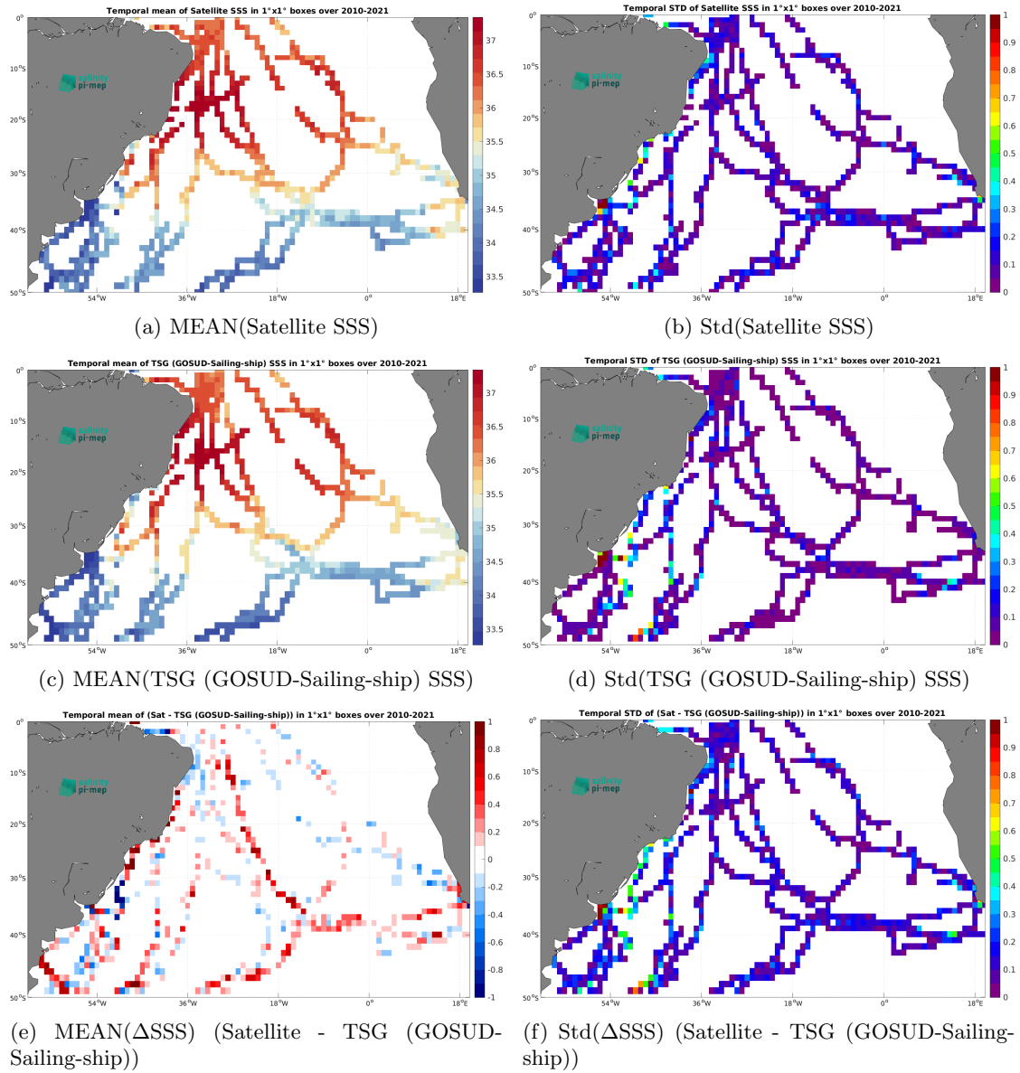
Figure 7: Temporal mean (left) and Std (right) of SSS from SMOS SSS L3 v9 - 9 Days (CATDS-CEC-LOCEAN) (top), TSG (GOSUD-Sailing-ship) (middle), and of \Delta SSS (Satellite - TSG (GOSUD-Sailing-ship)). Only match-up pairs are used to generate these maps.
