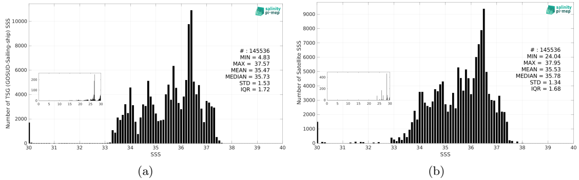
Figure 3: Histograms of SSS from TSG (GOSUD-Sailing-ship) (a) and SMOS SSS L3 v9 - 9 Days (CATDS-CEC-LOCEAN) (b) considering all match-up pairs per bins of 0.1 over the South Atlantic Ocean Pi-MEP region and for the full satellite product period.
