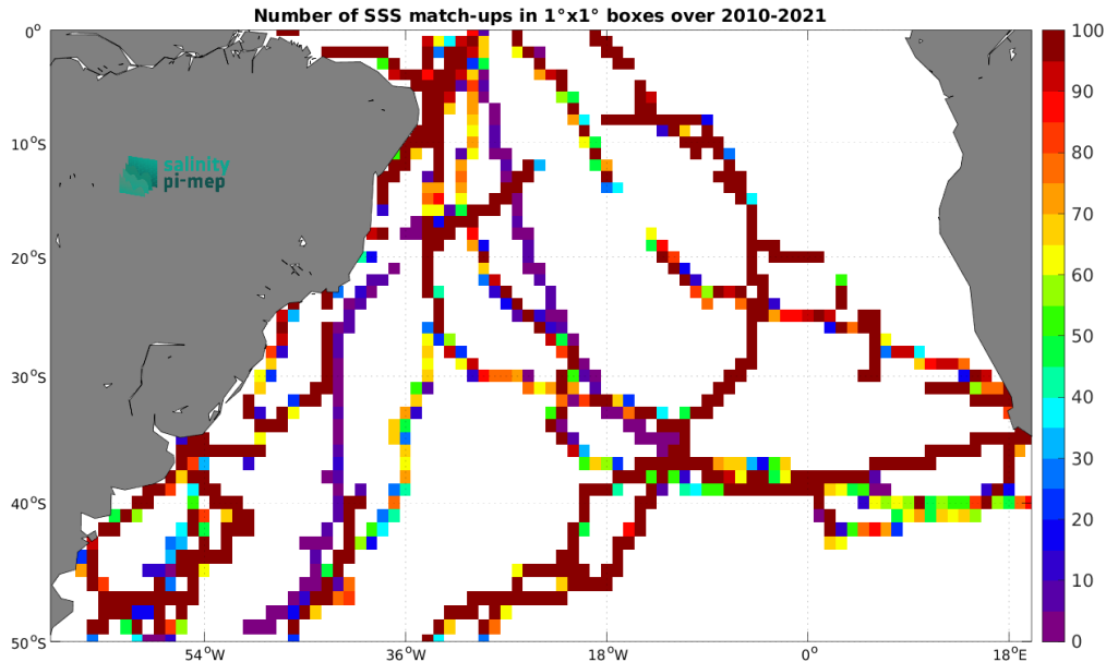
Figure 5: Number of SSS match-ups between TSG (GOSUD-Sailing-ship) SSS and the SMOS SSS L3 v9 - 9 Days (CATDS-CEC-LOCEAN) SSS product for the South Atlantic Ocean Pi-MEP region over 1^\circ \times 1^\circ boxes and for the full satellite product period.
