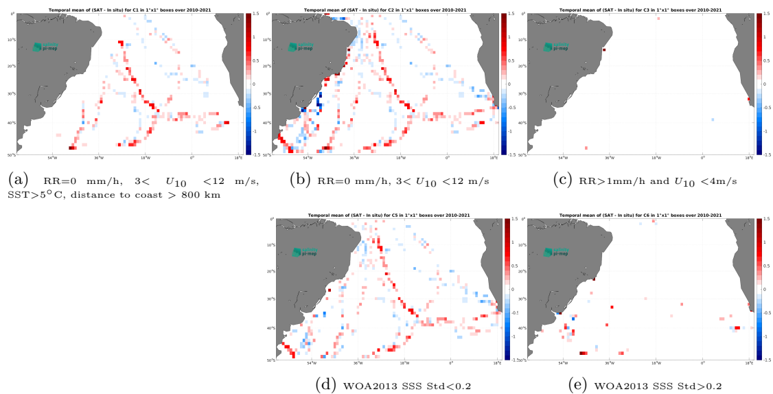
Figure 14: Temporal mean gridded over spatial boxes of size 1^\circ \times 1^\circ of \Delta SSS (SMOS SSS L3 v9 - 9 Days (CATDS-CEC-LOCEAN) - TSG (GOSUD-Sailing-ship)) for 5 different subdatasets corresponding to:RR=0 mm/h, 3 < U_{10} < 12 m/s, SST >5^\circ\text{C} , distance to coast > 800 km (a), RR=0 mm/h, 3 < U_{10} < 12 m/s (b), RR >1 mm/h and U_{10} < 4 m/s (c), WOA2013 SSS Std <0.2 (d), WOA2013 SSS Std >0.2 (e).
