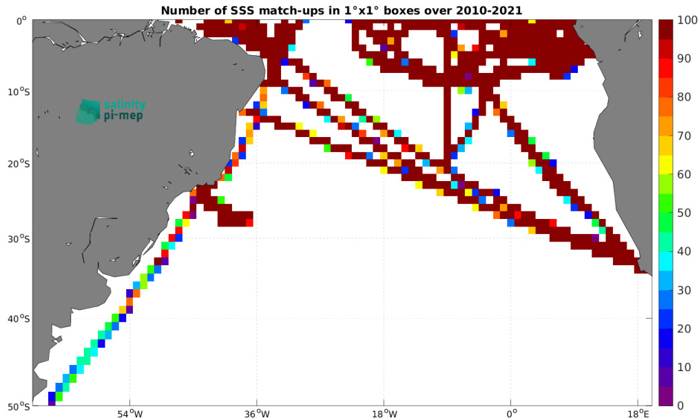
Figure 5: Number of SSS match-ups between TSG (GOSUD-Research-vessel) SSS and the SMOS SSS L3 v9 - 9 Days (CATDS-CEC-LOCEAN) SSS product for the South Atlantic Ocean Pi-MEP region over 1^\circ \times 1^\circ boxes and for the full satellite product period.
