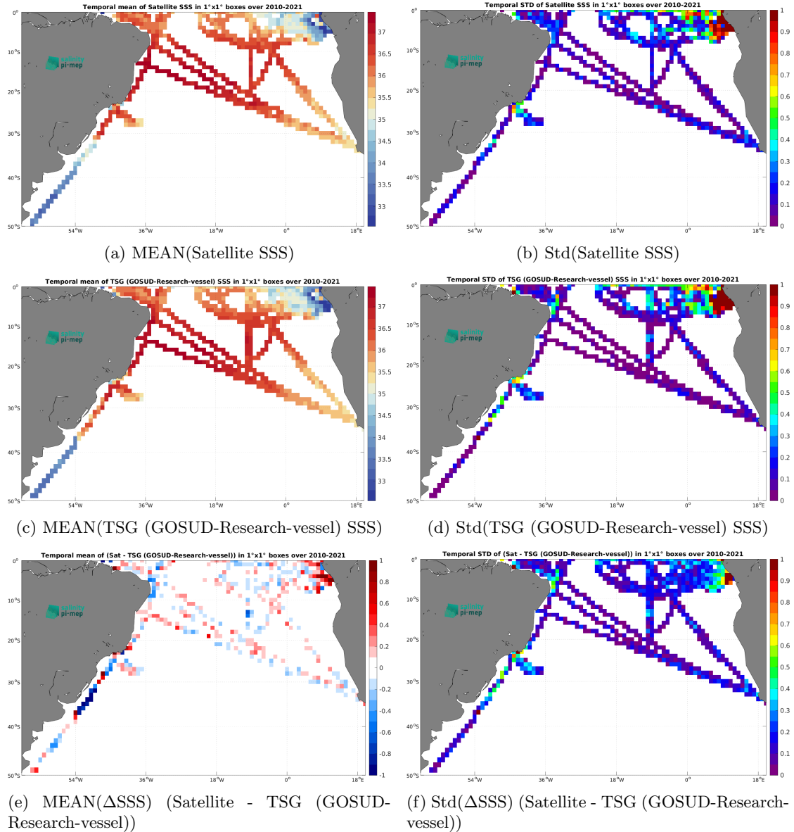
Figure 7: Temporal mean (left) and Std (right) of SSS from SMOS SSS L3 v9 - 9 Days (CATDS-CEC-LOCEAN) (top), TSG (GOSUD-Research-vessel) (middle), and of \Delta SSS (Satellite - TSG (GOSUD-Research-vessel)). Only match-up pairs are used to generate these maps.
