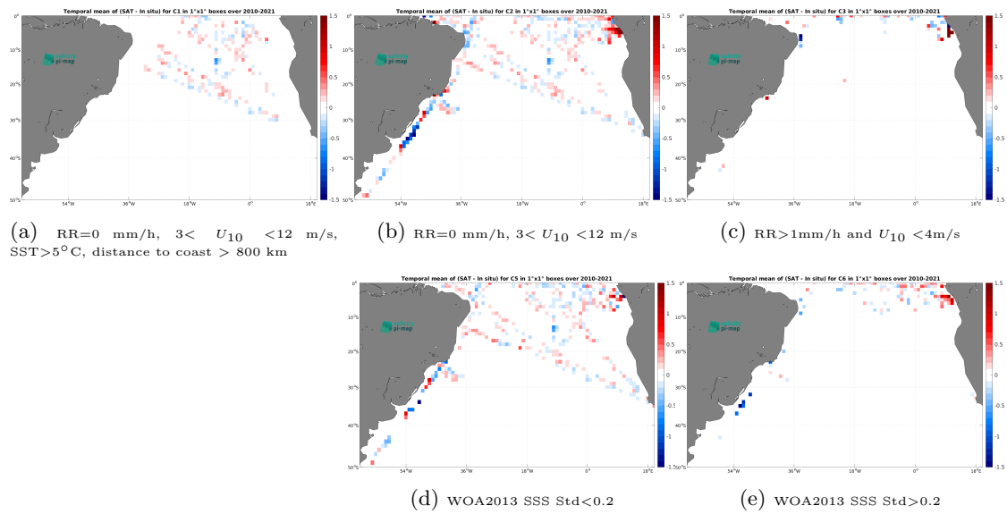
Figure 14: Temporal mean gridded over spatial boxes of size 1^\circ \times 1^\circ of \Delta SSS (SMOS SSS L3 v9 - 9 Days (CATDS-CEC-LOCEAN) - TSG (GOSUD-Research-vessel)) for 5 different subdatasets corresponding to:RR=0 mm/h, 3 < U_{10} < 12 m/s, SST >5^\circ\text{C} , distance to coast > 800 km (a), RR=0 mm/h, 3 < U_{10} < 12 m/s (b), RR >1 mm/h and U_{10} < 4 m/s (c), WOA2013 SSS Std <0.2 (d), WOA2013 SSS Std >0.2 (e).
