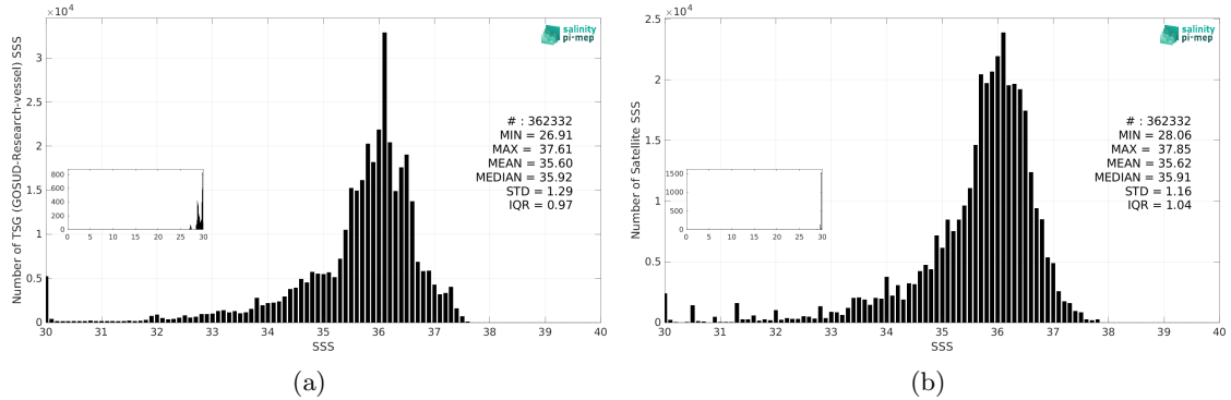
Figure 3: Histograms of SSS from TSG (GOSUD-Research-vessel) (a) and SMOS SSS L3 v9 - 9 Days (CATDS-CEC-LOCEAN) (b) considering all match-up pairs per bins of 0.1 over the South Atlantic Ocean Pi-MEP region and for the full satellite product period.
