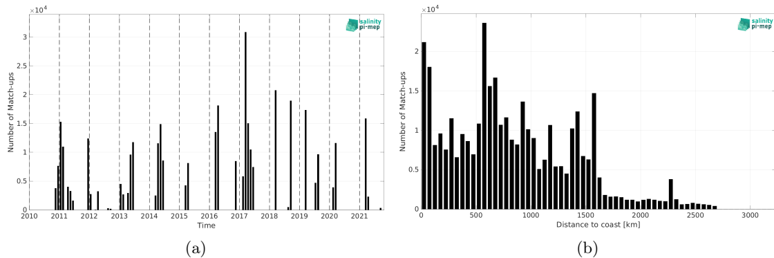
Figure 1: Number of match-ups between TSG (GOSUD-Research-vessel) and SMOS SSS L3 v9 - 9 Days (CATDS-CEC-LOCEAN) SSS as a function of time (a) and as function of the distance to coast (b) over the South Atlantic Ocean Pi-MEP region and for the full satellite product period.
