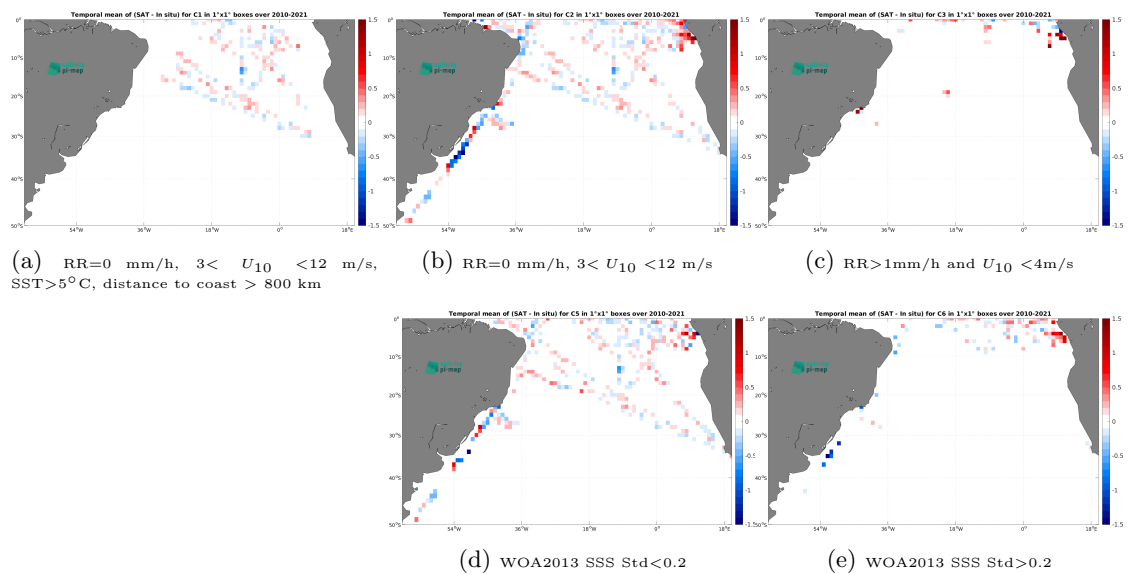
Figure 12: Temporal mean gridded over spatial boxes of size 1^\circ \times 1^\circ of \Delta SSS (SMOS SSS L3 v9 - 9 Days (CATDS-CEC-LOCEAN) - TSG (GOSUD-Research-vessel)) for 5 different subdatasets corresponding to:RR=0 mm/h, 3 < U_{10} < 12 m/s, SST>5°C, distance to coast > 800 km (a), RR=0 mm/h, 3 < U_{10} < 12 m/s (b), RR>1mm/h and U_{10} < 4 m/s (c), WOA2013 SSS Std<0.2 (d), WOA2013 SSS Std>0.2 (e).
