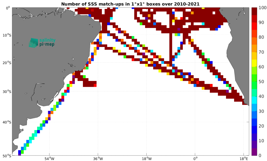
Figure 4: Number of SSS match-ups between TSG (GOSUD-Research-vessel) SSS and the SMOS SSS L3 v9 - 9 Days (CATDS-CEC-LOCEAN) SSS product for the South Atlantic Ocean Pi-MEP region over 1^\circ \times 1^\circ boxes and for the full satellite product period.
