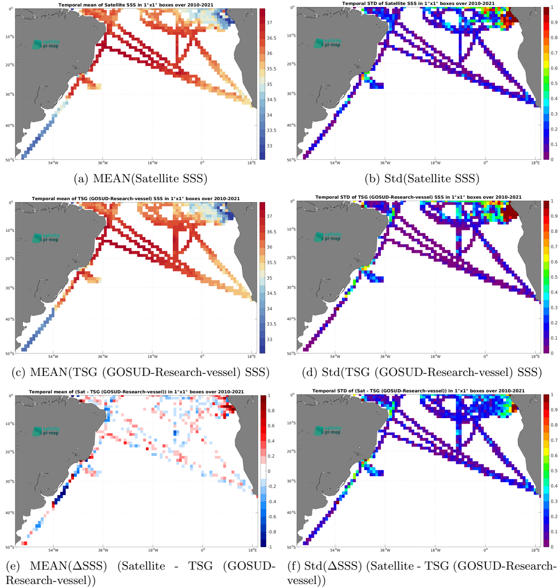
Figure 6: Temporal mean (left) and Std (right) of SSS from SMOS SSS L3 v9 - 9 Days (CATDS-CEC-LOCEAN) (top), TSG (GOSUD-Research-vessel) (middle), and of \Delta SSS (Satellite - TSG (GOSUD-Research-vessel)). Only match-up pairs are used to generate these maps.
