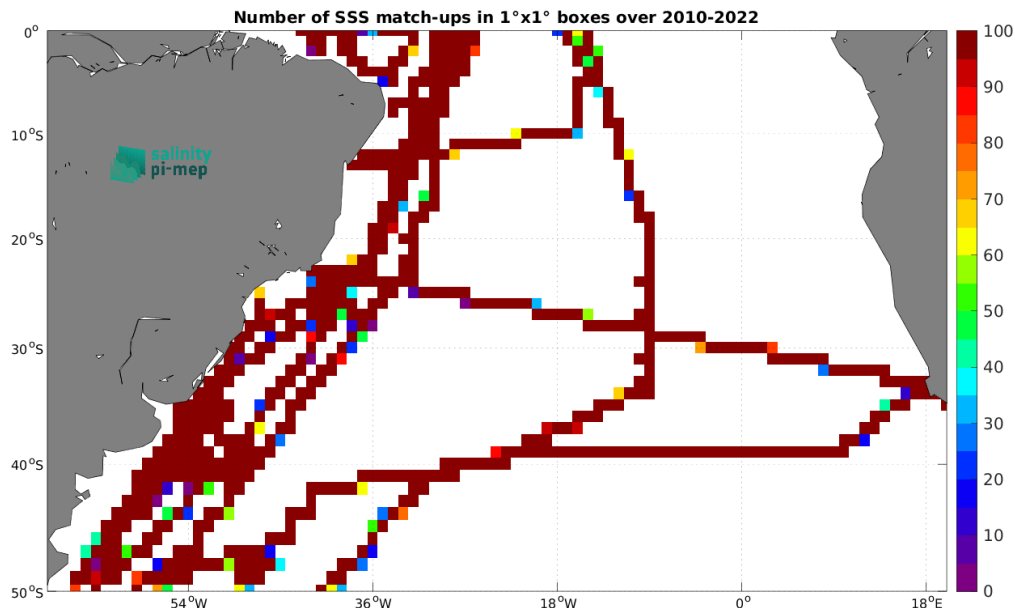
Figure 5: Number of SSS match-ups between TSG (CSIC-UTM) SSS and the SMOS SSS L3 v9 - 9 Days (CATDS-CEC-LOCEAN) SSS product for the South Atlantic Ocean Pi-MEP region over 1^\circ \times 1^\circ boxes and for the full satellite product period.
