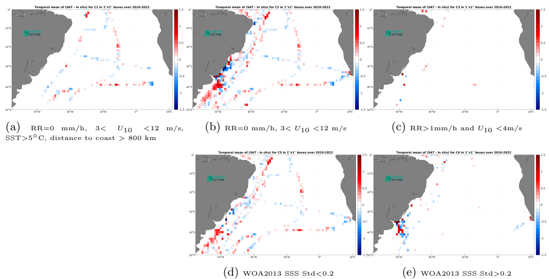
Figure 14: Temporal mean gridded over spatial boxes of size 1^\circ \times 1^\circ of \Delta SSS (SMOS SSS L3 v9 - 9 Days (CATDS-CEC-LOCEAN) - TSG (CSIC-UTM)) for 5 different subdatasets corresponding to:RR=0 mm/h, 3 < U_{10} < 12 m/s, SST>5°C, distance to coast > 800 km (a), RR=0 mm/h, 3 < U_{10} < 12 m/s (b), RR>1mm/h and U_{10} < 4 m/s (c), WOA2013 SSS Std<0.2 (d), WOA2013 SSS Std>0.2 (e).
