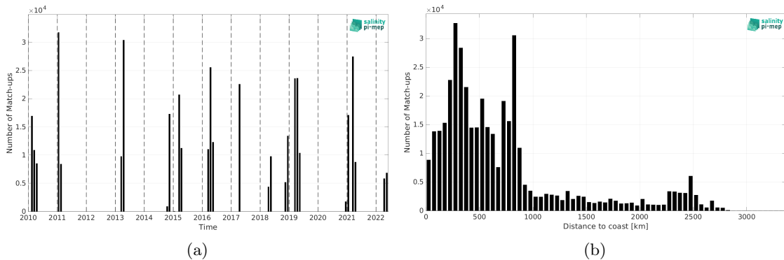
Figure 2: Number of match-ups between TSG (CSIC-UTM) and SMOS SSS L3 v9 - 9 Days (CATDS-CEC-LOCEAN) SSS as a function of time (a) and as function of the distance to coast (b) over the South Atlantic Ocean Pi-MEP region and for the full satellite product period.
