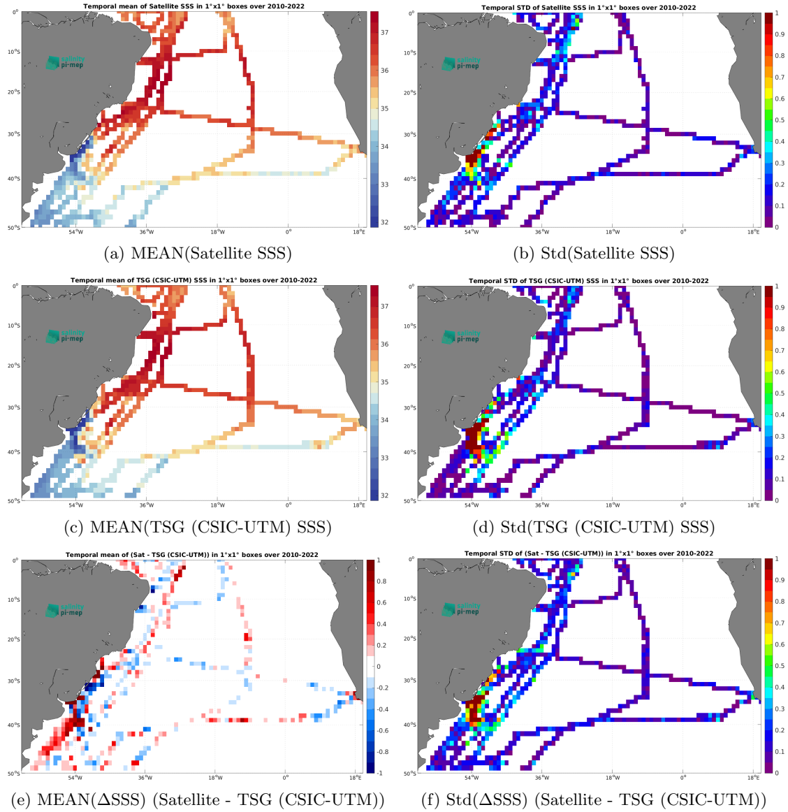
Figure 7: Temporal mean (left) and Std (right) of SSS from SMOS SSS L3 v9 - 9 Days (CATDS-CEC-LOCEAN) (top), TSG (CSIC-UTM) (middle), and of \Delta SSS (Satellite - TSG (CSIC-UTM)). Only match-up pairs are used to generate these maps.
