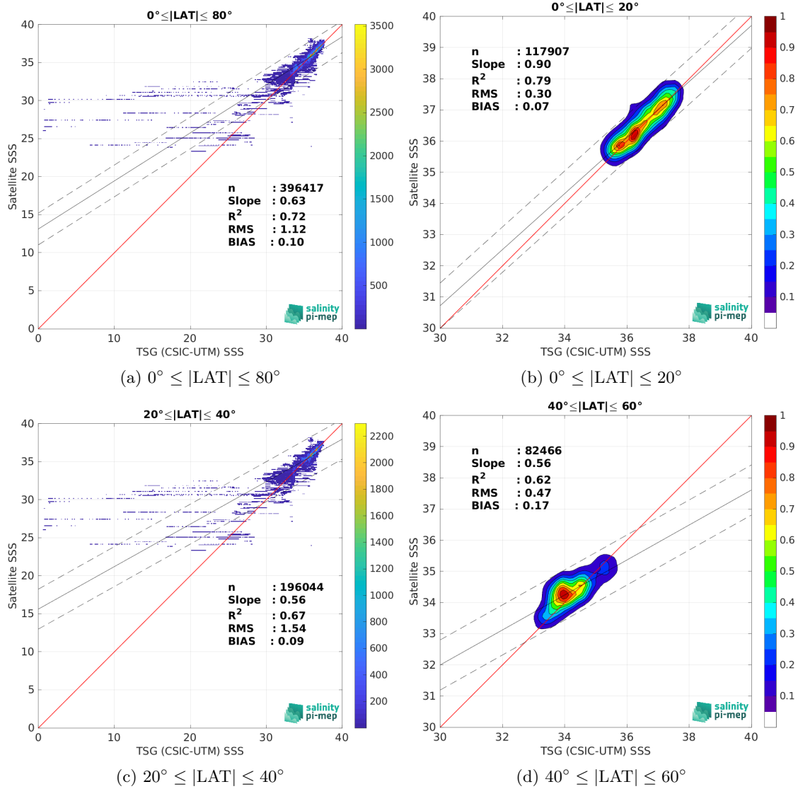
Figure 10: Contour maps of the concentration of SMOS SSS L3 v9 - 9 Days (CATDS-CEC-LOCEAN) SSS ( y -axis) versus TSG (CSIC-UTM) SSS ( x -axis) at match-up pairs for different latitude bands. For each plot, the red line shows x=y . The black thin and dashed lines indicate a linear fit through the data cloud and the \pm 95\% confidence levels, respectively. The number match-up pairs n , the slope and R^2 coefficient of the linear fit, the root mean square (RMS) and the mean bias between satellite and in situ data are indicated for each latitude band in each plots.
