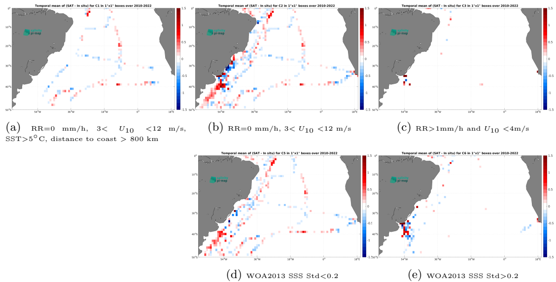
Figure 12: Temporal mean gridded over spatial boxes of size 1^\circ \times 1^\circ of \Delta\text{SSS} (SMOS SSS L3 v9 - 9 Days (CATDS-CEC-LOCEAN) - TSG (CSIC-UTM)) for 5 different subdatasets corresponding to:RR=0 mm/h, 3 < U_{10} < 12 m/s, SST >5^\circ\text{C} , distance to coast > 800 km (a), RR=0 mm/h, 3 < U_{10} < 12 m/s (b), RR >1 mm/h and U_{10} < 4 m/s (c), WOA2013 SSS Std <0.2 (d), WOA2013 SSS Std >0.2 (e).
