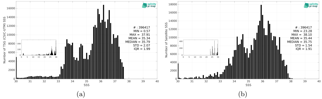
Figure 2: Histograms of SSS from TSG (CSIC-UTM) (a) and SMOS SSS L3 v9 - 9 Days (CATDS-CEC-LOCEAN) (b) considering all match-up pairs per bins of 0.1 over the South Atlantic Ocean Pi-MEP region and for the full satellite product period.
