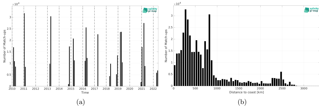
Figure 1: Number of match-ups between TSG (CSIC-UTM) and SMOS SSS L3 v9 - 9 Days (CATDS-CEC-LOCEAN) SSS as a function of time (a) and as function of the distance to coast (b) over the South Atlantic Ocean Pi-MEP region and for the full satellite product period.
