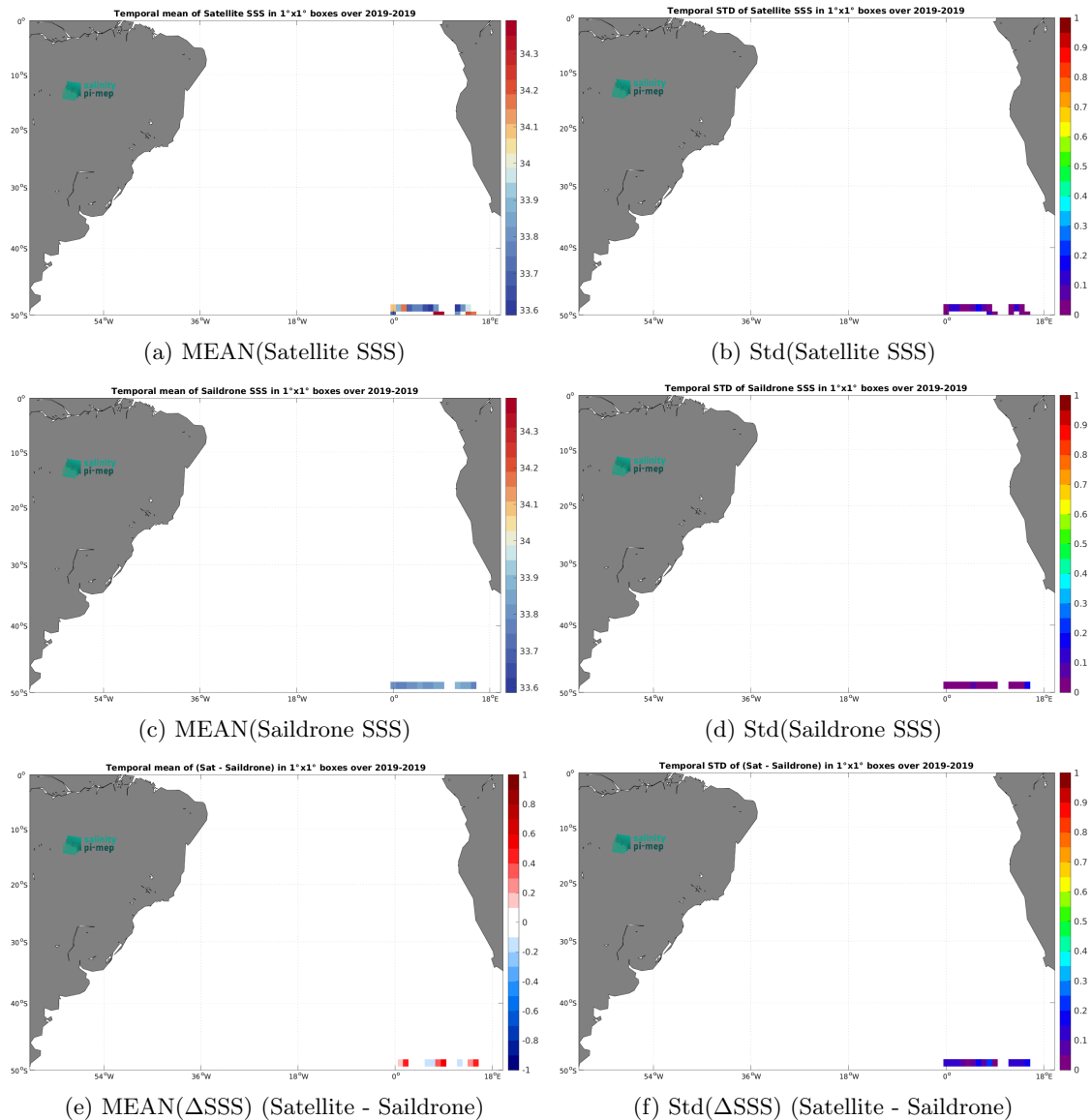
Figure 6: Temporal mean (left) and Std (right) of SSS from SMOS SSS L3 v9 - 9 Days (CATDS-CEC-LOCEAN) (top), Saildrone (middle), and of \Delta SSS (Satellite - Saildrone). Only match-up pairs are used to generate these maps.
