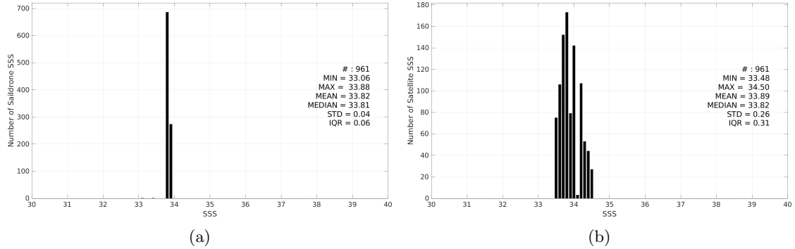
Figure 2: Histograms of SSS from Saildrone (a) and SMOS SSS L3 v9 - 9 Days (CATDS-CEC-LOCEAN) (b) considering all match-up pairs per bins of 0.1 over the South Atlantic Ocean Pi-MEP region and for the full satellite product period.
