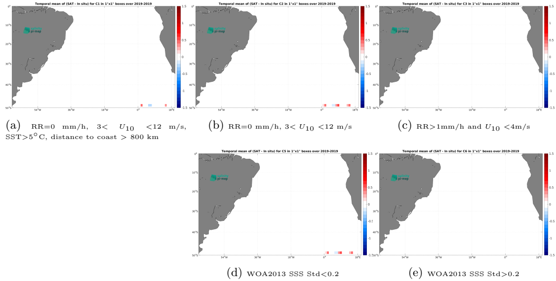
Figure 12: Temporal mean gridded over spatial boxes of size 1^{\circ}\times 1^{\circ} of \Delta\text{SSS} (SMOS SSS L3 v9 - 9 Days (CATDS-CEC-LOCEAN) - Saifdrone) for 5 different subdatasets corresponding to:RR=0 mm/h, 3 < U_{10} < 12 m/s, SST >5^{\circ}\text{C} , distance to coast > 800 km (a), RR=0 mm/h, 3 < U_{10} < 12 m/s (b), RR >1 mm/h and U_{10} < 4 m/s (c), WOA2013 SSS Std <0.2 (d), WOA2013 SSS Std >0.2 (e).
