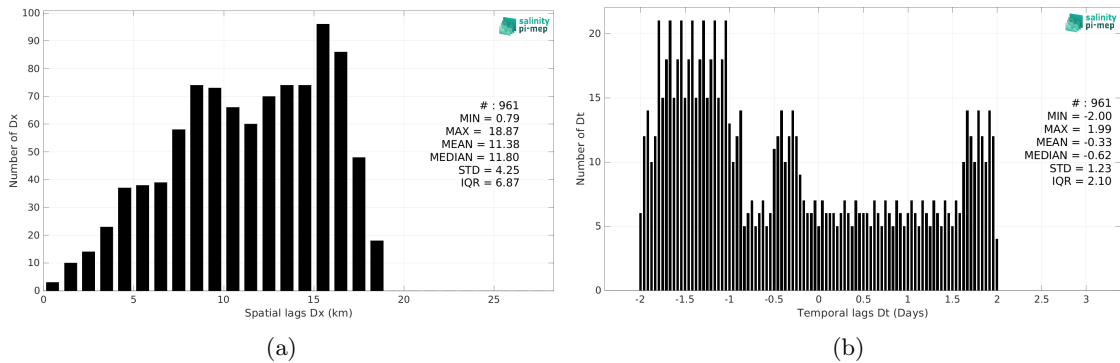
Figure 5: Histograms of the spatial (a) and temporal (b) lags between the location/time of the Sairdrone measurement and the date of the corresponding SMOS SSS L3 v9 - 9 Days (CATDS-CEC-LOCEAN) SSS pixel.
