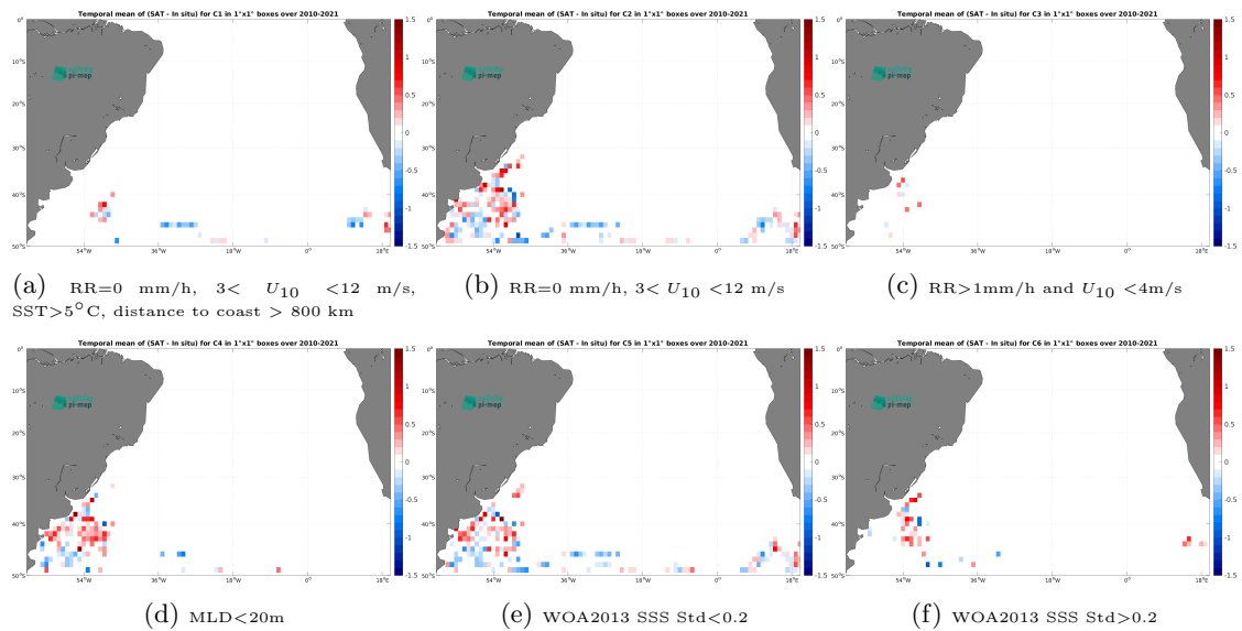
Figure 14: Temporal mean gridded over spatial boxes of size 1^\circ \times 1^\circ of \Delta SSS (SMOS SSS L3 v9 - 9 Days (CATDS-CEC-LOCEAN) - Marine mammals) for 6 different subdatasets corresponding to:RR=0 mm/h, 3 < U_{10} < 12 m/s, SST>5°C, distance to coast > 800 km (a), RR=0 mm/h, 3 < U_{10} < 12 m/s (b), RR>1mm/h and U_{10} < 4 m/s (c),MLD<20m (d),WOA2013 SSS Std<0.2 (e),WOA2013 SSS Std>0.2 (f).
