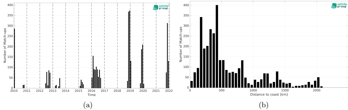
Figure 2: Number of match-ups between Marine mammals and SMOS SSS L3 v9 - 9 Days (CATDS-CEC-LOCEAN) SSS as a function of time (a) and as function of the distance to coast (b) over the South Atlantic Ocean Pi-MEP region and for the full satellite product period.
