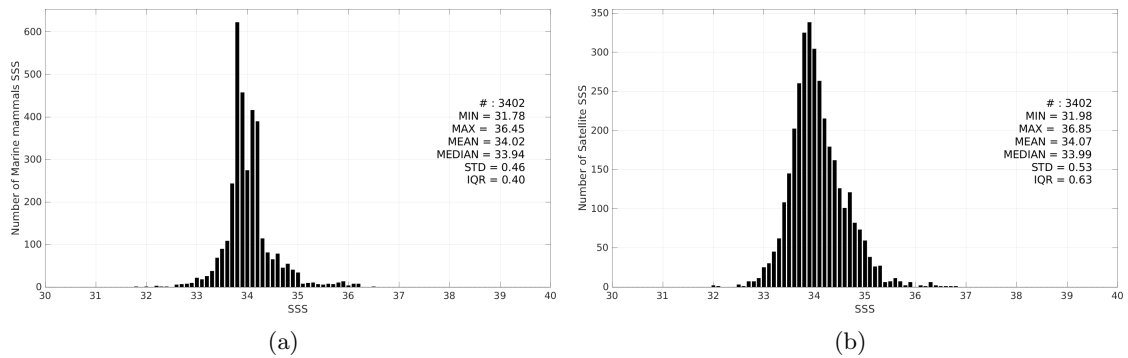
Figure 3: Histograms of SSS from Marine mammals (a) and SMOS SSS L3 v9 - 9 Days (CATDS-CEC-LOCEAN) (b) considering all match-up pairs per bins of 0.1 over the South Atlantic Ocean Pi-MEP region and for the full satellite product period.
